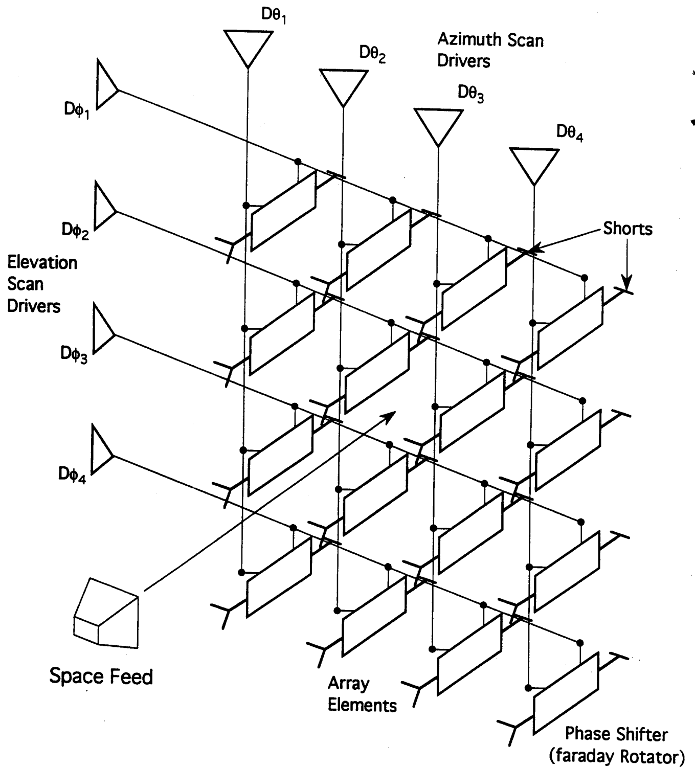
FIG. 13. REFLECTARRAY CONFIGURATION USING RUSSIAN APPROACH
