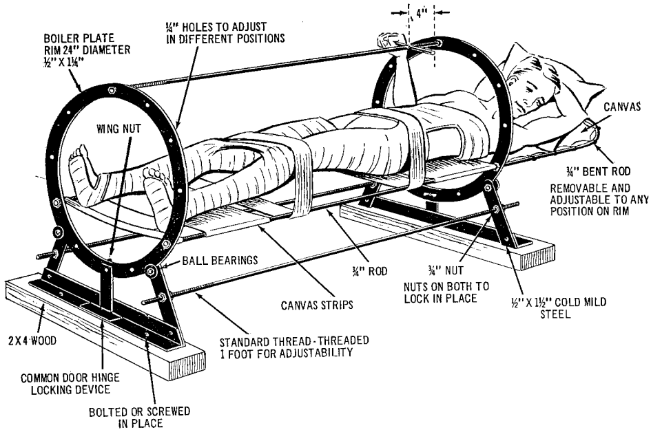
FIGURE 11.—Improved revolving Bradford frame.
