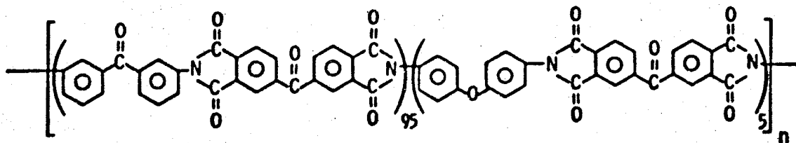
LARC-TPI/ODA
