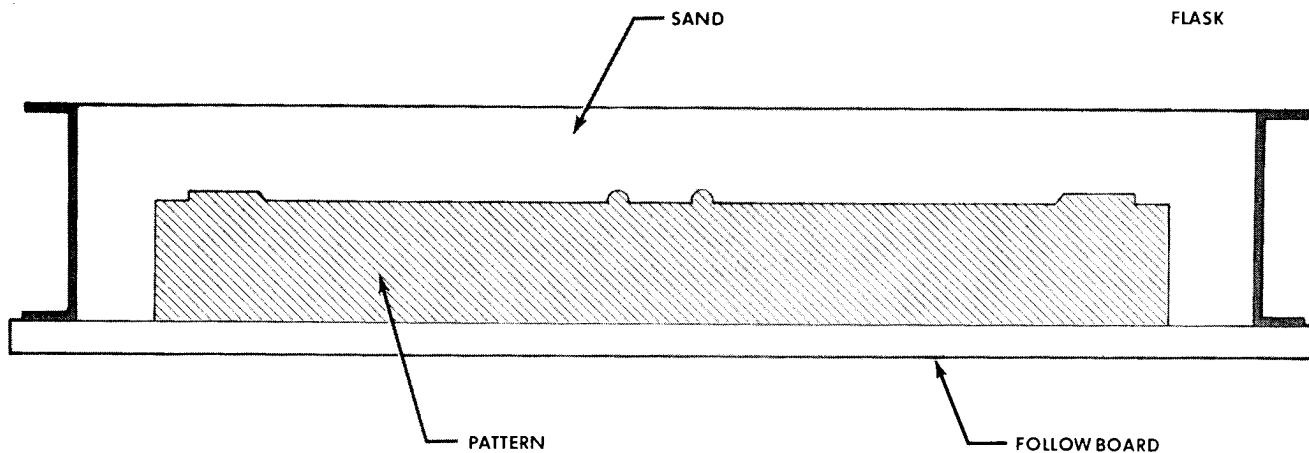
FIG.2 EXPANDED WOOD OR PLASTER PATTERN IN SAND
