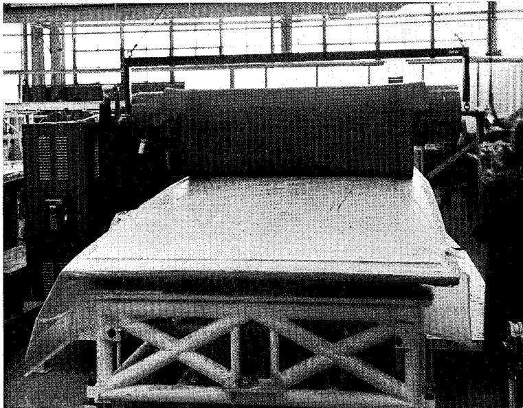
Fig. 4 Silicone Rubber Embedded blanket being placed in operation.
