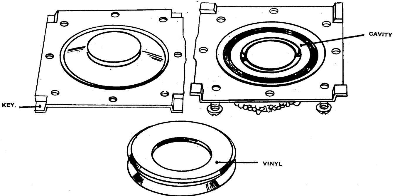
FIG. #7 ELECTROFORMED MOLD
