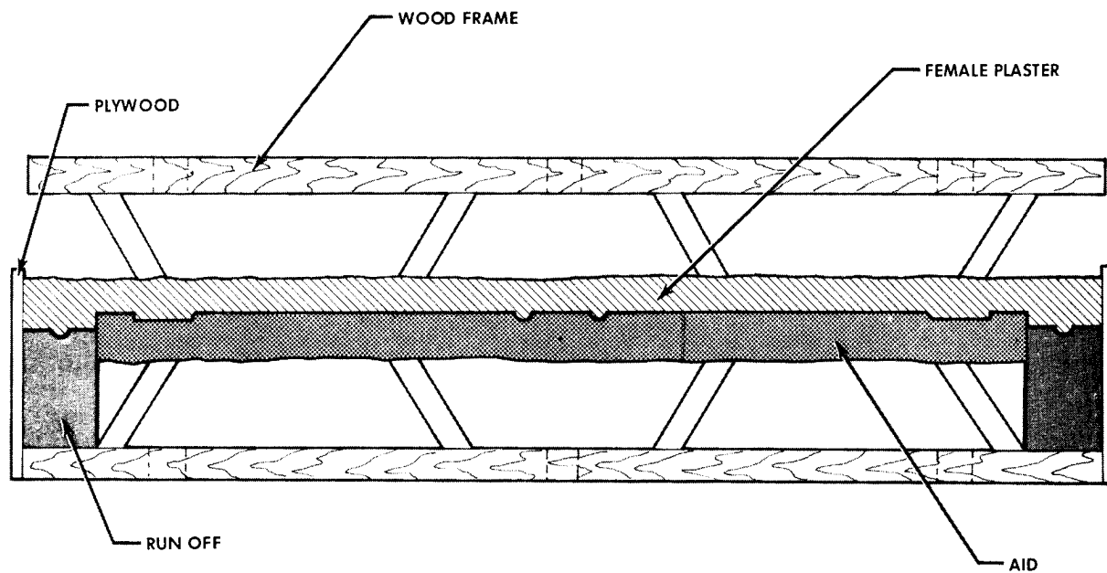
FIG. 8 ADD RUN OFF, RING SURFACE AND MAKE FEMALE PLASTER
