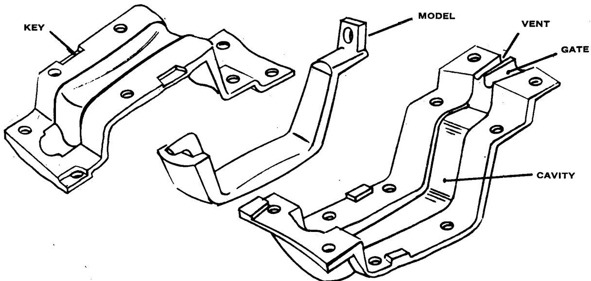
FIG. #8 CAST METAL MOLD
