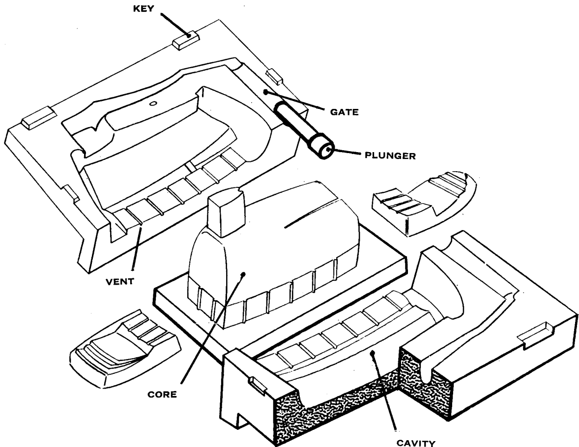
FIG. #6 REINFORCED PLASTIC MOLD
