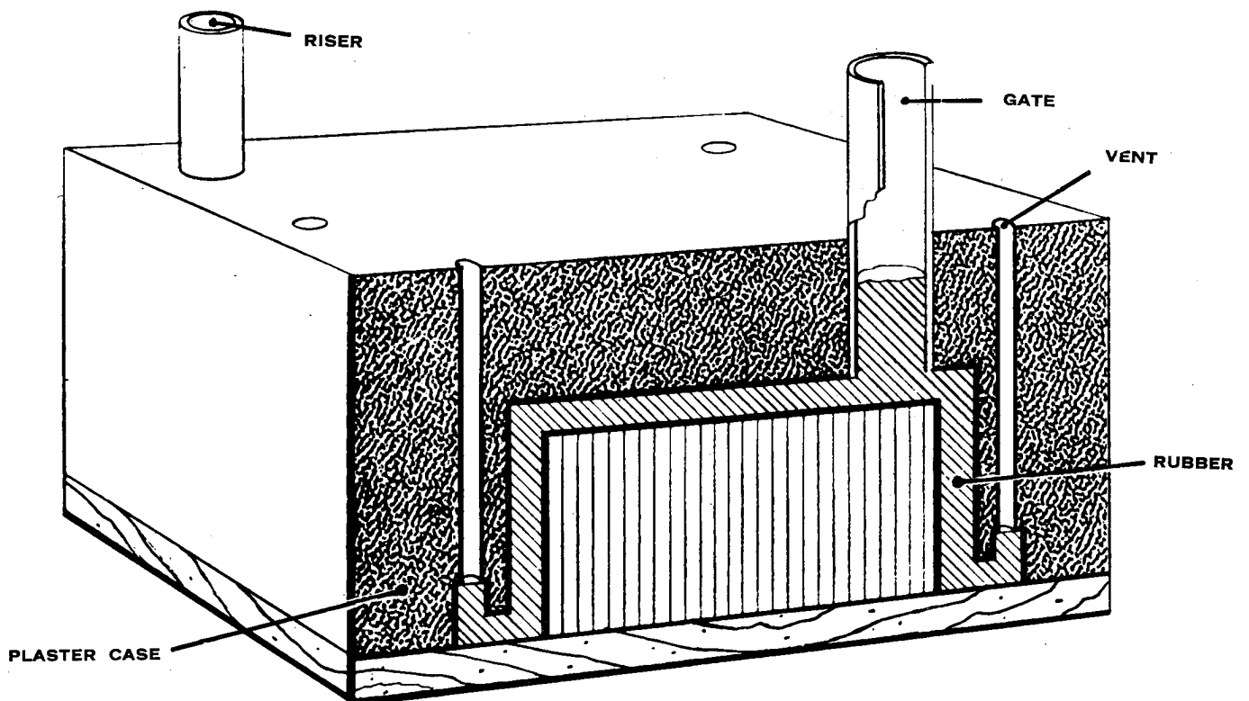
FIG. #9 POLYSULFIDE MOLD
