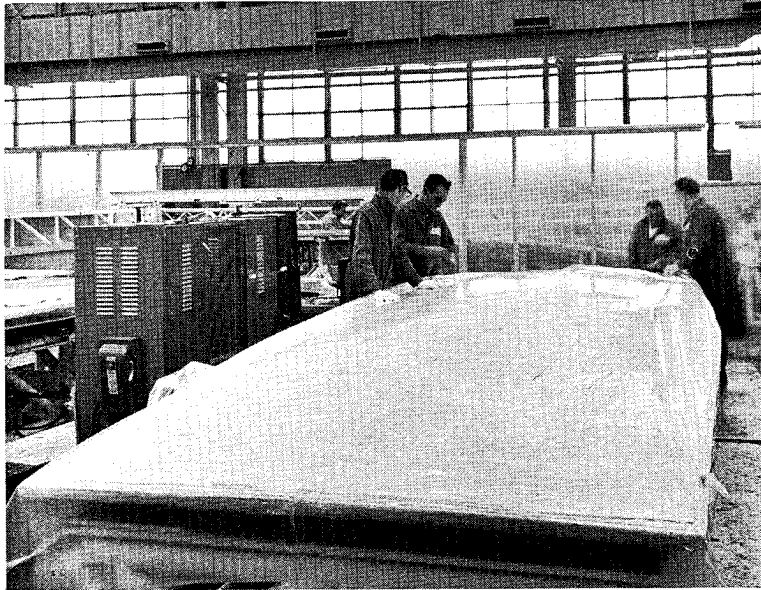
Fig. 3 PVA film being placed for vacuum bag operation.
