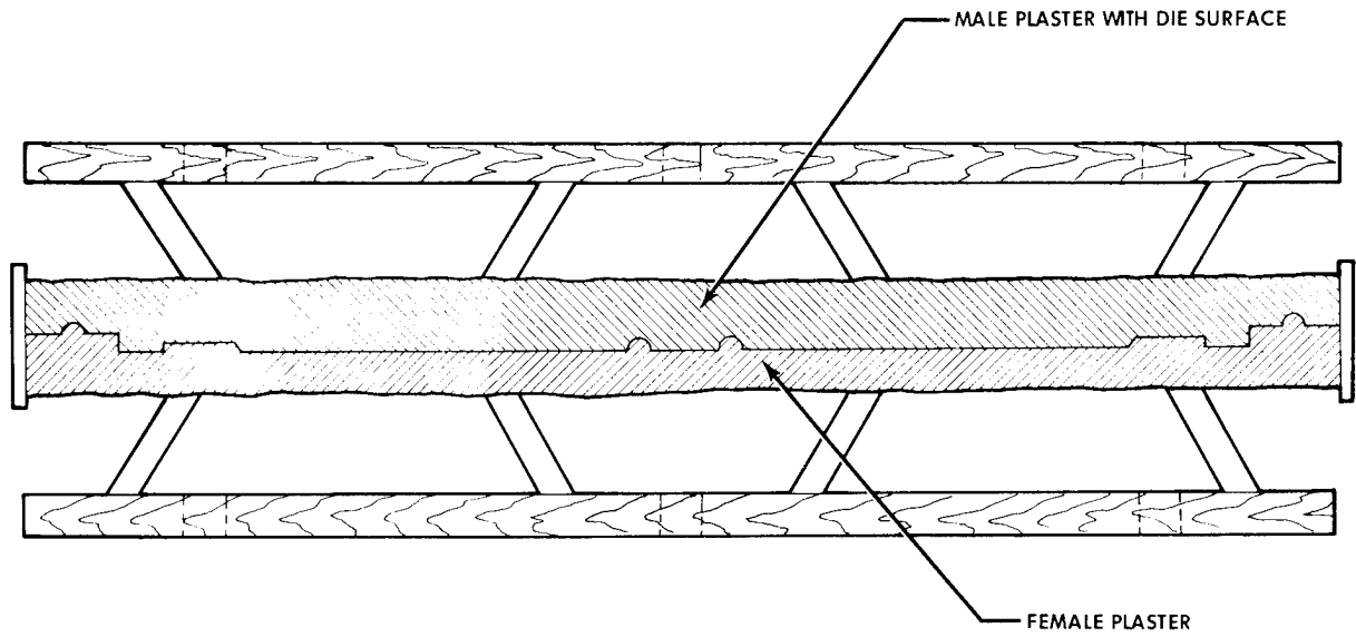
FIG. 9 MAKE MALE PLASTER TO USE FOR DIE
