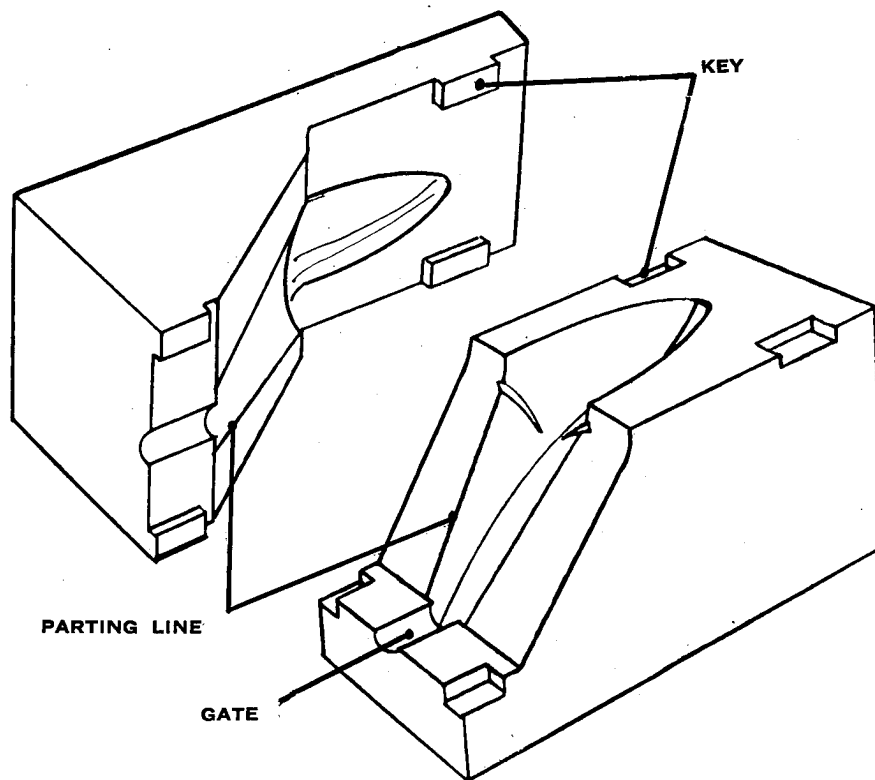
FIG. #3 PLASTER PIECE MOLD
