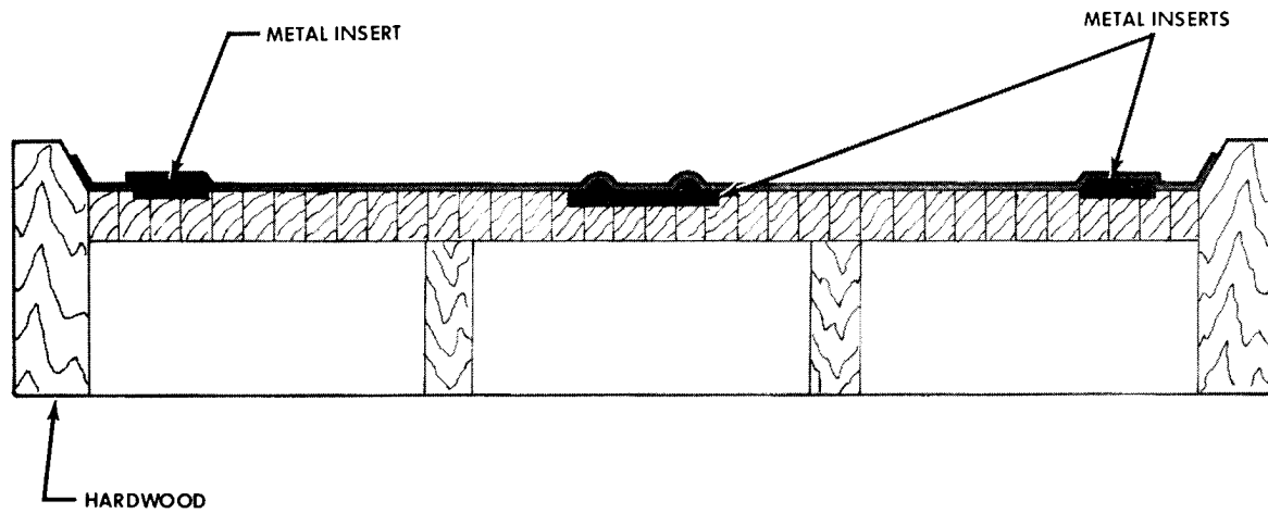
FIG.1 HARDWOOD HAMMER FORM
