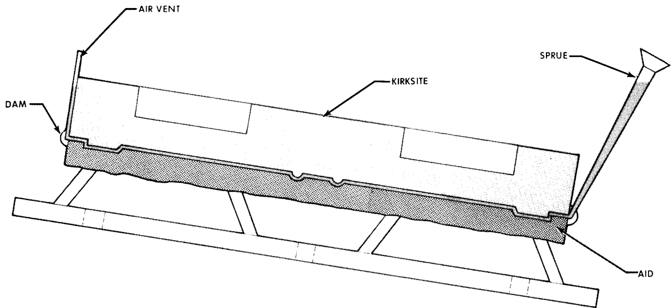
FIG. 5 PLASTIC FACE WITH KIRKSITE CORE
