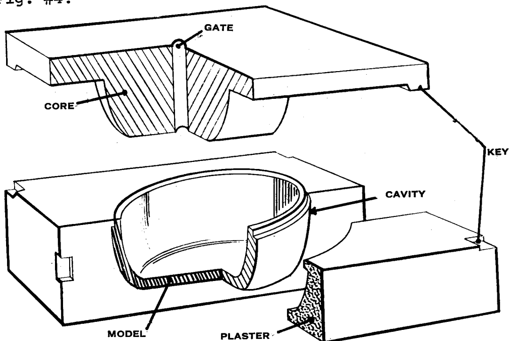
FIG. #4 PLASTER PIECE MOLD — CLOSED CORE
