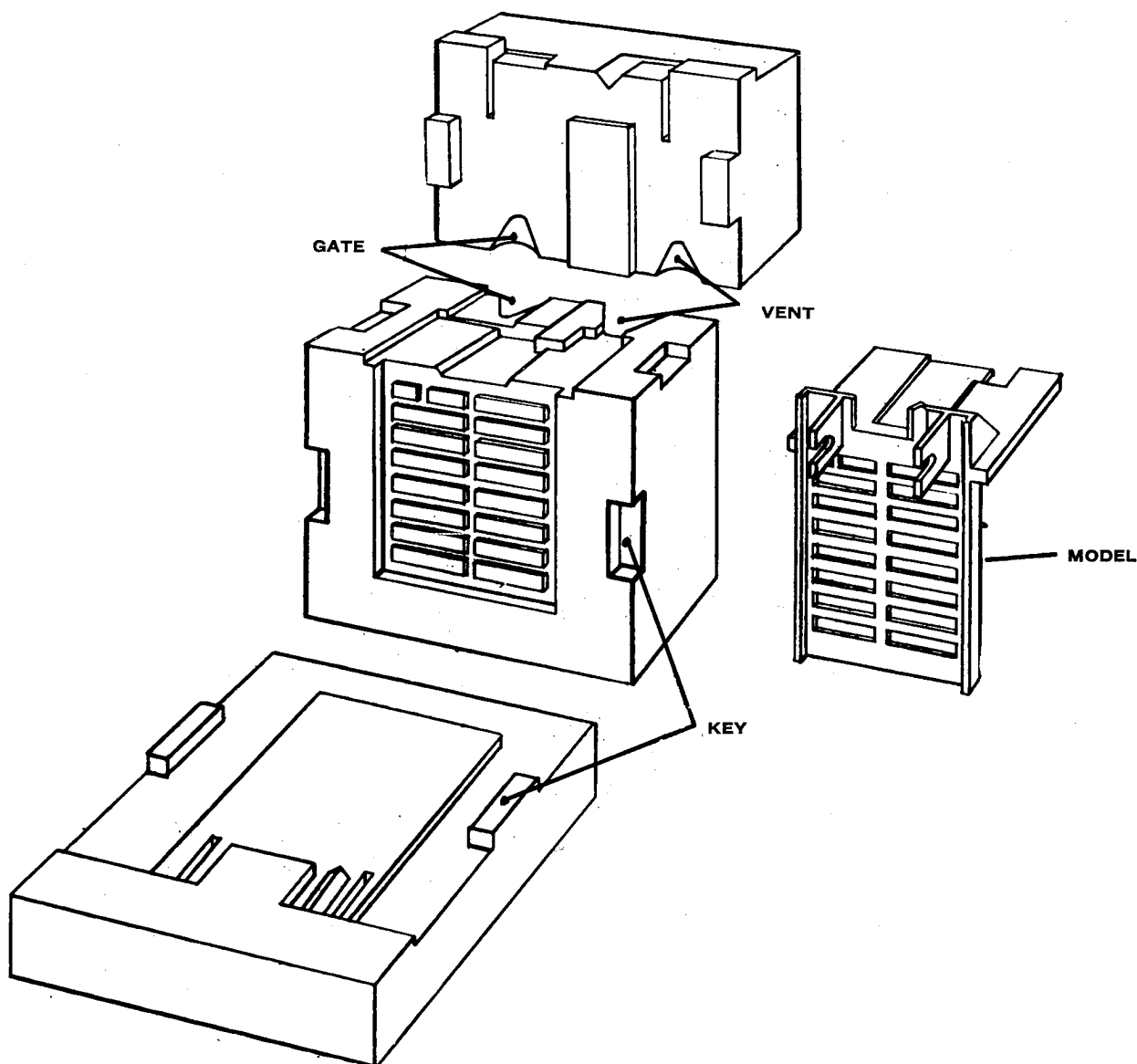
FIG. #10 RTV RUBBER MOLD
