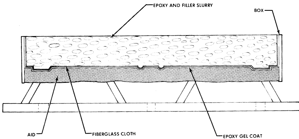
FIG. 6 EPOXY FACE WITH EPOXY RESIN AND FILLER SLURRY
