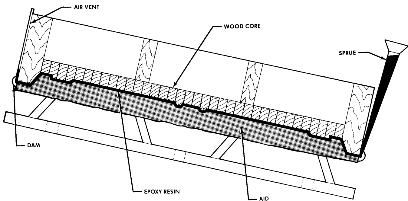
FIG. 4 PLASTIC FACE WITH WOOD CORE
