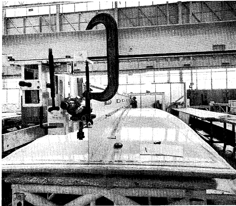
Fig. 1 Tool being checked for Surface Tolerance.
