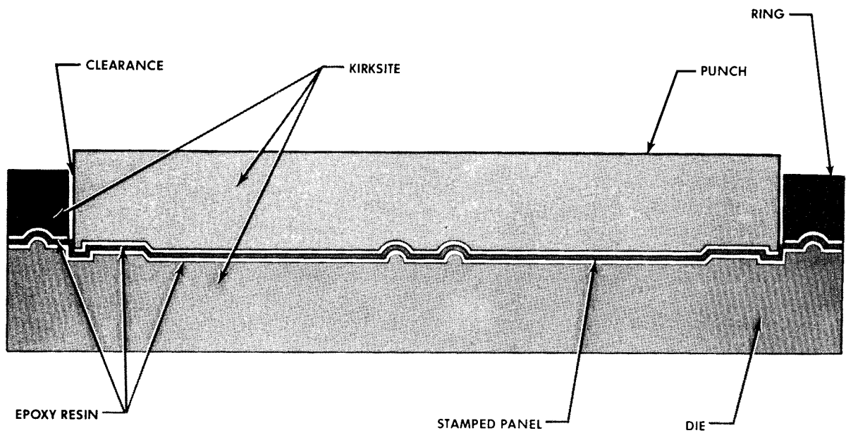
FIG.13 THREE PIECE PLASTIC FACED KIRKSITE DIE SET
