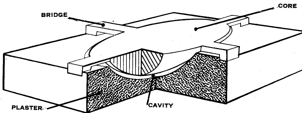
FIG. #2 PLASTER MOLD OPEN CORE
