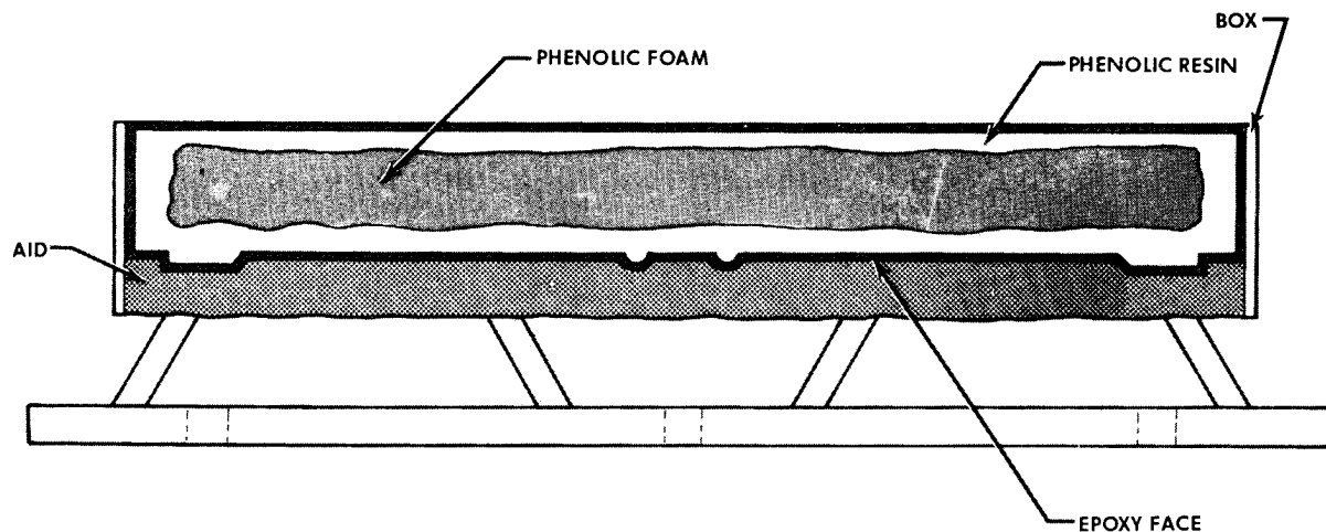
FIG.7 EPOXY FACE WITH PHENOLIC FOAM AND PHENOLIC RESIN CORE
