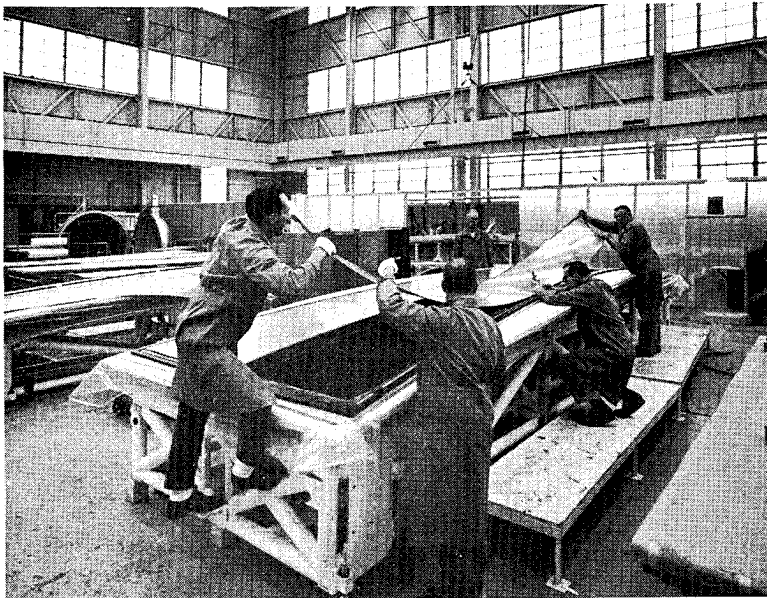
Fig. 2 Outer skin being applied to core.
