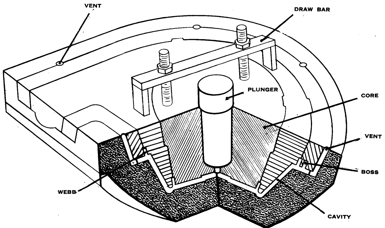
FIG. #5 REINFORCED PLASTIC MOLD
