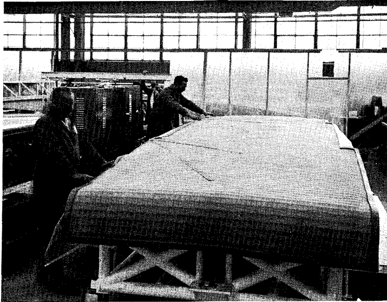
Fig. 5 Ready for the heating bonding operation.
