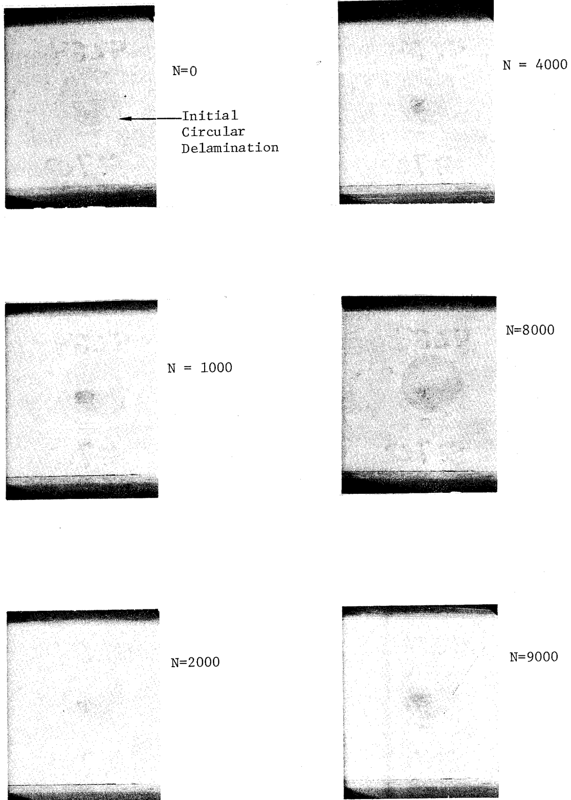
Figure 34. Delamination Growth in Specimen 4284-70; Laminate A; Test Series 14; S=0.83
