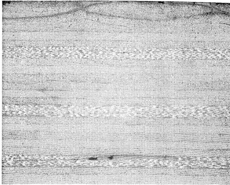
Figure 79 Selected Hybrid System #5a (25X)
