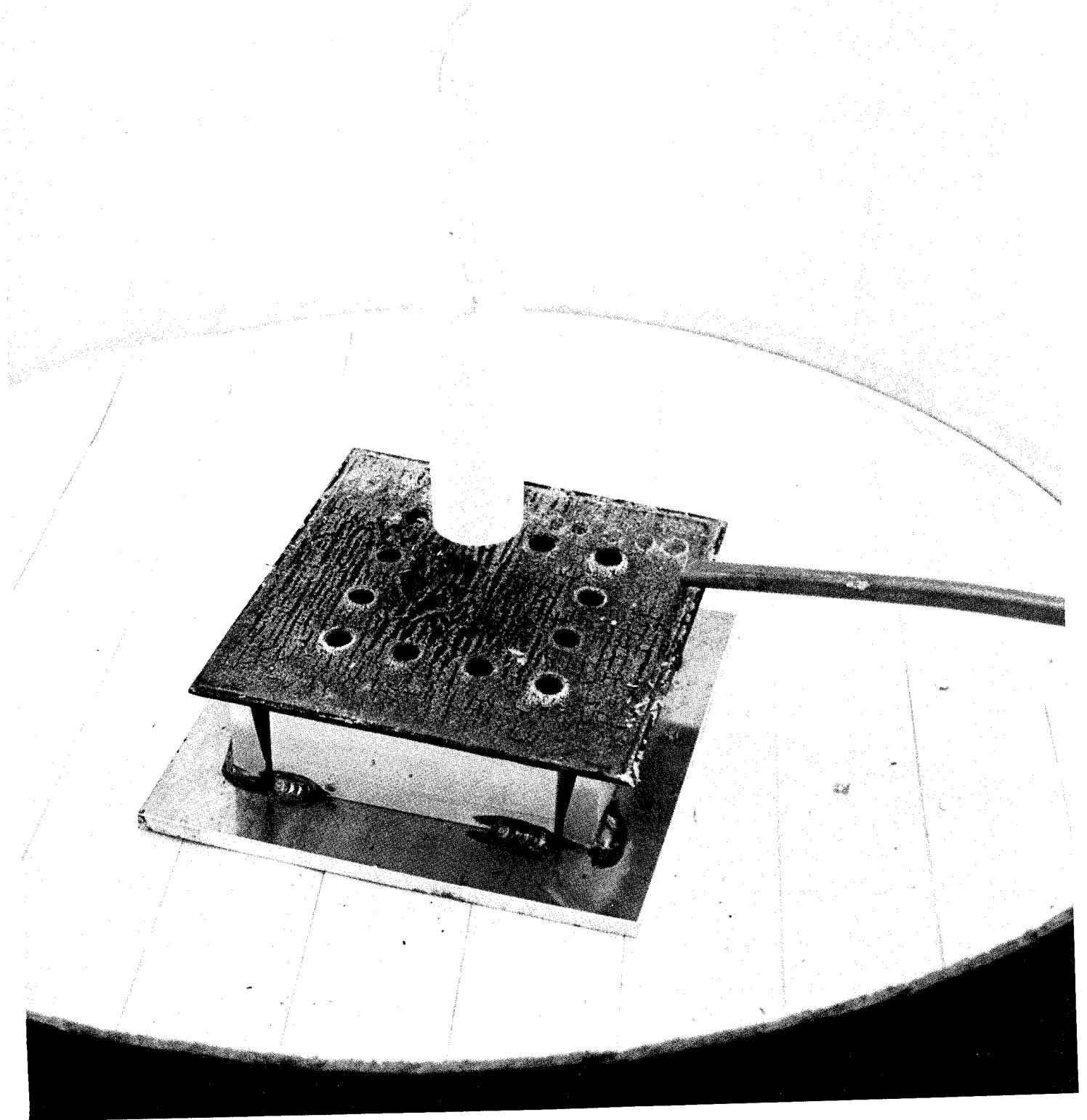
Figure 52 Specimen Positioned in Impact and Air Flow Test Chamber
