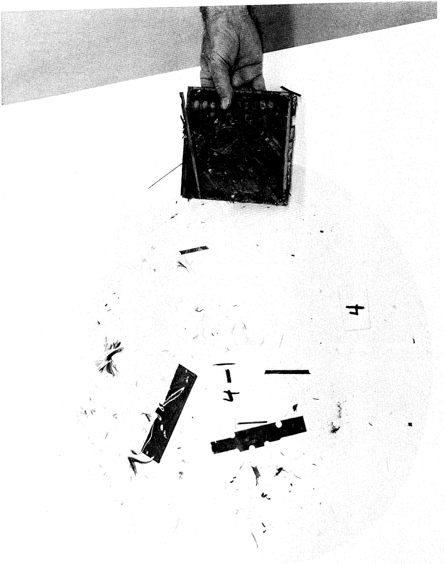
Baseline System #4 After Burn, Impact, and Air Flow Test
