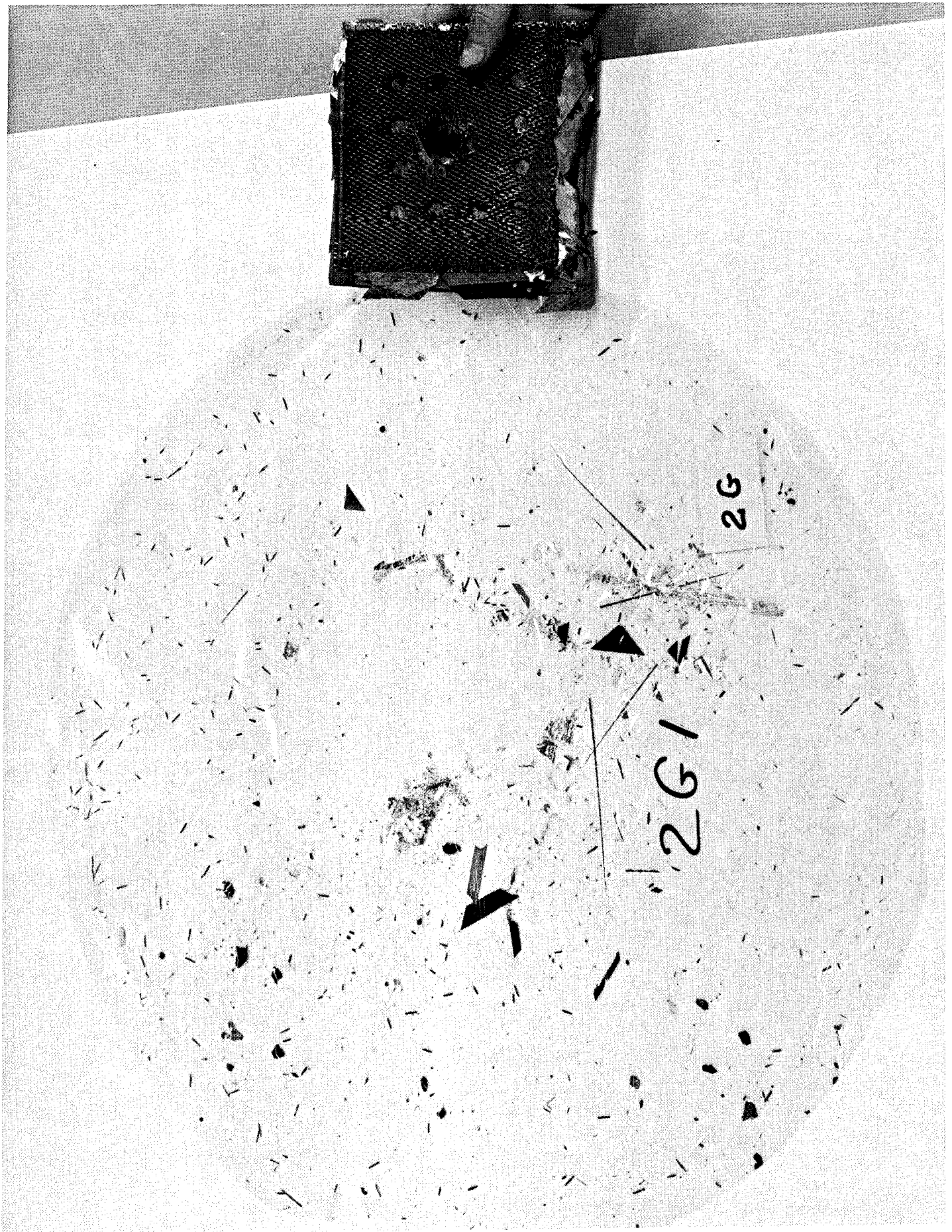
Figure 66 Hybrid System #2g After Burn, Impact, and Air Flow Test
