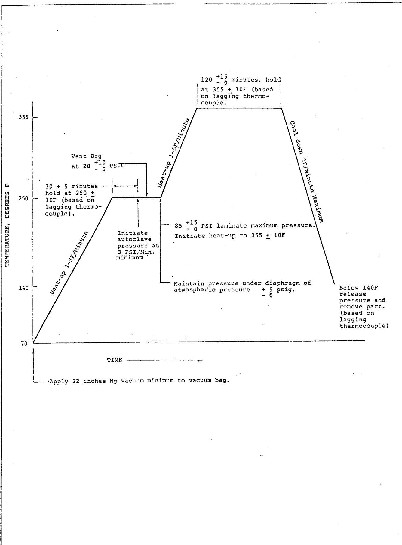
Figure 25. Autoclave Cure Cycle for Epoxy Matrix Composites
