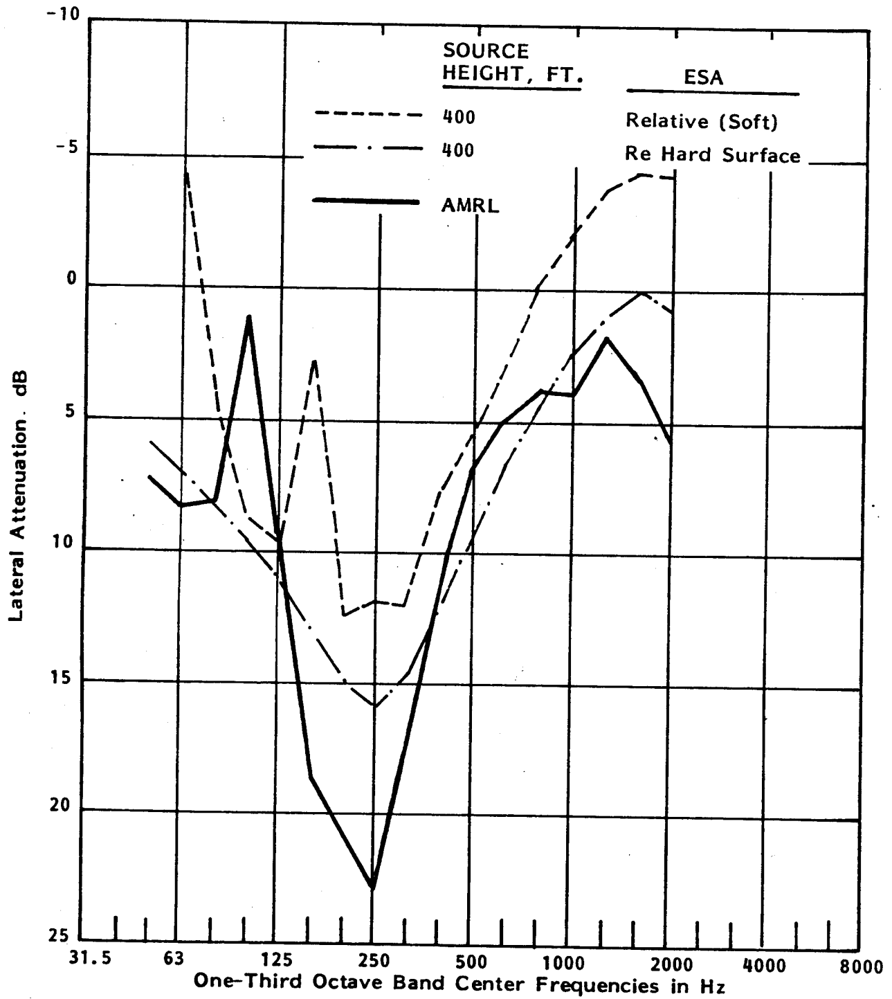
FIGURE 2. COMPARISON OF LATERAL ATTENUATION, 2° ELEVATION ANGLE
