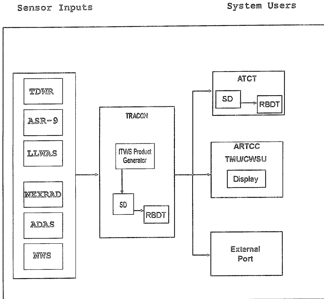
FIGURE 5.5.1.1.2-1. SIMPLE SITE OT&E INTEGRATION PHASE II CONFIGURATION
