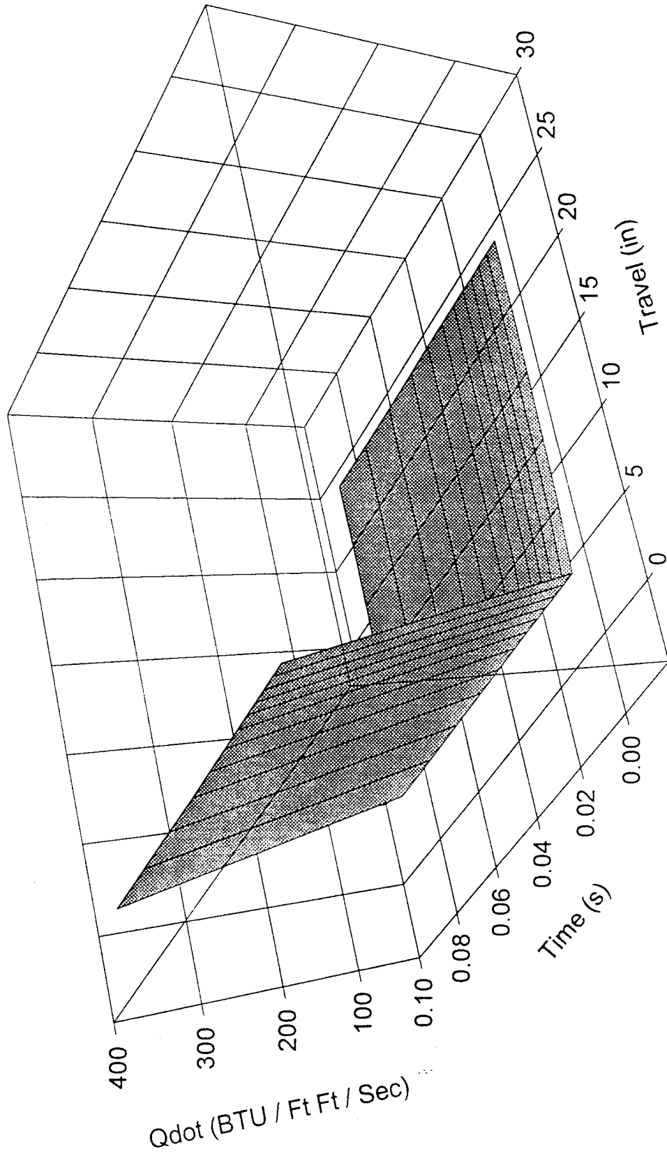
Figure 9 - TDK/MABL 155mm M203 Cold Wall Qdot Data
