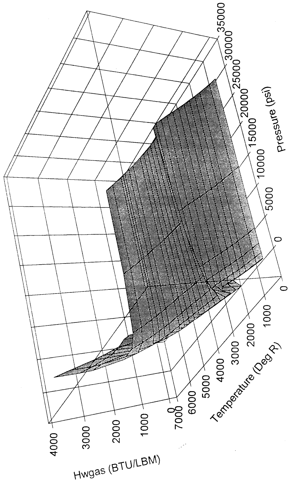
Figure 11 - TDK/ODE 155mm M203 Hwgas Reacting Chromium Wall Data
