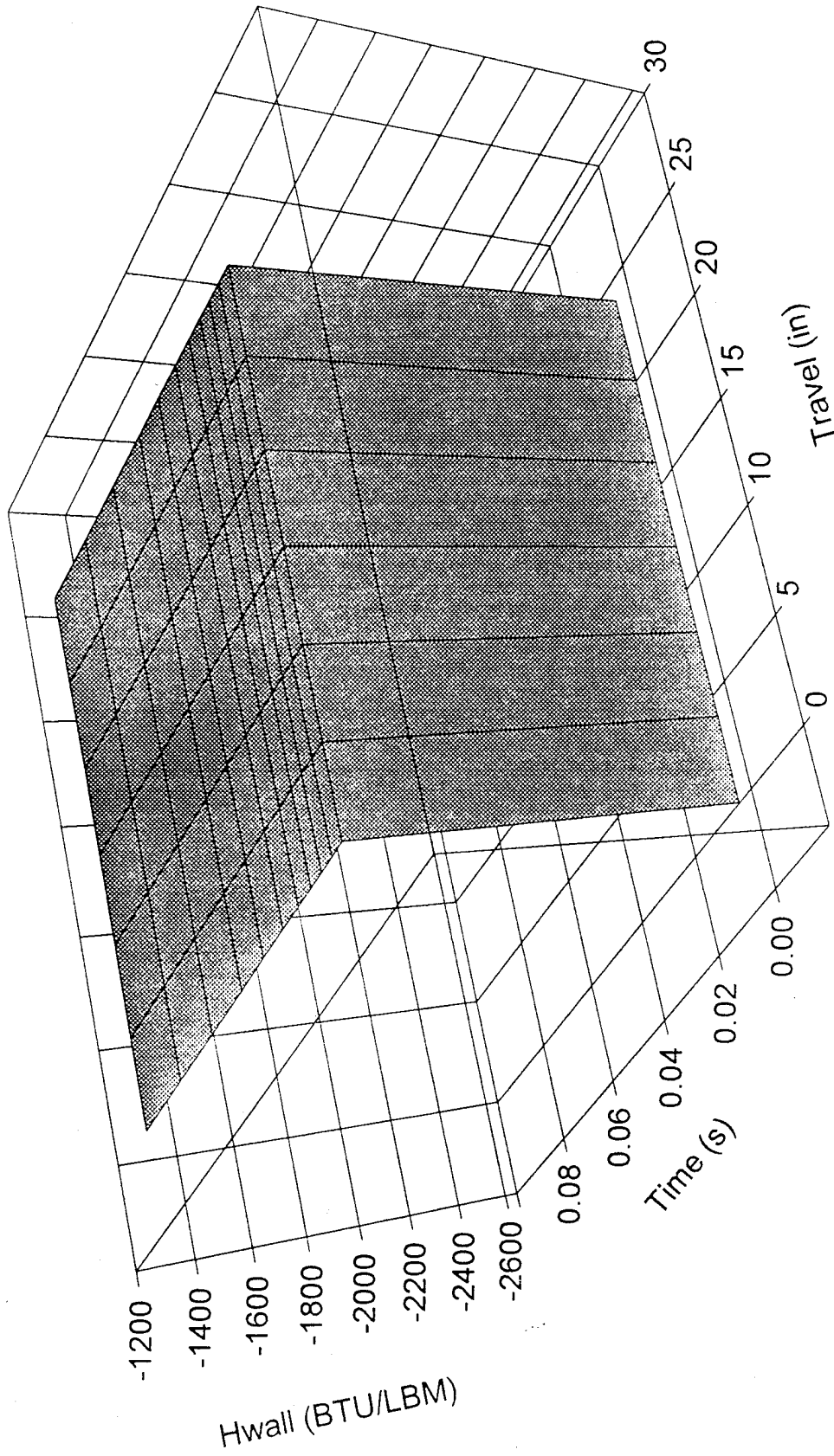
Figure 7 - TDK/MABL 155mm M203 Adiabatic Hwall Data
