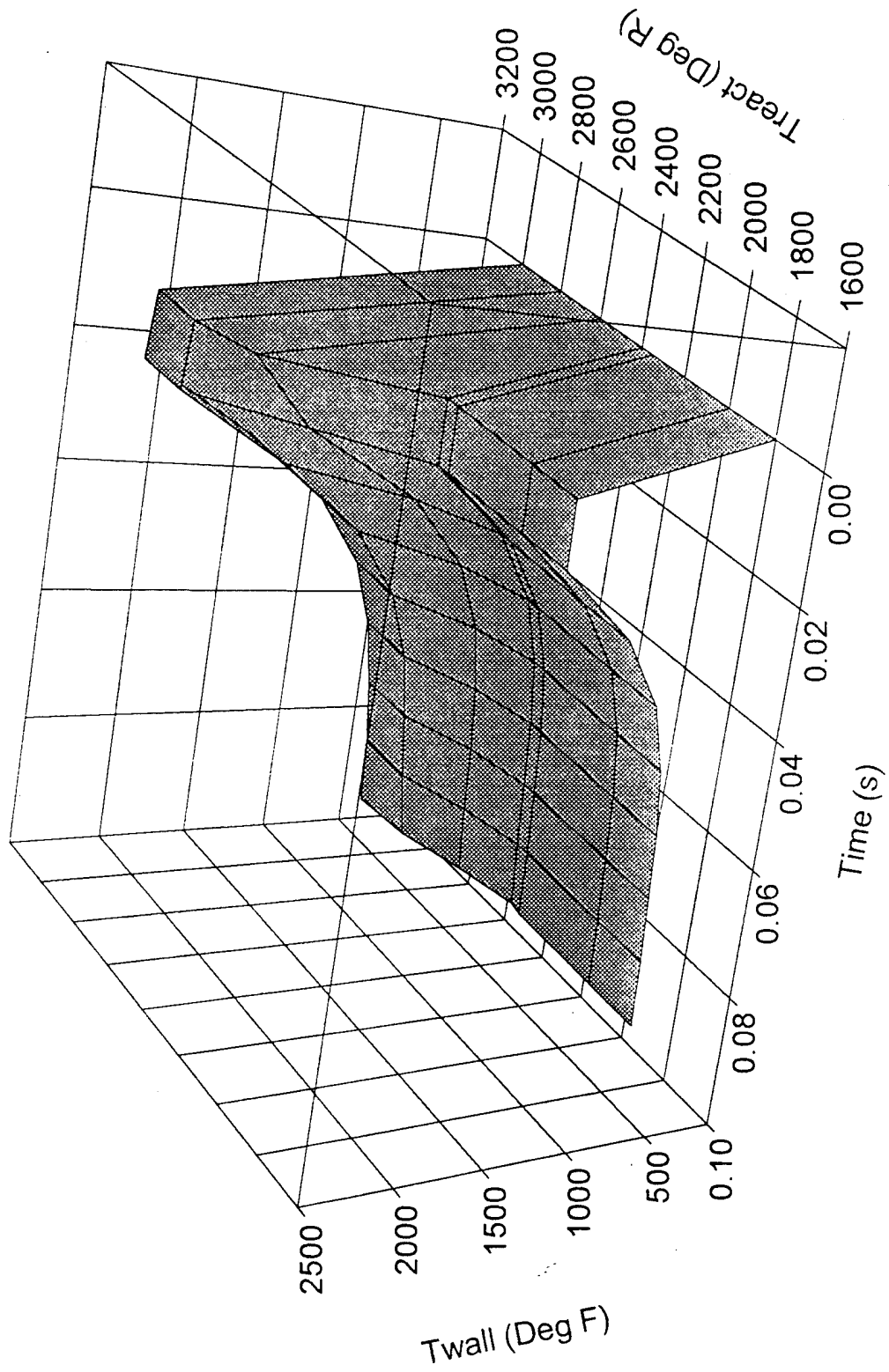
Figure 22 - MACE 155mm M203 Chromium Station One Twall Data
