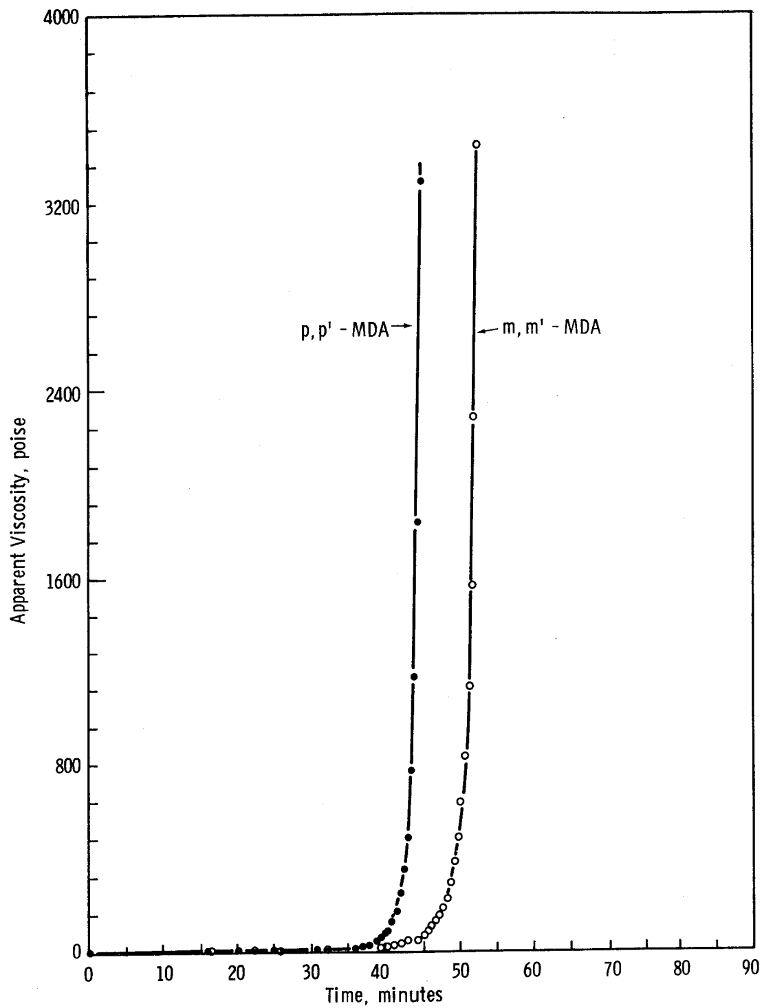
Figure 5. Apparent Viscosity vs Time at 100°C for Diamine/Epoxy Mixtures
