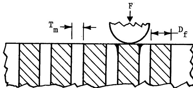
Figure III-5 Schematics of single fiber methods of measuring interfacial shear strengths.
