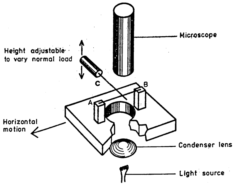
Figure III-2 Schematic of single filament friction test (36)
