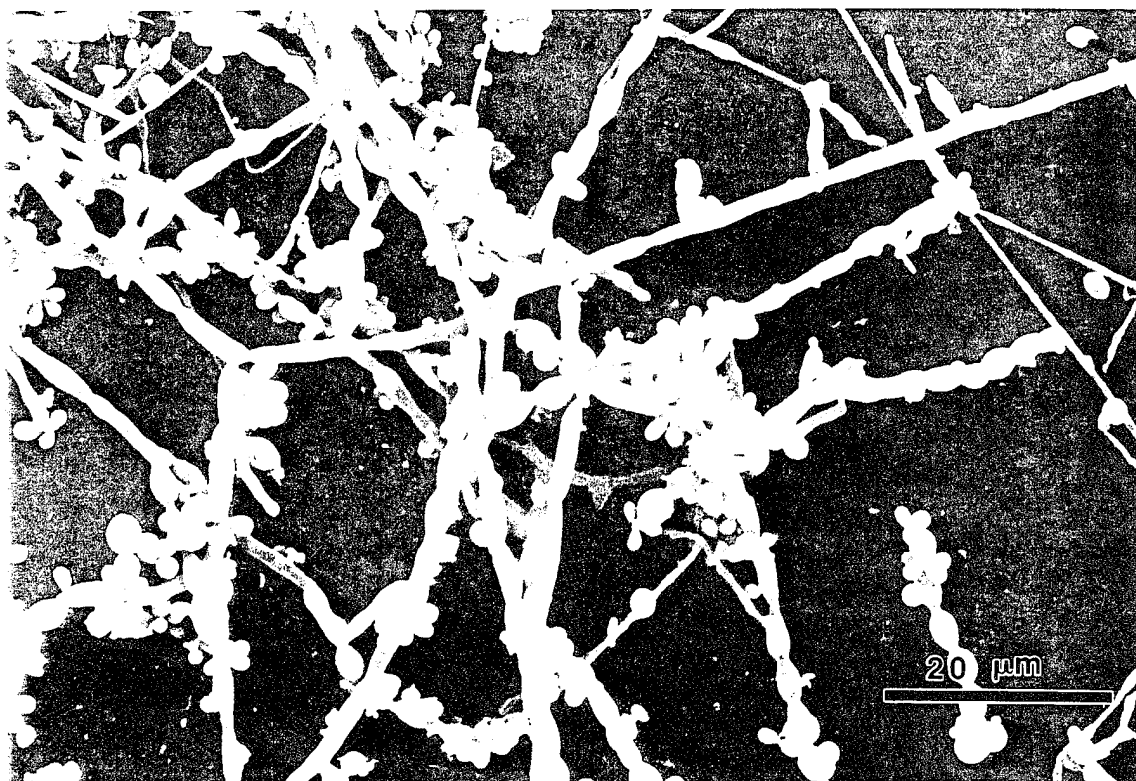
Fig. 3.7 SEM micrographs of biodeteriorated polyimides from the inoculated EIS cell showing fungi on the polyimide film
