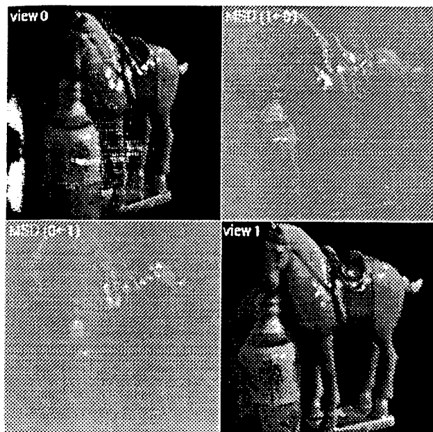
Figure 1: Spectral differencing
