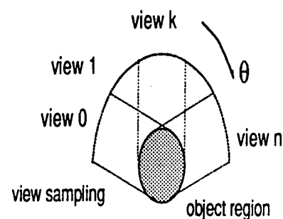
Figure 3: View sampling
