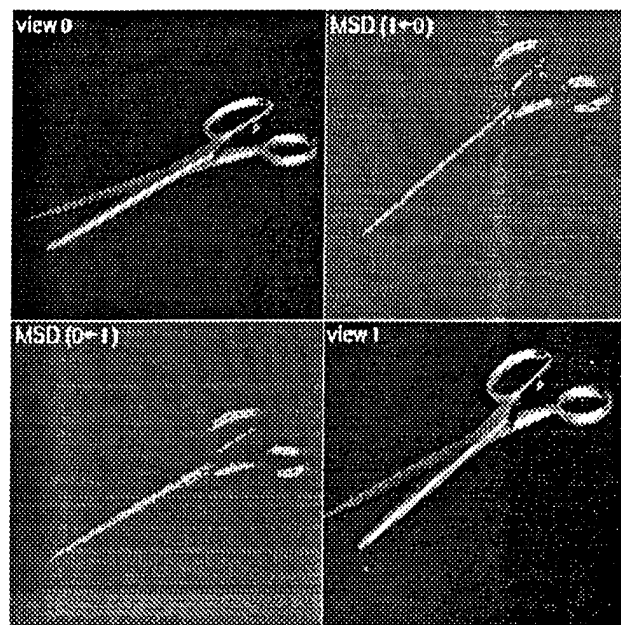
Figure 2: Spectral differencing
