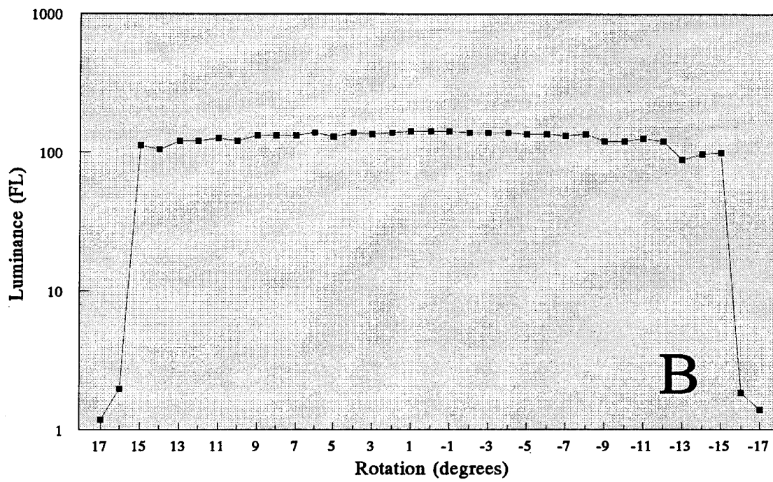
Figure 9. Luminance measurements showing the horizontal and vertical fields-of-view. A - horizontal FOV, B - Vertical FOV.
