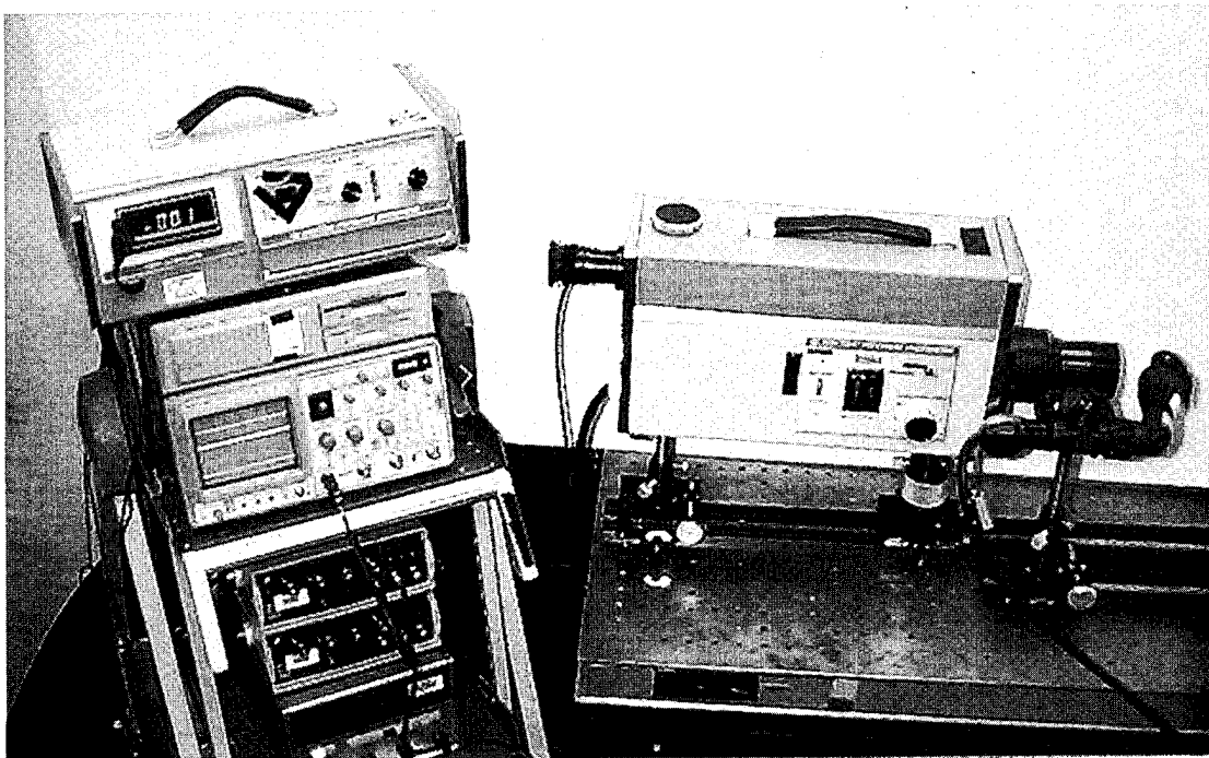
Figure 20. Photograph of test setup for measuring the spatiotemporal MTF.
