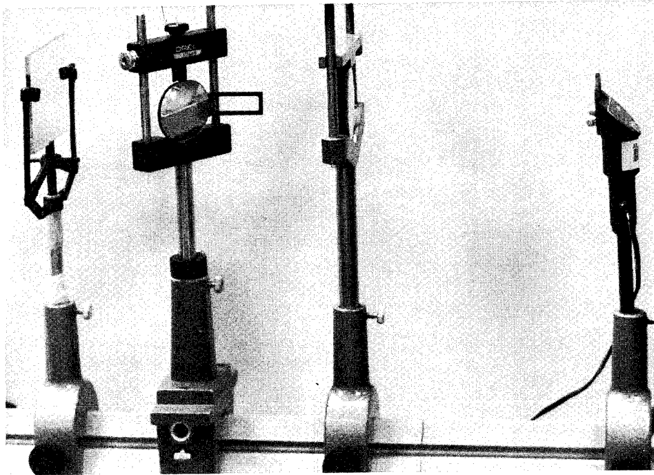
Figure 14. Photograph of test setup for measuring optical distortion.
