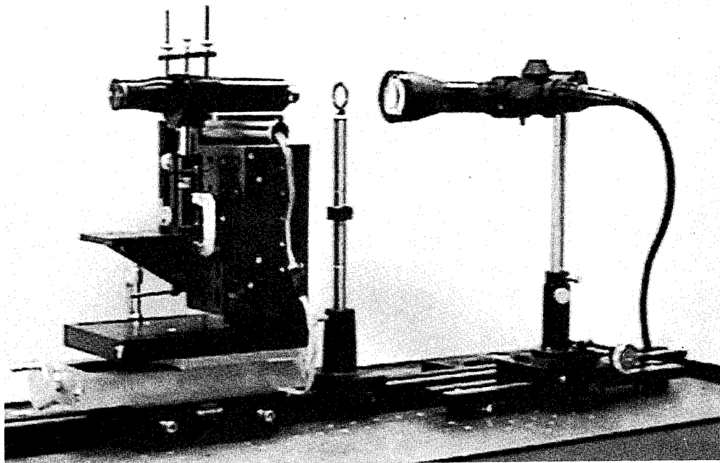
Figure 5. HDU (without the combiner lens in place) test setup for measurement of exit pupil size, position, and eye relief.
