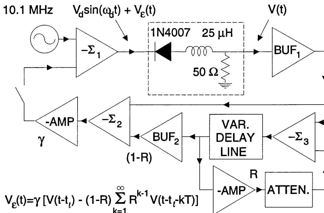
Figure 3.3: Analog implementation ETDAS used to control a diode resonator. Components: high-impedance buffers (BUF), inverting op amp (-AMP), inverting, summing op amp (-Σ), attenuator (ATTEN.), and low-loss variable delay line. The time lag t_{\ell} between BUF 1 and -Σ 1 was ~10 nsec.
