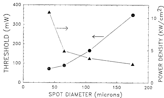
Figure 12: The effect of changes in the laser spot size on the threshold ignition irradiance (power density) and threshold ignition power for TiH_{1.65}/KClO_4 in 2.9 MPa argon [52].
