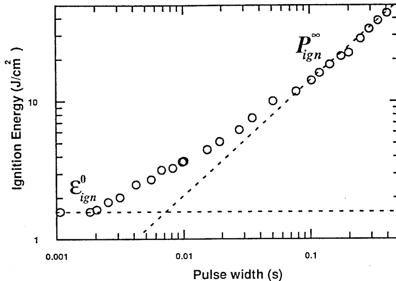
Figure 5: Ignition energy versus pulse width for Mg/NaNO 3 . Observe the two ignition regimes: one for long pulses and one for short pulses [43].
