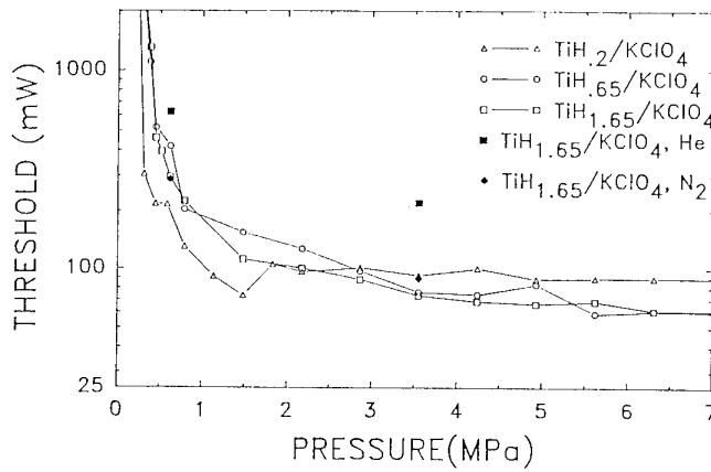
Figure 10: Change in the ignition power threshold for Ti/KClO_4 as a function of pressure and the type of gas (pulse width 3 ms) [52].
