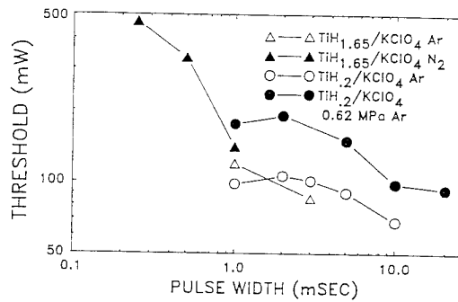
Figure 11: Variation in the threshold ignition power with laser pulse width for TiH_x/KClO_4 pyrotechnic compositions (spot size 65 \mu m ) [52].
