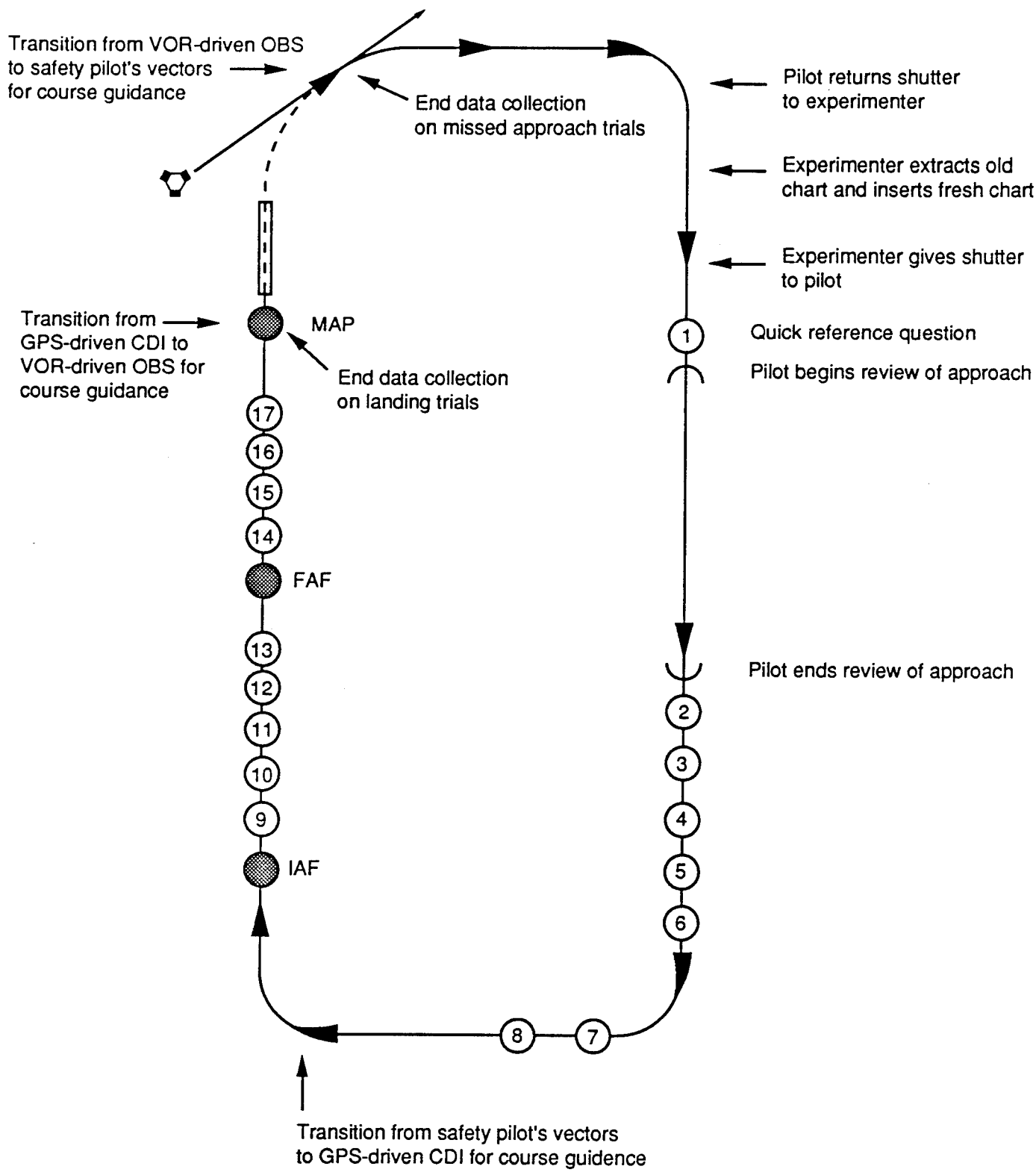
Figure 9. Sequence of Pilot, Safety Pilot, and Experimenter Activities During an Approach Trial
