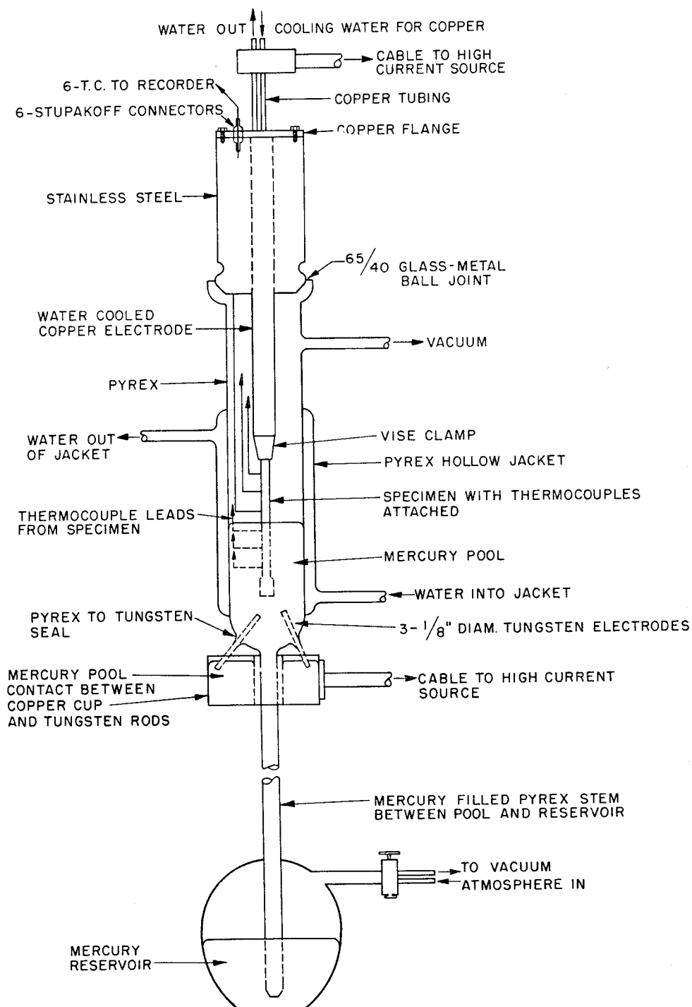
FIGURE 5 URANIUM FILAMENT FURNACE APPARATUS FOR ANNEALING SPECIMEN AS FILAMENT (Similar to Vacuum Filament Crystal Device-KAPL)
