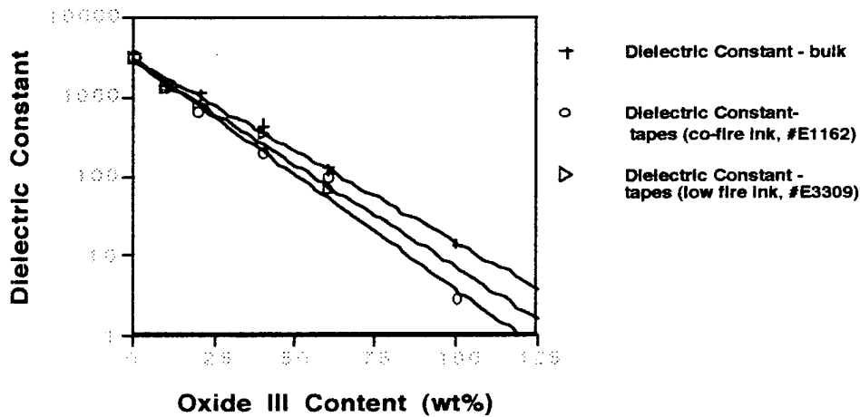
FIGURE 4. Semi-log Plot of Dielectric Constant versus Oxide III Content of the Bulk Ceramics and the Tapes Measured at 1 KHz (lines represent best fit to the data).
