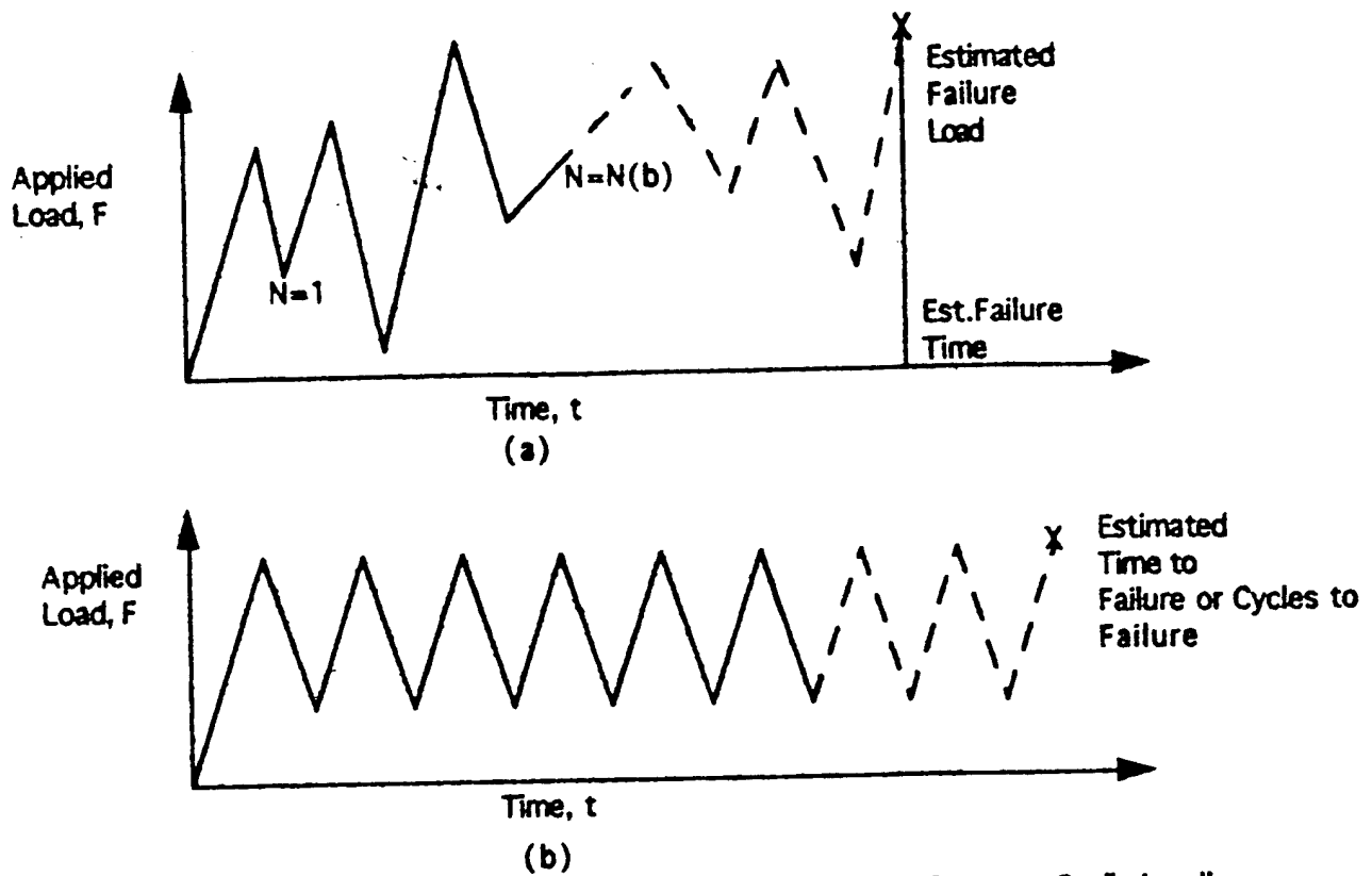
Figure 7 Predicting Fracture Failure in Random Cyclic Loading and In Constant Cyclic Loading
