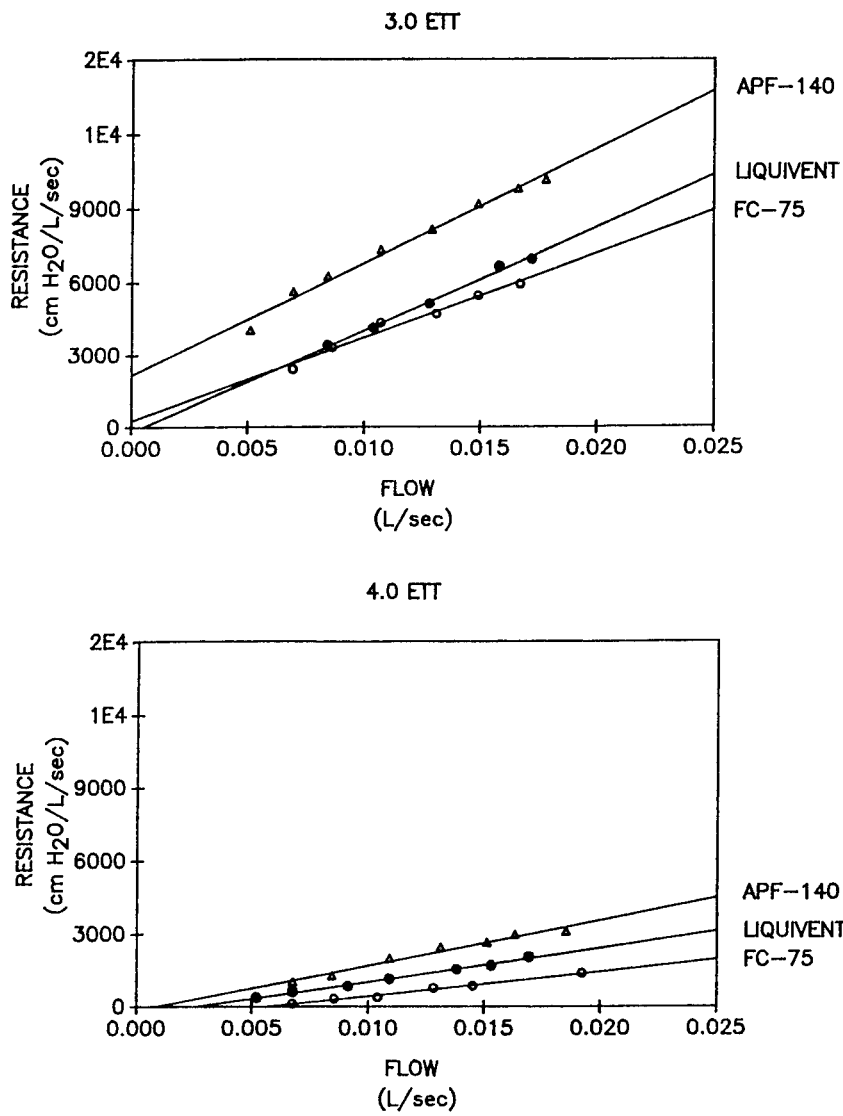
FIGURE I: Resistance and Flow Relationships For Three PFC Fluids Evaluated with Two Neonatal Endotracheal Tubes
