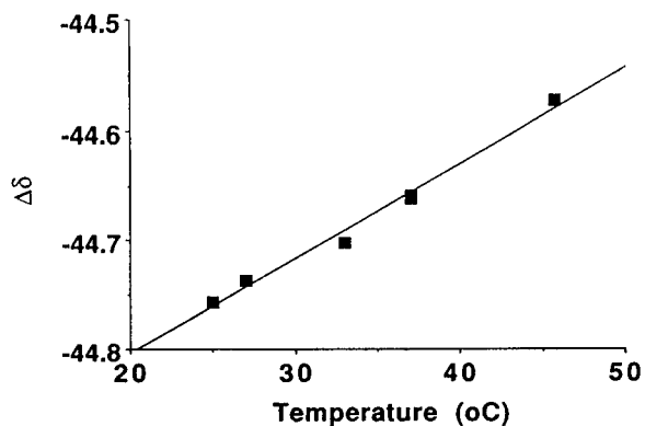
FIGURE 6 Internal chemical shift difference between the CF 3 and CF 2 (-45 ppm) resonances of Oxygen at 4.7 T as a function of temperature at 0%pO 2 :
