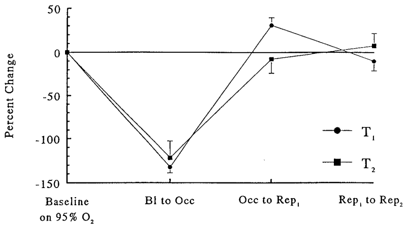
FIGURE 3: Change in pO_2 in the abscess of rabbit #1. The values were obtained by dividing the 1/T_1 and 1/T_2 measurements by their respective calibration slope.
