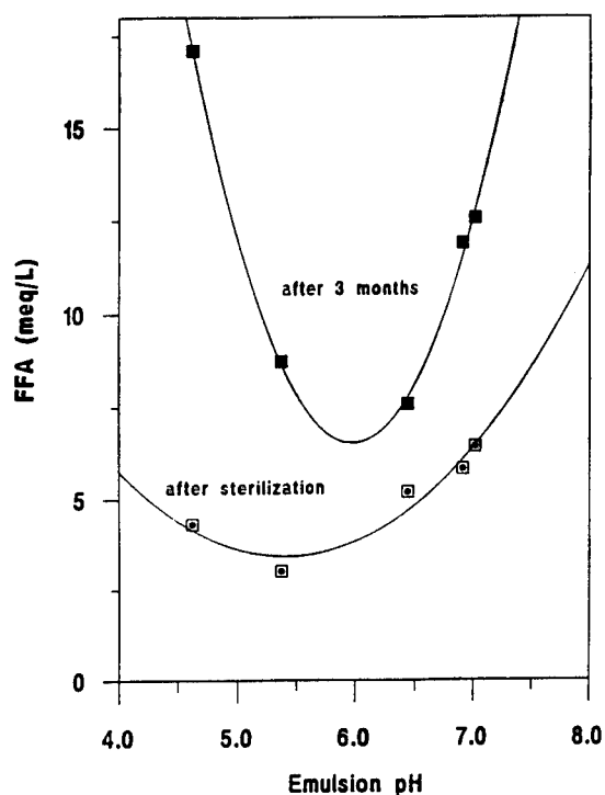
FIGURE 3. FFA in emulsions with 30 mM phosphate buffer at 0 and 3 months vs emulsion pH.
