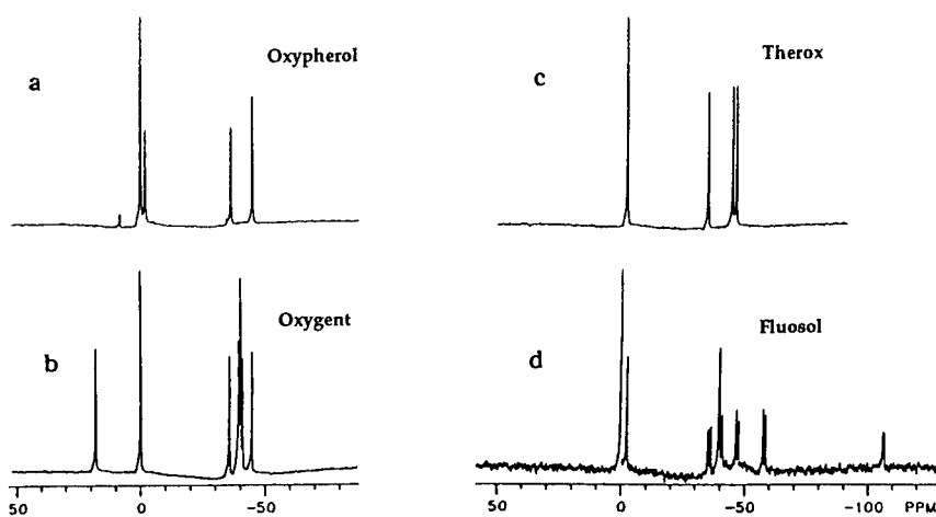
FIGURE 1 282 MHz 19 F NMR spectra of commercial PFC emulsions: a) Oxypherol (20% w/v emulsion of perfluorotributylamine (PFTB), Alpha Therapeutics), b) Oxygent™ (90% w/v emulsion perflubron [perfluorooctyl bromide, PFOB], Alliance Pharmaceutical Corp.), c) Therox (40% w/v emulsion of trans-1,2 bis-(perfluorobutyl)-ethylene, Du Pont) and d) Fluosol (emulsion of 14% w/v perfluorodecalin and 6% w/v perfluorotripropylamine (PFTP), Alpha Therapeutics). CF 3 of each emulsion is essentially coincident and set to 0 ppm. There is some confusion in the literature regarding spectral assignments [12, 25, 31, 32] and it may be preferable to refer to resonances by their chemical shift. CF 2 's occur ~ 40 ppm upfield, whilst CF 2 X (heteronucleus) are shifted downfield.
