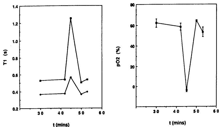
FIGURE 3 The variation of T_1 and calculated myocardial pO_2 with global ischemia and reperfusion for a perfused Oxypherol-loaded rat heart (Reproduced from Mason et al [18]). CF_3 □ and CF_2 ●.
