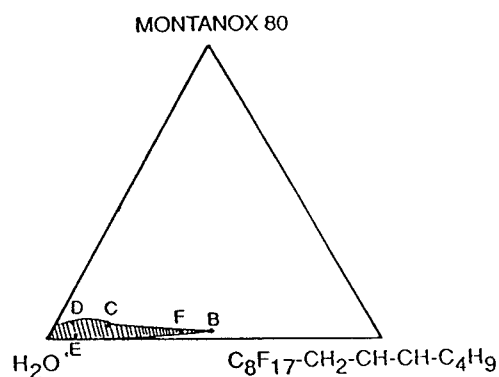
FIGURE 3 - Pseudoternary phase diagram of the system H 2 O-Montanox 80 C 8 F 17 -CH 2 -CH=CH-C 4 H 9
