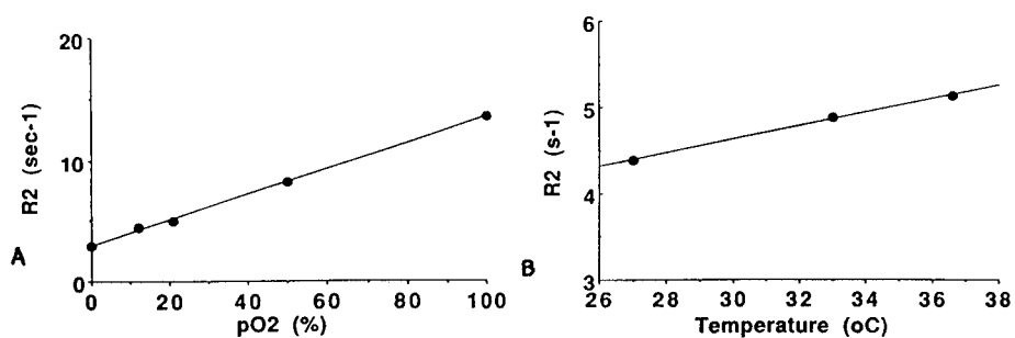
FIGURE 5 The variation of R 2 with pO 2 and temperature for the CF 2 Br resonance of Oxygen at 4.7 T.
