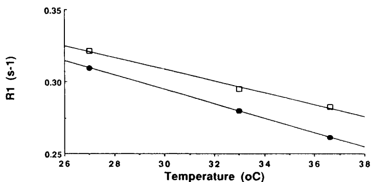
FIGURE 3 The variation of R_1 with temperature in the absence of oxygen ( pO_2=0\% ) for Oxygen at 4.7 T: ● CF 3 R_1 = 0.444 - 4.97 \times 10^{-3} (°C) and □ CF 2 Br R_1 = 0.432 - 4.10 \times 10^{-3} (°C).
