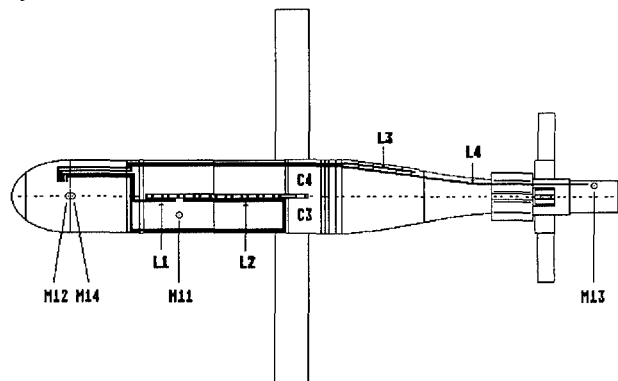
Fig.5.4.1: Route of the four selected lines L1, L2, L3 and L4 in the test object
