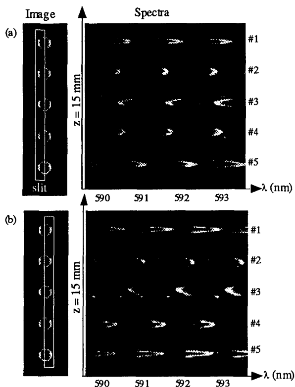
Figure 14 At medium magnification (5x), the CCD image of the lasing droplets (15 mm below the orifice) as they appear at the entrance slit (250 \mu\text{m} wide) of a spectrograph (left column). For (a) the right-half rim and for (b) the left-half rim is imaged onto the slit. The spatially preserved wavelength-dispersed data captured by a CCD camera are shown on the right side. Note the \supset - and \subset -shaped curves are better resolved spatially than in Fig. 13.
