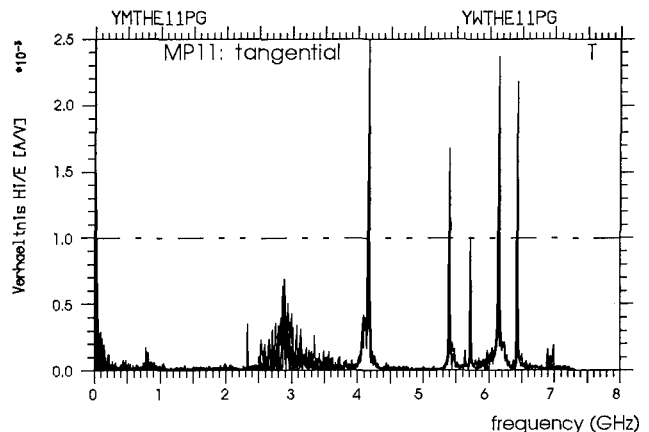
Fig.5.3.6: Magnetic field H_t/E_e behind the partition in the middle of the front chamber (M11) in position T
