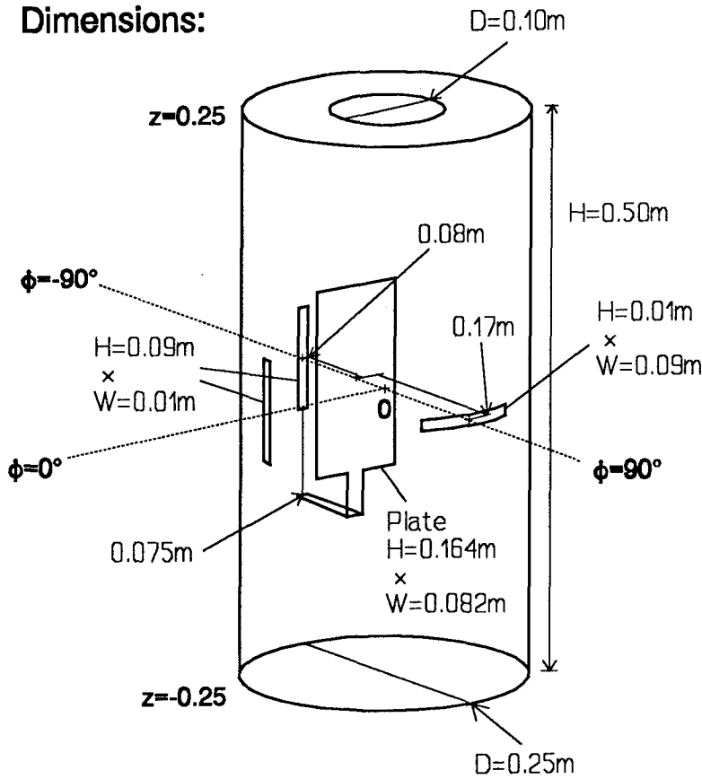
Figure 6. Cylinder dimensions and pulse orientations
