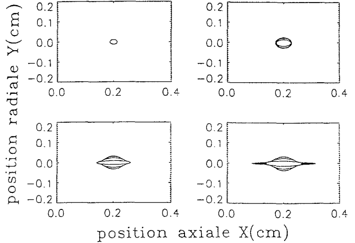
Figure 6 : Electron density distribution of a "plasmoid" in logarithm scale (between 10^{10} and 10^{14} \text{ cm}^{-3} ) at four times (8, 12, 16 and 18 ns) in a 4.5 MV/m average field, in ambient atmosphere
