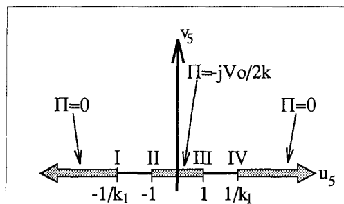
Figure 10 : Collinear slots, in w_5 -plane, after bilinear mapping
