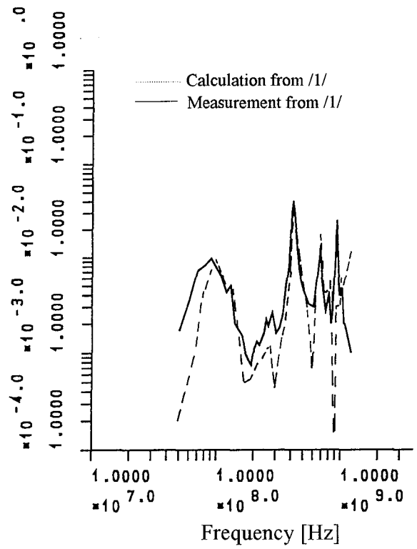
Fig. 9b: Voltage at the end of the receiving wire from /1/
