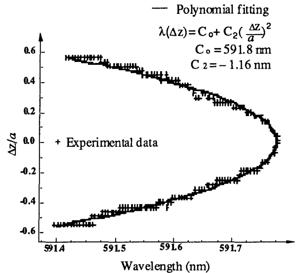
Figure 17 The + symbols designate the image-artifact corrected \lambda(\Delta z) data extracted from one of the \supset -curves shown in Fig. 15(b). The solid curve is the second-order polynomial fit \lambda(\Delta z) = C_0 + C_2(\Delta z/a)^2 . To reach the least-squared-error, C_0 = 591.8 \text{ nm} and C_2 = -1.16 \text{ nm} .
