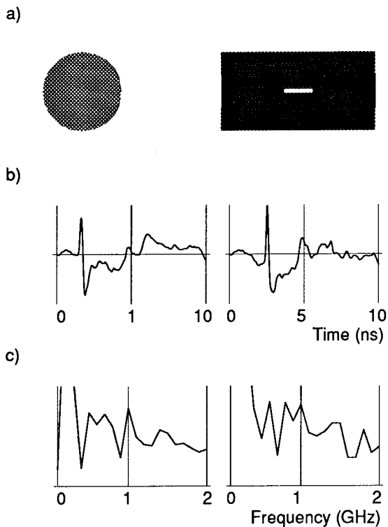
Figure 1. Experimental results obtained with ultrawideband radar. a) Aspect of the target facing the antenna and probe. b) Integrated time domain responses from D - dot probe. c) Fourier transforms of time domain responses.
