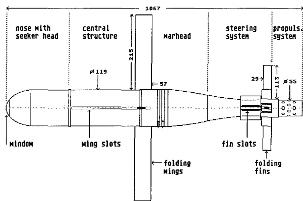
Fig.5.1: Outline and dimensions of the Bussard
