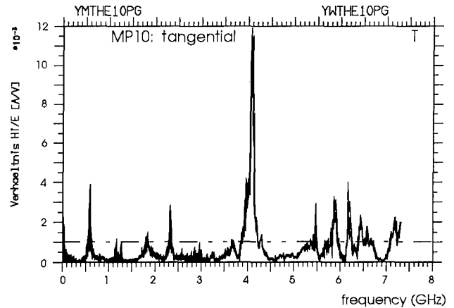
Fig.5.3.5: Magnetic field H_t/E_e in the middle of the rear chamber (M10) in position T
