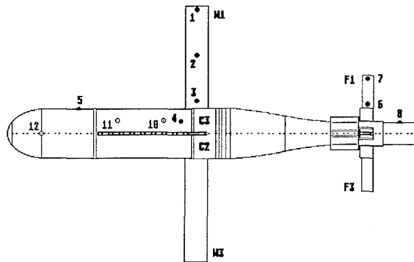
Fig.5.2.1: Location of the eight measuring points at the surface of the Bussard ( M10 , M11 and M12 are in the interior)
