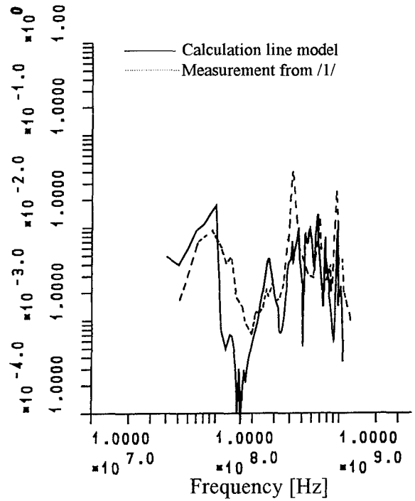
Fig. 10b: Voltage at the end of the receiving wire received by the line model
