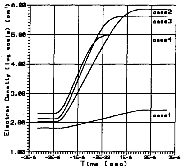
Fig.1(b) Electron density vs time.
