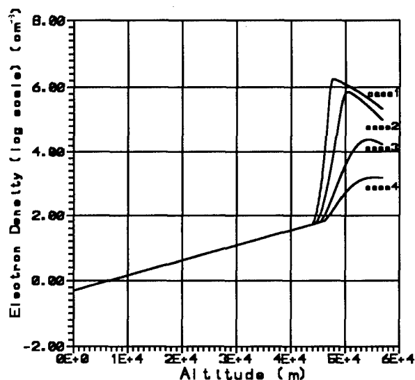
Fig. 2(b) The maximum (in time) electron density distribution for four cases of different carrier frequencies. [Normalized Power: 9 \times 10^{-6} , Width: 5.4 \mu sec, Frequency: case 1 (0.5GHz), case 2 (1GHz), case 3 (1.3GHz), case 4 (1.5GHz)]
