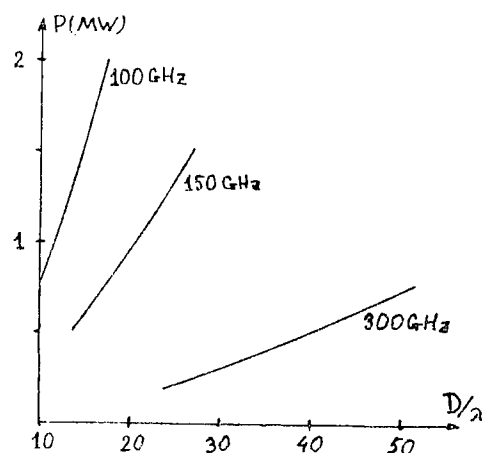
FIGURE 2. Estimation of maximum power from gyrotron
