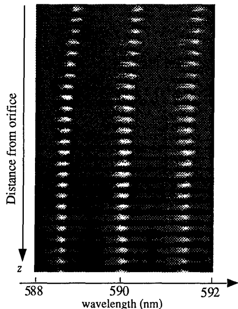
Figure 10 The spectrally and spatially resolved CCD recording of the lasing droplets in a continuous droplet stream. All the droplets are uncharged. The distance between the center of the droplet stream and the orifice is 20 mm.
