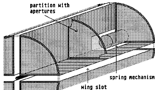
Fig.5.3.1: Perspective drawing of an empty chamber
