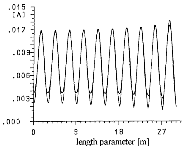
Fig.3b: Current distribution on the monopole of fig. 4 for receiving due to NEC2 and the line model ( f=100 MHz)
