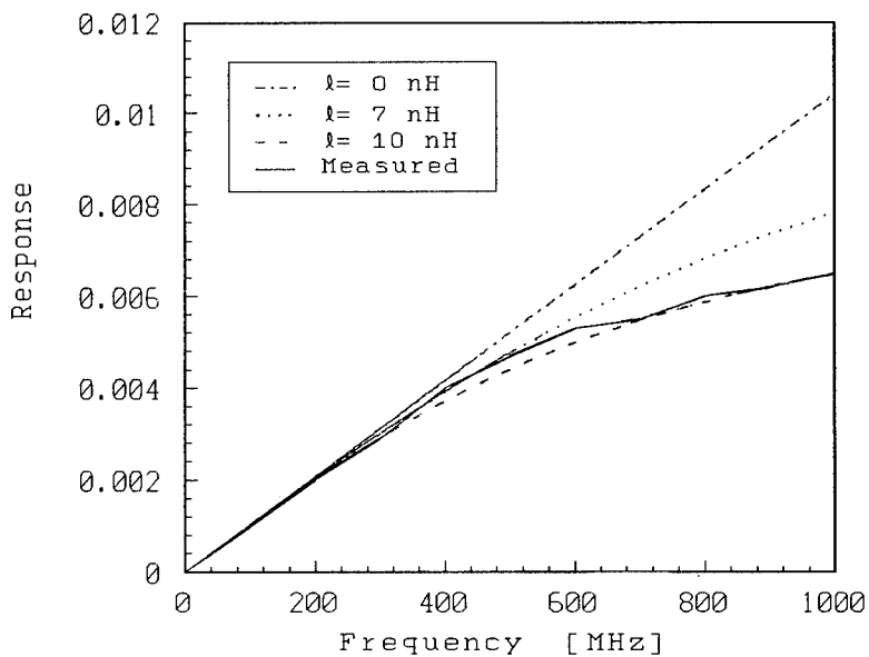
Figure 8: The response of the field probe depicted in Figure 6 when tested in a TEM cell. The inductance, l , of the probe is calculated to be approximately 8 nH.
