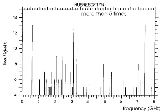
Fig.5.4.6: Frequency probability of the summarized resonances on the four lines in the Bussard (only for peaks occurring more than five times)
