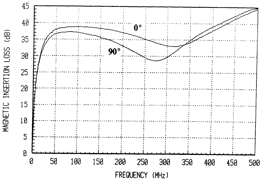
Figure 6 - Effect of Sample Orientation on Magnetic Shielding
