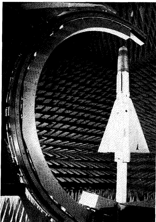
figure 3 : SOCRATE device
