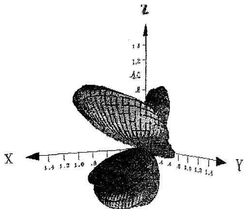
figure 10 : C.C.S at f = 920\text{ MHz} : max = 1.6 cm 2
