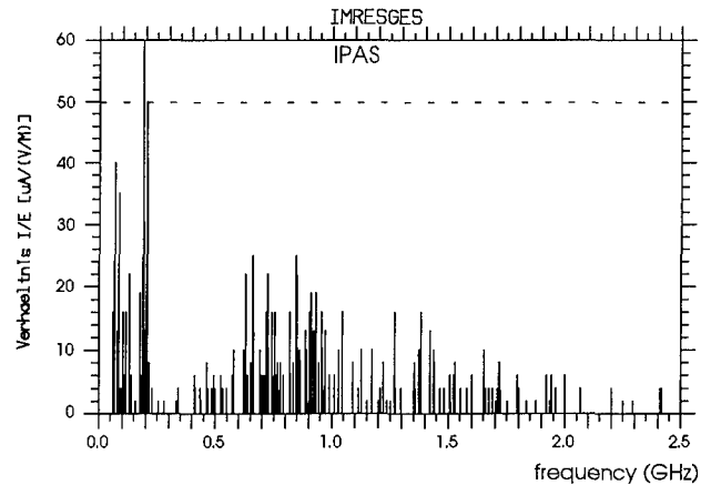
Fig.6.3.4: Amplitude spectrum of the summarized resonances on the examined ten lines in the IPAS
