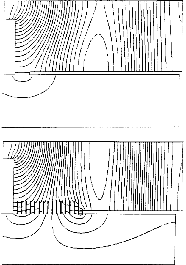
Figure 2 Narrow and extended gap geometries
