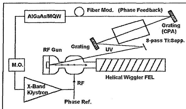
3. Experimental Arrangement
