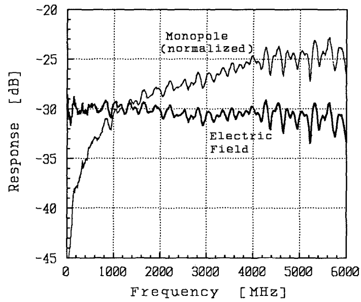
Figure 11: The E-field response of a 1m long GTEM cell as measured by a short monopole. Although the magnitude varies a few dB both spatially (not shown) and with frequency, there are no deep nulls in the response.
