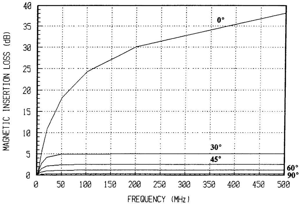
Figure 9 - Effect of Orientation on Magnetic Insertion Loss
