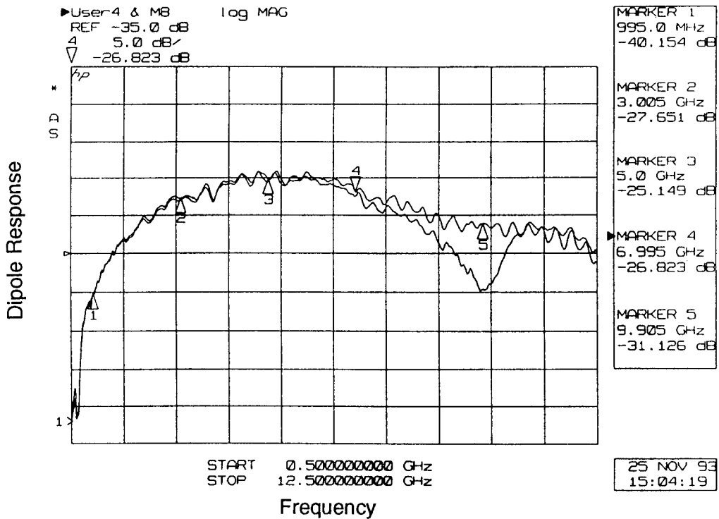
Figure 2: Response of the dipole depicted in Fig. 1. The measurement was made in an anechoic chamber with a standard gain horn antenna as a source. Although both sensors are physically virtually identical, there is clearly a difference in the response.
