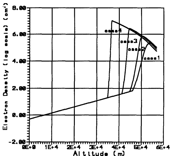
Fig. 2(a) The spatial distribution of the maximum (in time) electron density generated by a pulse for four cases of different incident power level. [Frequency: 1GHz, Width: 5.4 \mu sec, Normalized Power: case 1 ( 7 \times 10^{-6} ), case 2 ( 9 \times 10^{-6} ), case 3 ( 5 \times 10^{-5} ), case 4 ( 1 \times 10^{-4} )]
