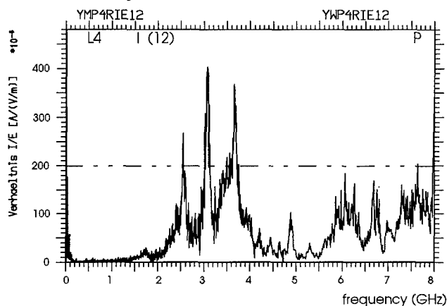
Fig.5.4.3: Short circuit current I_0/E_e on the left side (M12) of line L4 in position P
