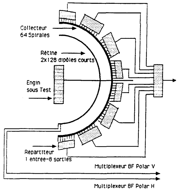
figure 4 : H.F. band, near field measurement device
