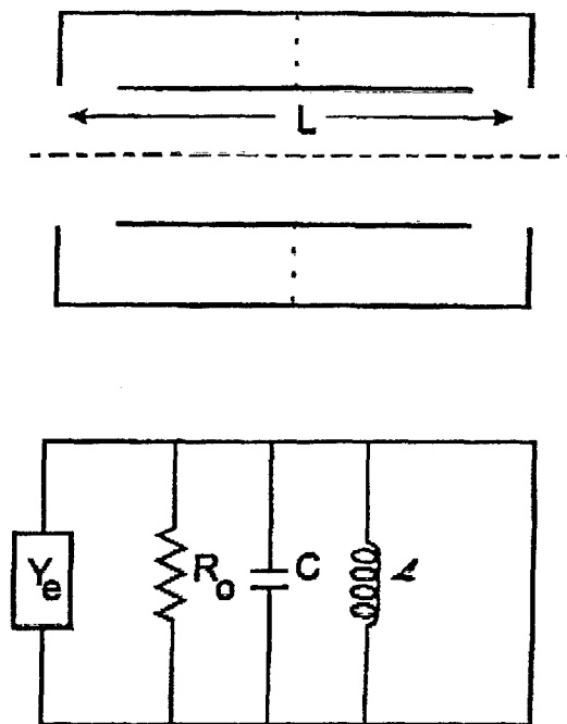
Figure 8 Simple cavity (top) and equivalent circuit (bottom)
