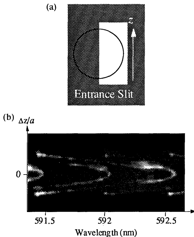
Figure 15 (a) At larger magnification (20x), the right half of circular image of a single droplet (10 mm below the orifice) fits into the entrance slit (800 \mu\text{m} wide) of a spectrograph. (b) The spatially preserved wavelength-dispersed data captured by a CCD camera.
