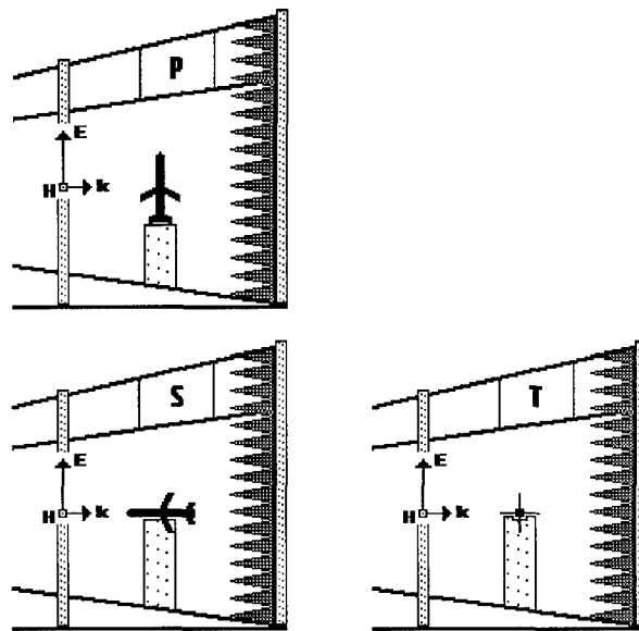
Fig.4.1: Test object in three orthogonal directions ( P , S , T ) in the rear part of the TEM simulator
