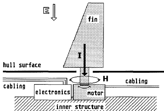
Fig.4.3: Typical coupling path 'fin-cabling-inner structure'
