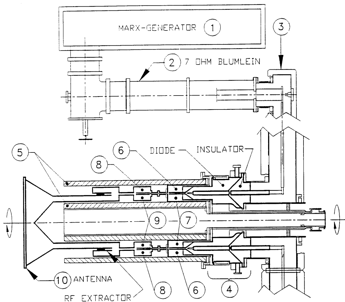
Figure 6 Schematics of the Triaxial RKA.
