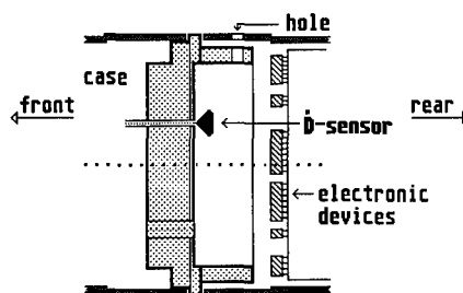
Fig.7.3.1: E-field measurement on M12 near electronic devices
