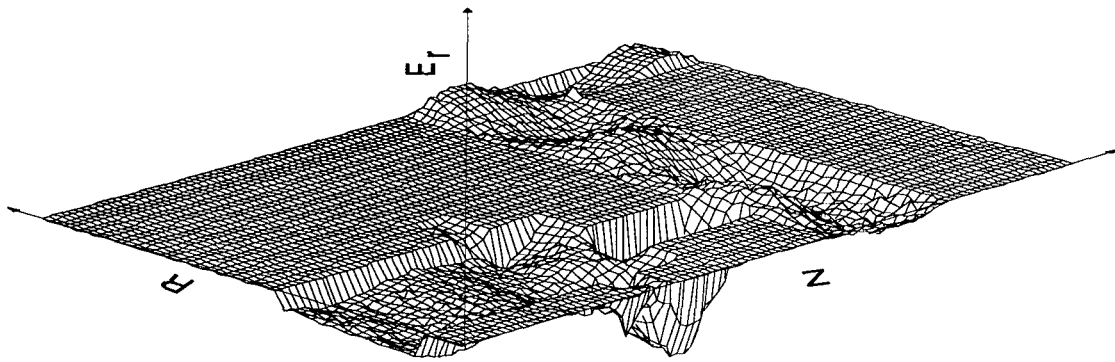
Figure 3. Perspective plot of the radial electric field showing the rf being generated in the cavity, propagating radially outward towards the coaxial line and leaving the system through the coax.
