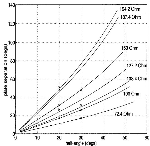
Figure 12 : Calculated Z_o curves for free-space antenna structure with experimental values (*)
