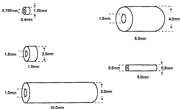
Fig. 7 Some bead sizes and shapes tested.
