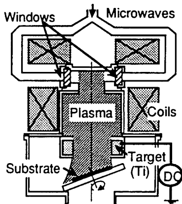
ECR Plasma Deposition for Conductive Films
