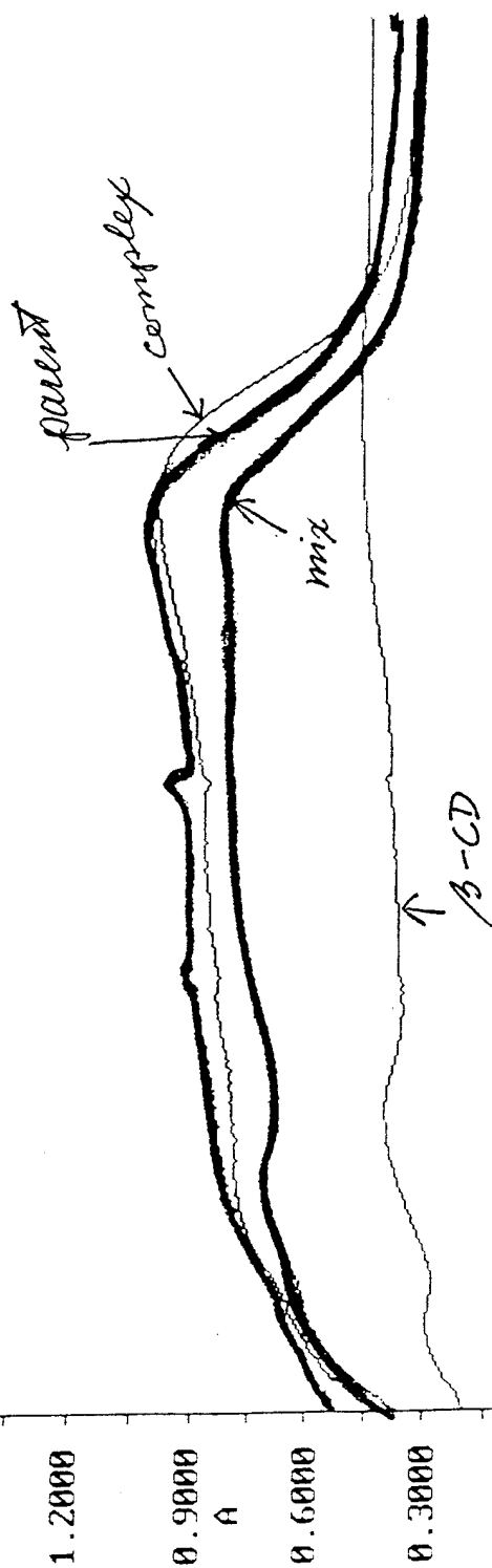
Inf: (12) 2-AMINO-6-NITROBENZOTHIAZOLE OVERLAY OF BCD, PARENT, MIX, & COMPLEX
