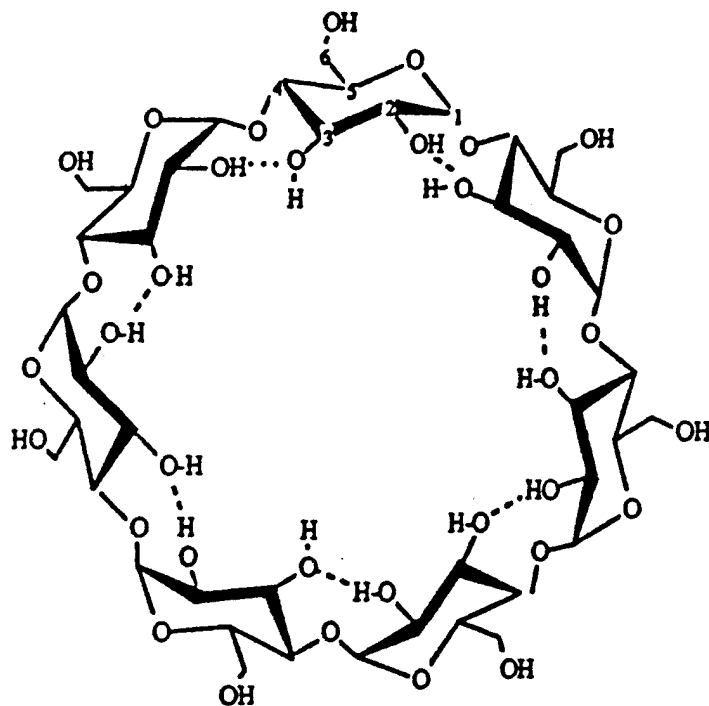
CHEMICAL STRUCTURE OF β-CYCLODEXTRIN
