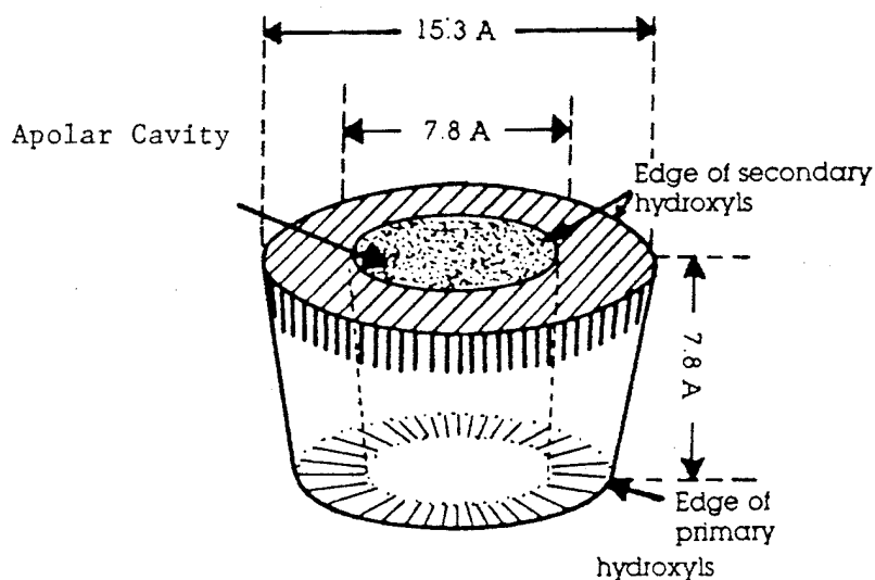
DIMENSIONAL STRUCTURE OF β-CYCLODEXTRIN
