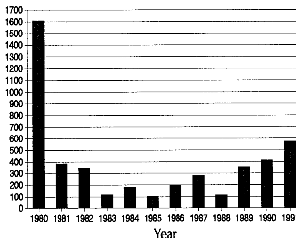
Figure 20. Index of Fall Abundance of Smelt 1980-1991 (CDWR 1991)
