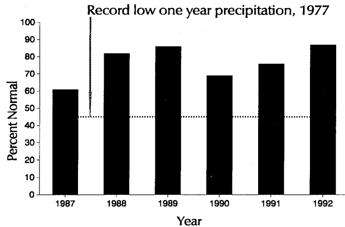
Figure 6. Water Year Runoff: 1987-1992
