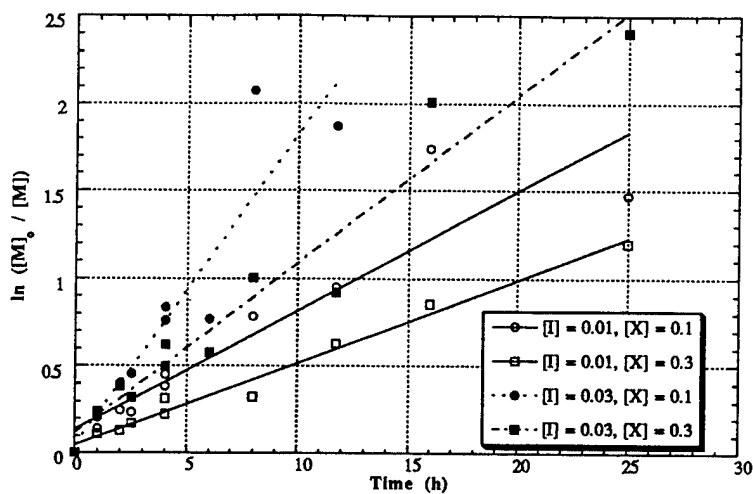
Fig. 4 Kinetics for the bulk polymerization of styrene at 70 °C, [I] = AIBN, [X] = 1 - phenylethyl iodide.
