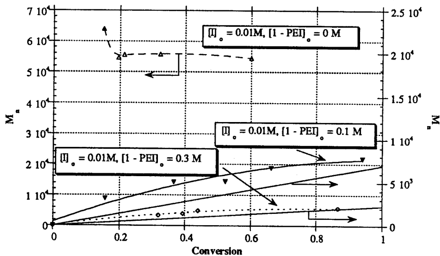
Fig. 5 Dependence of M_n upon conversion for the bulk polymerization of styrene at 70 °C, [I] = AIBN, [1-PEI] = 1 - phenylethyl iodide.
