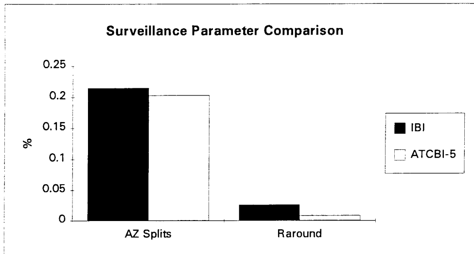
FIGURE 4.1-4. FILTERED SPLITS AND RINGAROUND
