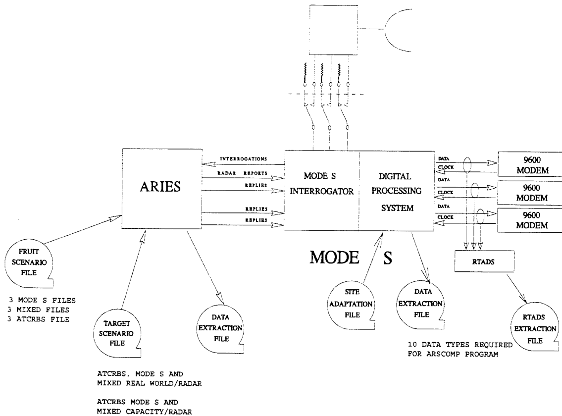
FIGURE 4.4-1. SURVEILLANCE BASELINE - REPORT PARAMETERS
