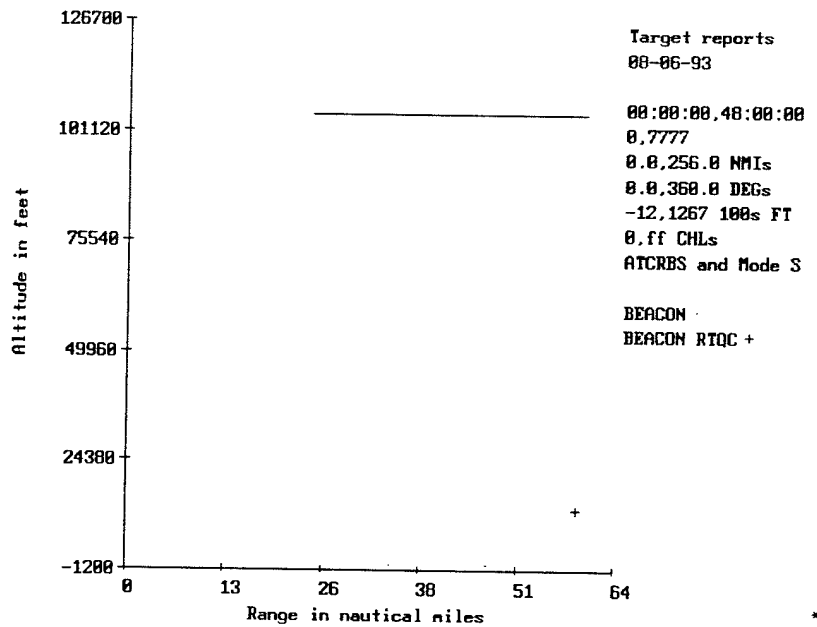
FIGURE 4.7-4. SUBTEST 6, RANGE VERSUS ALTITUDE
