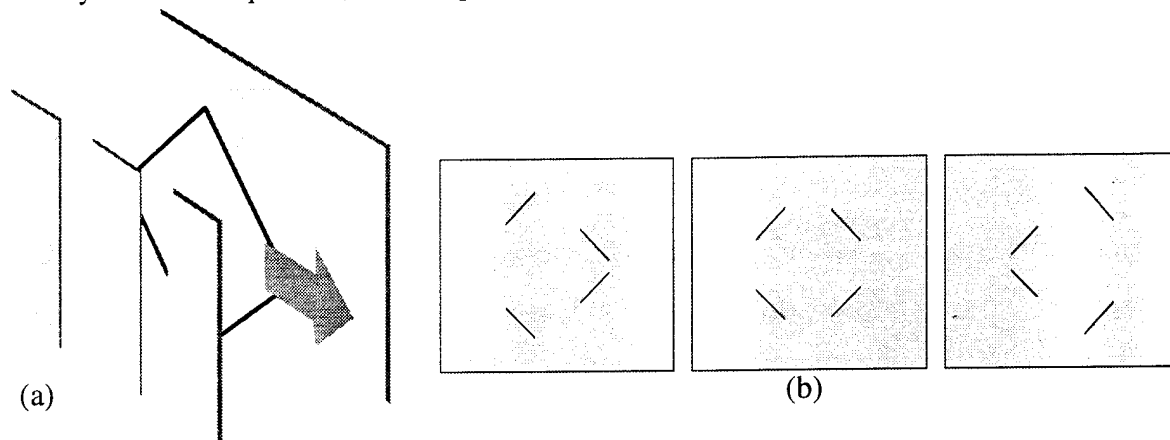
Figure 1. (a) The setup used in our experiments. (There is no physical significance to the absolute depth differences between the occluders, diamond and background shown in this figure. They are indicative only of the depth ordering used to generate the 2D motion sequences.) We used the Macromind Director software package running on a Macintosh Quadra 700 to generate the sequences. The sequences were presented on a 16" monochrome monitor and subtended 7 degrees of visual angle at a viewing distance of 80 cm. The diamond's speed of oscillation was 0.7 degrees per second. (b) Three frames from sequence 'A': the diamond oscillating horizontally behind occluders that have exactly the same gray-level as the background.
