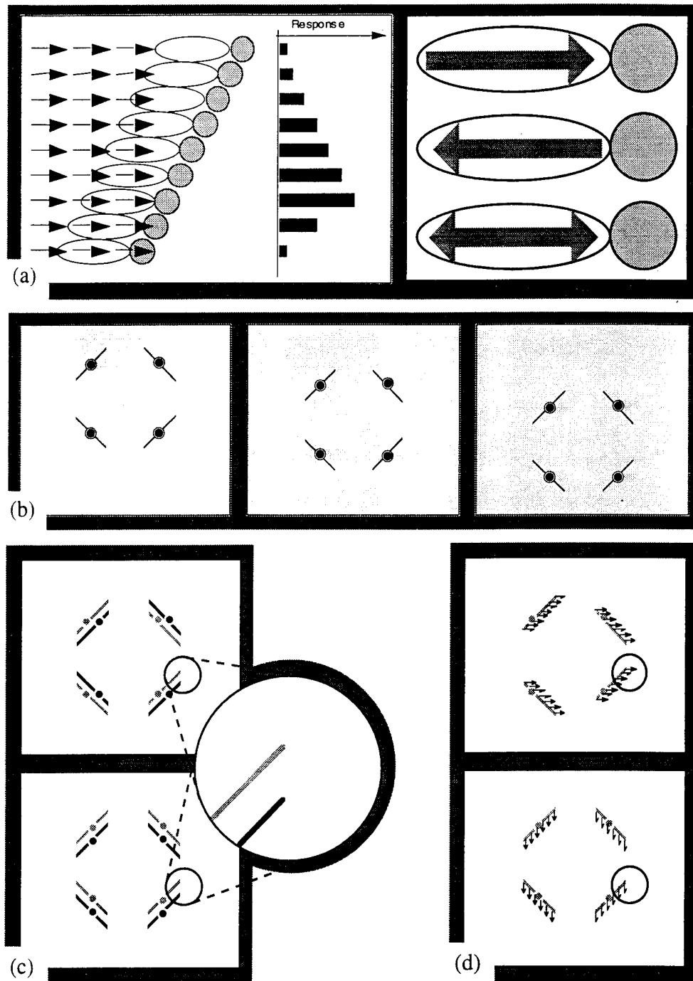
Figure 5. (a) A qualitative characterization of the predicted 'motion end-stopped' units. The left panel shows how the response is expected to vary as a function of the extent of overlap between a motion field and a unit's receptive field. The excitatory and inhibitory regions of the receptive field are represented by the white and speckled ovals respectively. As indicated in the right panel, the preferred direction of the unit needs to be aligned with its major axis to allow it to detect discontinuities in a motion-field along the motion trajectory. The discontinuities can be classified into two basic categories: those associated with the abrupt appearance of motion and those associated with its abrupt disappearance. These discontinuities can either be detected by two different units with opposite preferred directions or by one unit that is sensitive to the motion field's orientation but not its sign. (b) Three frames from sequence 'D'. (c) Due to the aperture problem, the local patterns of motion in sequences 'C' and 'D' are identical (they do, however, differ in phase). (d) The global motion fields in the two sequences are, however, very different.
