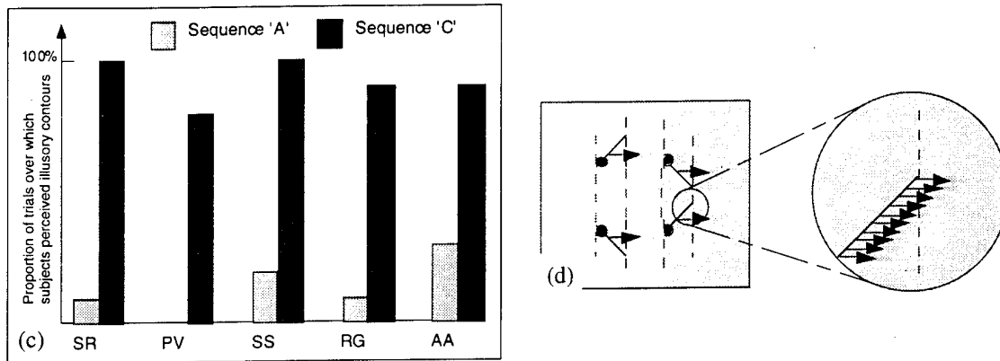
Figure 4. (Contd.) (c) A summary of the results obtained with experiment 2. The imposition of a horizontal motion field induced subjects to perceive contours delimiting illusory occluding strips. (d) The percept with sequence 'C': strong subjective contours are reported at the indicated locations. As shown in the enlarged inset, the illusory contours coincide with the abrupt discontinuities in the horizontal motion-field.
