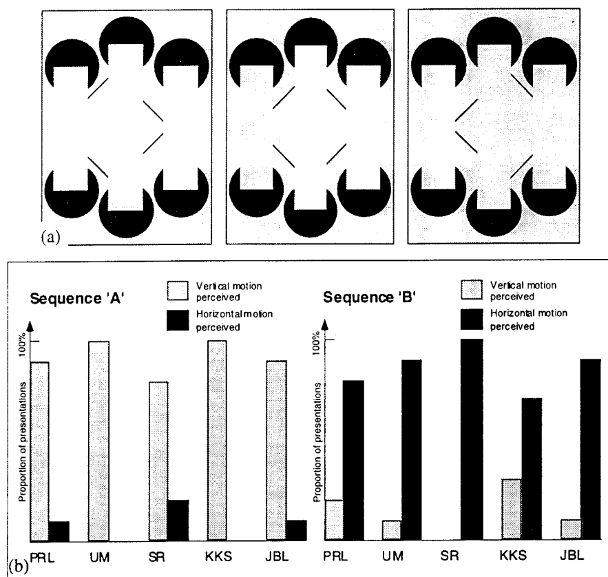
Figure 2. (a) Three frames from sequence 'B'. This is the same as sequence 'A' except for the inclusion of a few static figural elements that indicate the occluders' presence. (b) A summary of the results obtained with sequences 'A' and 'B' in experiment 1. For each of the five subjects, the inclusion of the static figural elements strongly biases the percept from being one of motion in the vertical direction to one of horizontal motion. (Contd. on next page)
