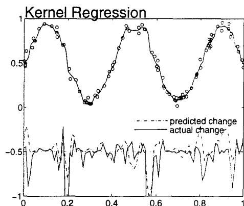
Figure 3: Fit to data and correlation for kernel regression.
