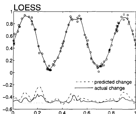
Figure 4: Fit to data and correlation for LOESS model.
