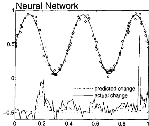
Figure 1: The upper portion of the plot indicates the neural network's fit to noisy sinusoidal data. The lower portion of the plot indicates predicted and actual changes in the network's average estimated variance when \tilde{x} is queried and added to the training set, for \tilde{x} \in [0, 1] . Changes are not plotted to scale with fits.
