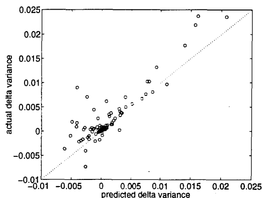
Figure 6: Predicted vs. actual changes in model variance for LOESS on the arm kinematics problem. 100 candidate points are shown for a model trained with 50 initial random examples. Note that most of the potential queries produce very little improvement, and that the algorithm successfully identifies those few that will help most.
