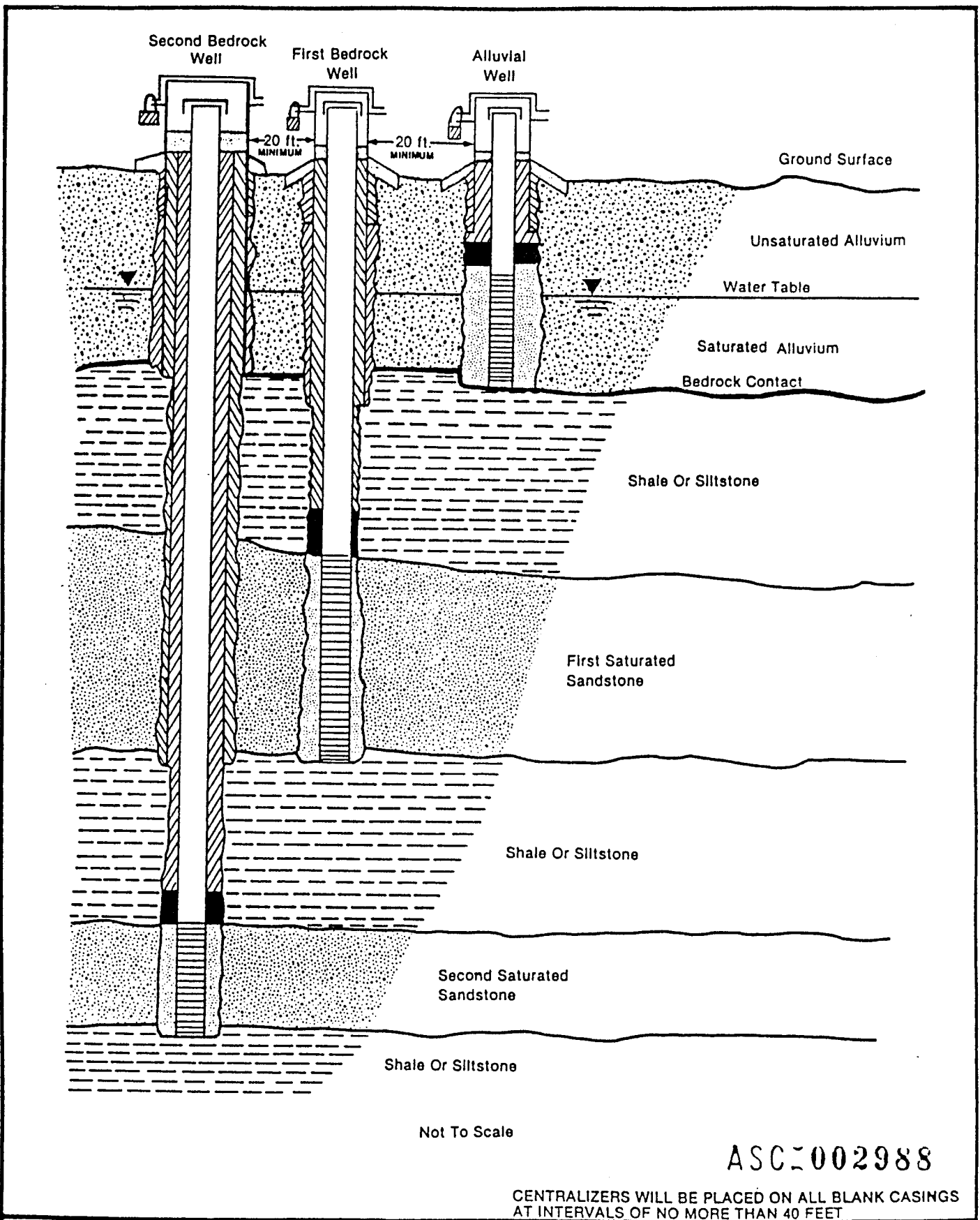
Figure 3.2-3 SCHEMATIC DRAWING OF A TYPICAL CLUSTER WELL INSTALLATION SOURCE: ESE, 1986
