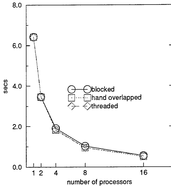
Figure 2: Measured runtime for parallel regular Jacobi program versions with N=512 , ITER=20 , B=1
