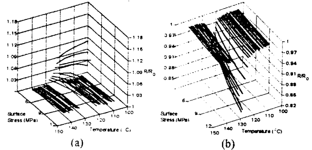
Fig. 5. Normalized resistance of a 3/30/3 layer trilaminate (0.30 at% La only) vs. surface stress and temperature, for regions under a) compression, b) tension.
