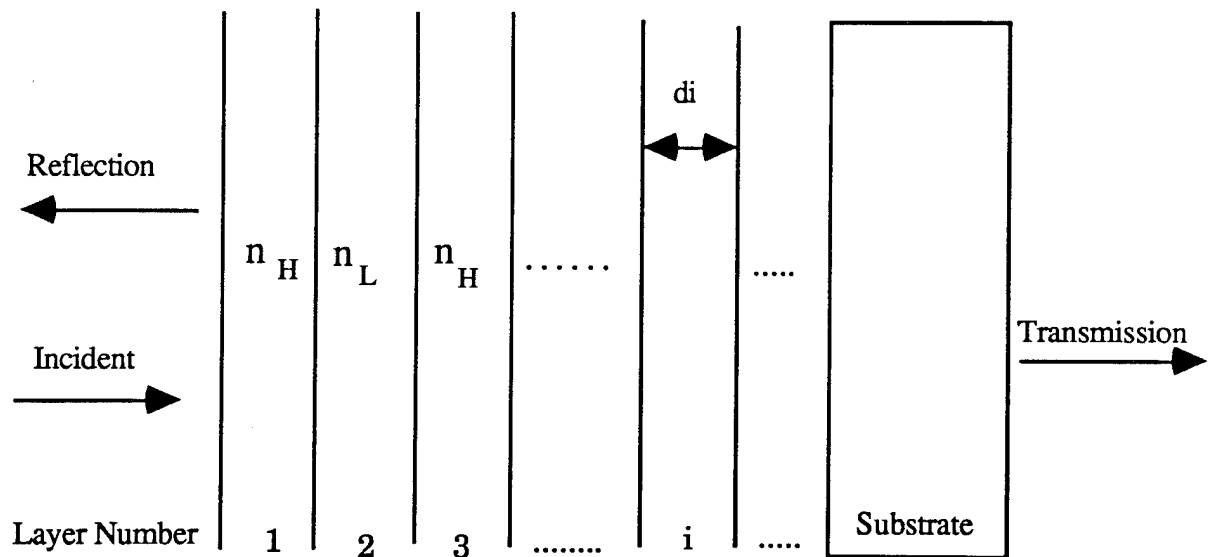
Fig. 1. Multilayers of optical thin films with high- and low- nonlinearity. The optical thickness ( d_i ) of each layer is (a) quarter of central wavelength for the quarter-wavelength scheme, (b) random between 100 to 200 nm for the random thickness scheme, and (c) sinusoidally modulated between 13 to 40 nm for the superlattice scheme.
