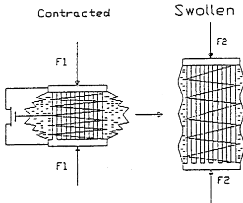
Figure 2- Modes of expansion and counterions of the ionic gel actuator
