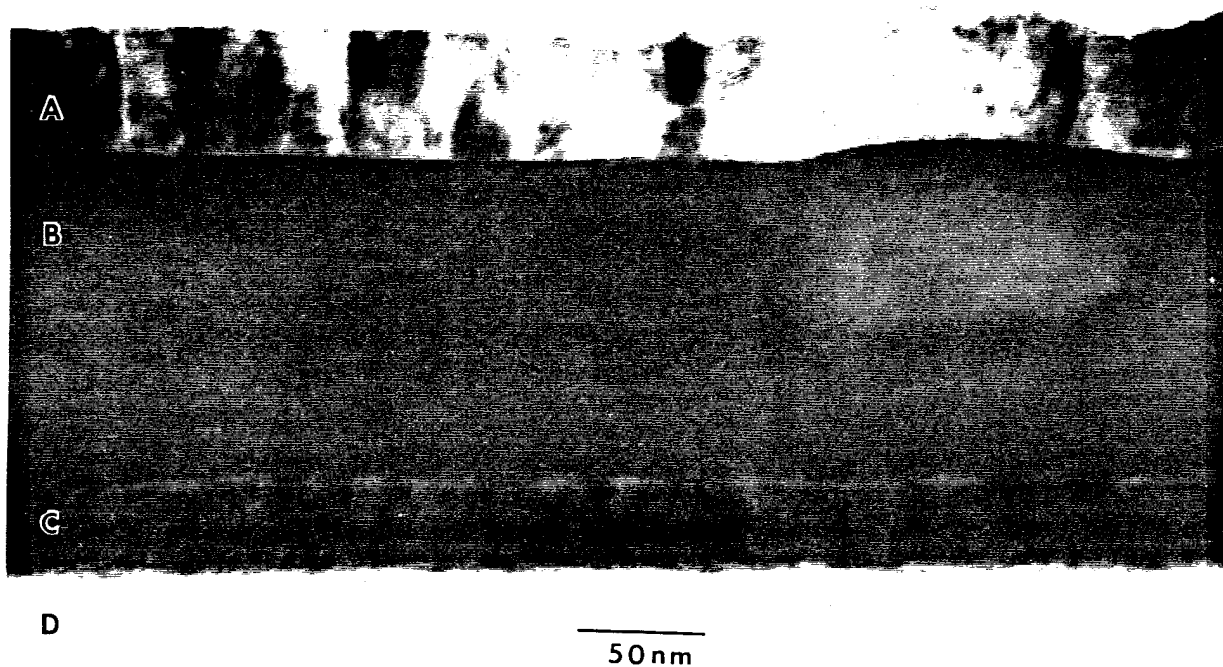
Figure 3. Cross-sectional TEM showing (A) BST ferroelectric, (B) Pt electrode, (C) ZrO_2 adhesion layer and (D) SiO_2 .
