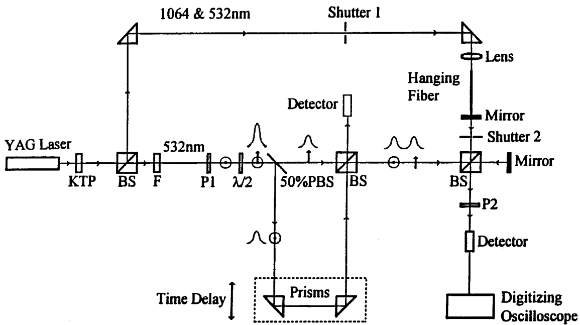
Figure 4: Fast actuator experiment.
