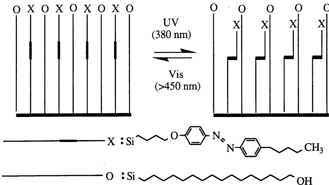
Figure 1. Principle : irradiation will reversibly alter the composition at the surface which will control wettability and adsorption.
