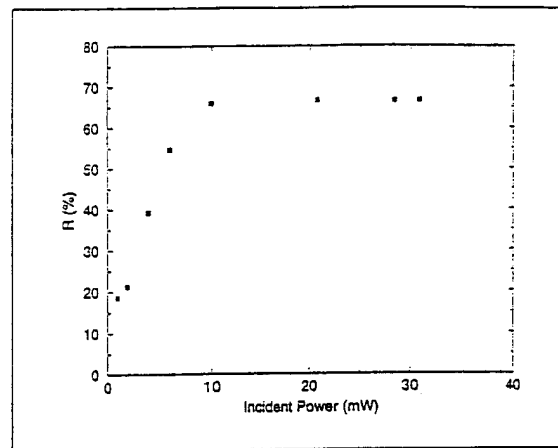
Figure 5: Reflectivity of our device as a function of laser power at an ambient temperature of 27°C.
