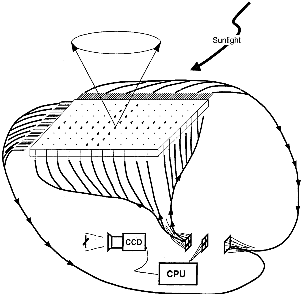
Figure 1: Schematic Diagram of concept. In addition to direct transfer of images to the skin, the optical system could be used to gather optical information from the exterior, transmit images/data optically via line-of-sight to any viewer, or identify concealed material with a narrow-bandpass optical signature.
