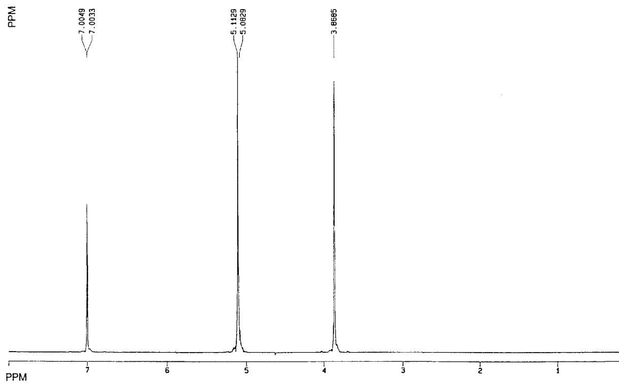
FIGURE 20. ^1\text{H} NMR Spectrum of Aconitic Acid in \text{D}_2\text{O} .
