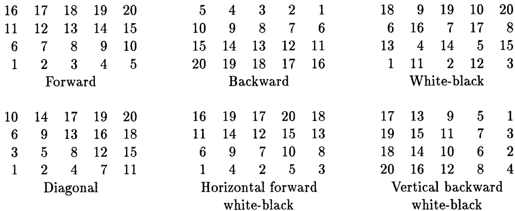
Figure 3.3.1: Grid point orderings for point Gauss-Seidel.
