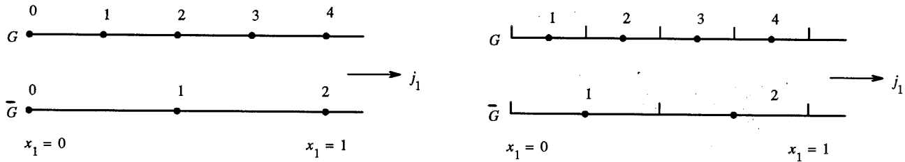
Figure 5.1.1: Vertex-centered and cell-centered coarsening in one dimension. (• grid points)
