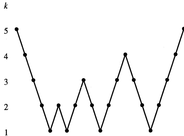
Figure 6.3.2: F-cycle diagram.
