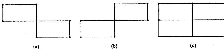
Figure 3.3.3: Discretization stencils.
