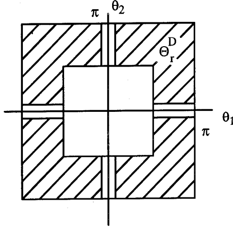
Figure 4.4.3: Rough wavenumber set ( \Theta_r^D , hatched) in two dimensions, with exclusion of \theta_\alpha = 0 modes; standard coarsening.
