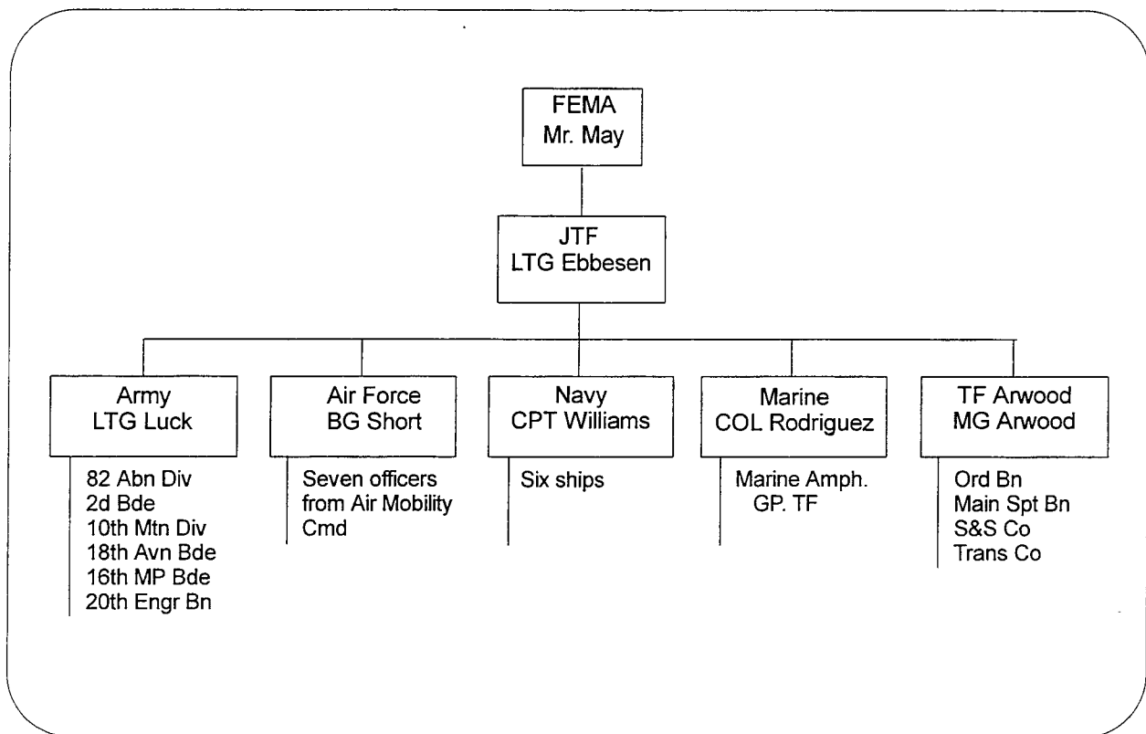
Figure 2-2. JTF organization
