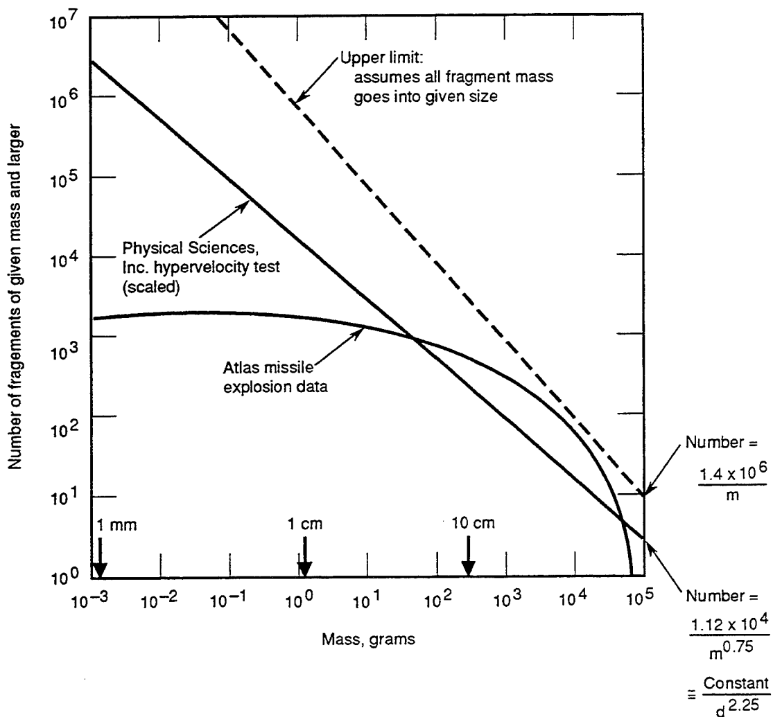
Figure 10. Expected number of fragments from the breakup of a 1400-kg satellite.
