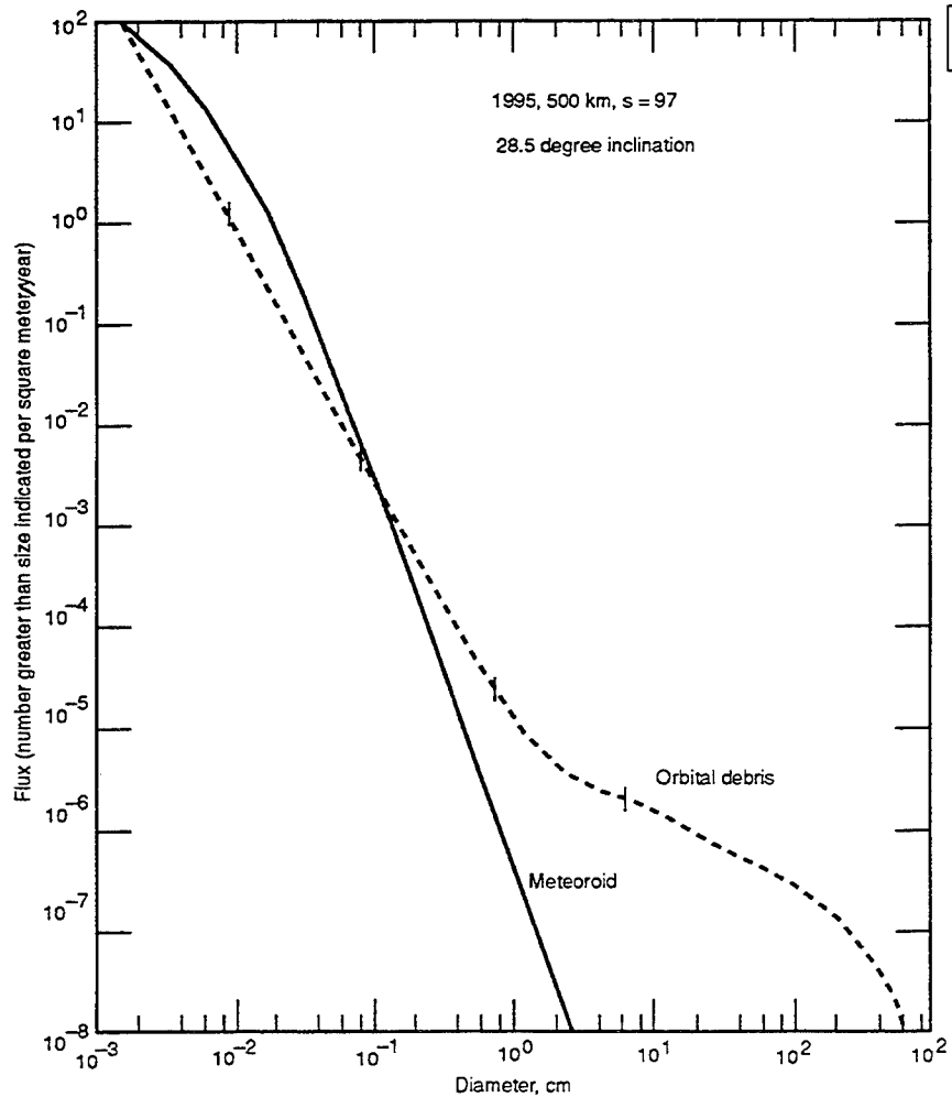
Figure 1. Comparison of meteoroid and orbital debris fluxes as a function of size.
