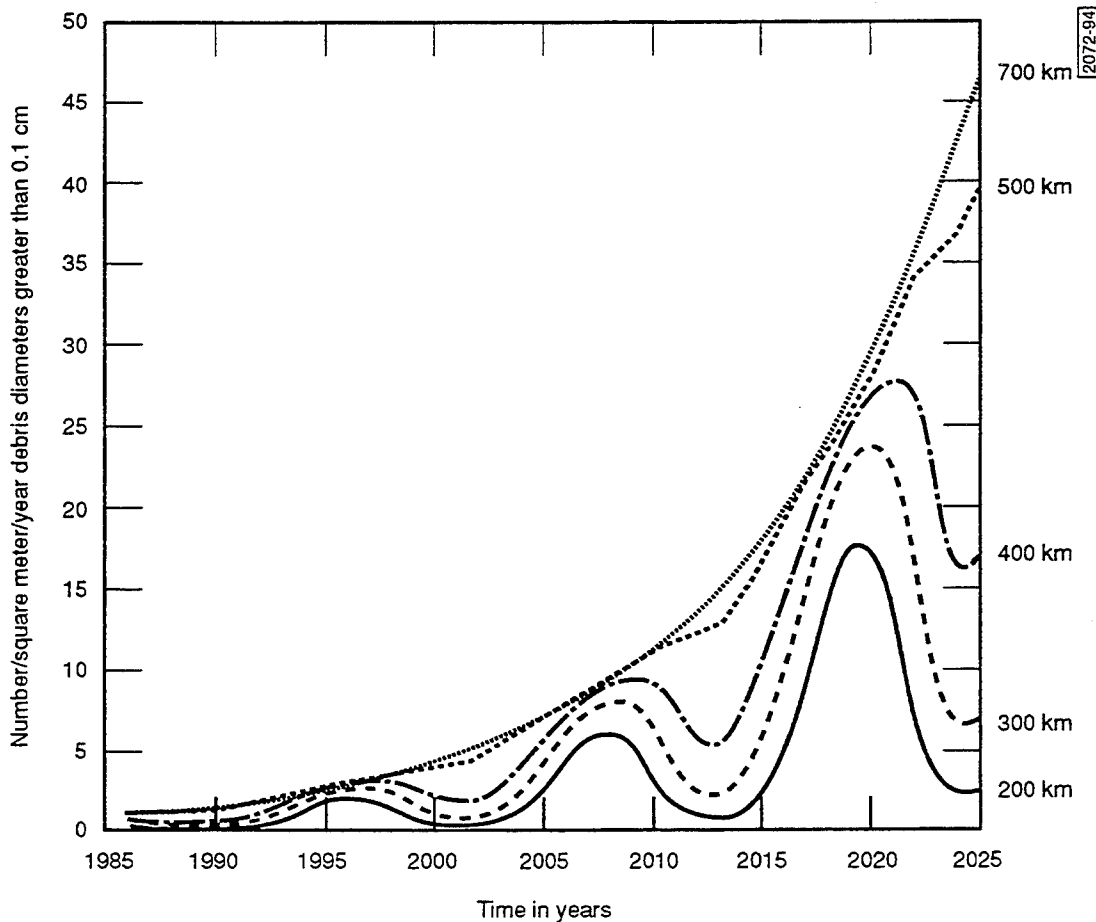
Figure 5. Dependence of debris flux on solar activity and altitude (from Ref. 13).
