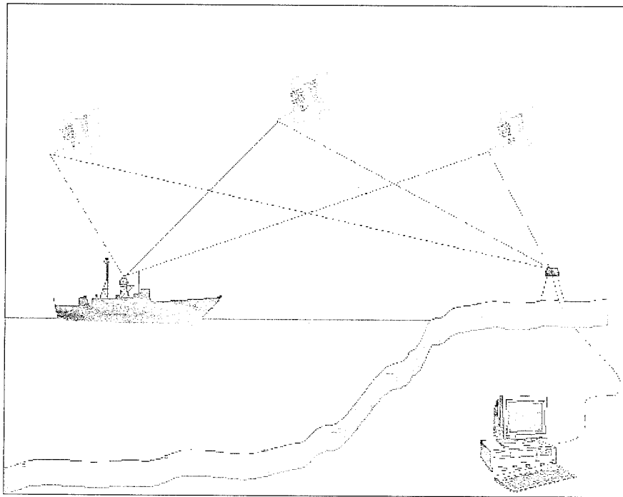
Figure 1. Three basic components of GPS-based surveying: the satellite-based signal transmitters, the mobile or stationary signal receivers, and computer software for calculating real-world coordinates from the signal
