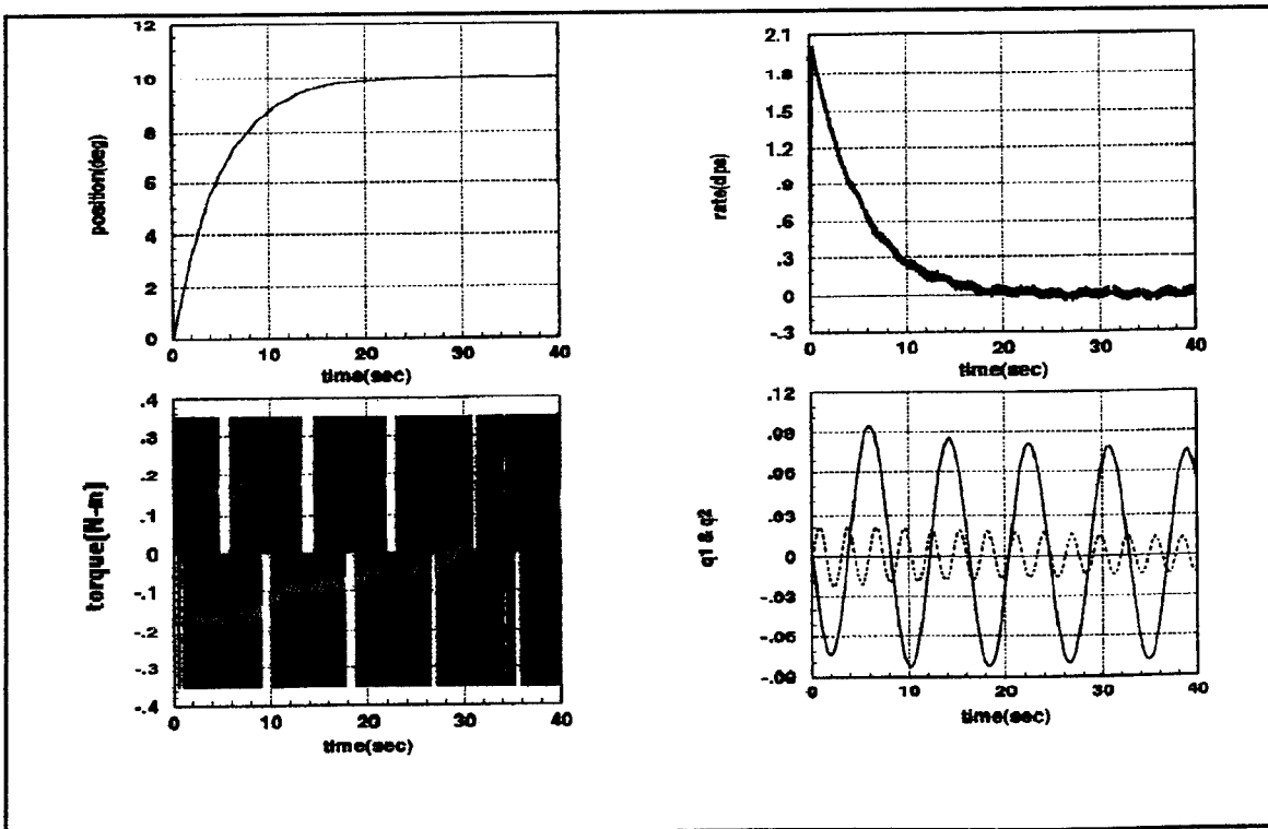
Figure 38. Simple Bang-Bang Step Response, Flexible Dynamics
