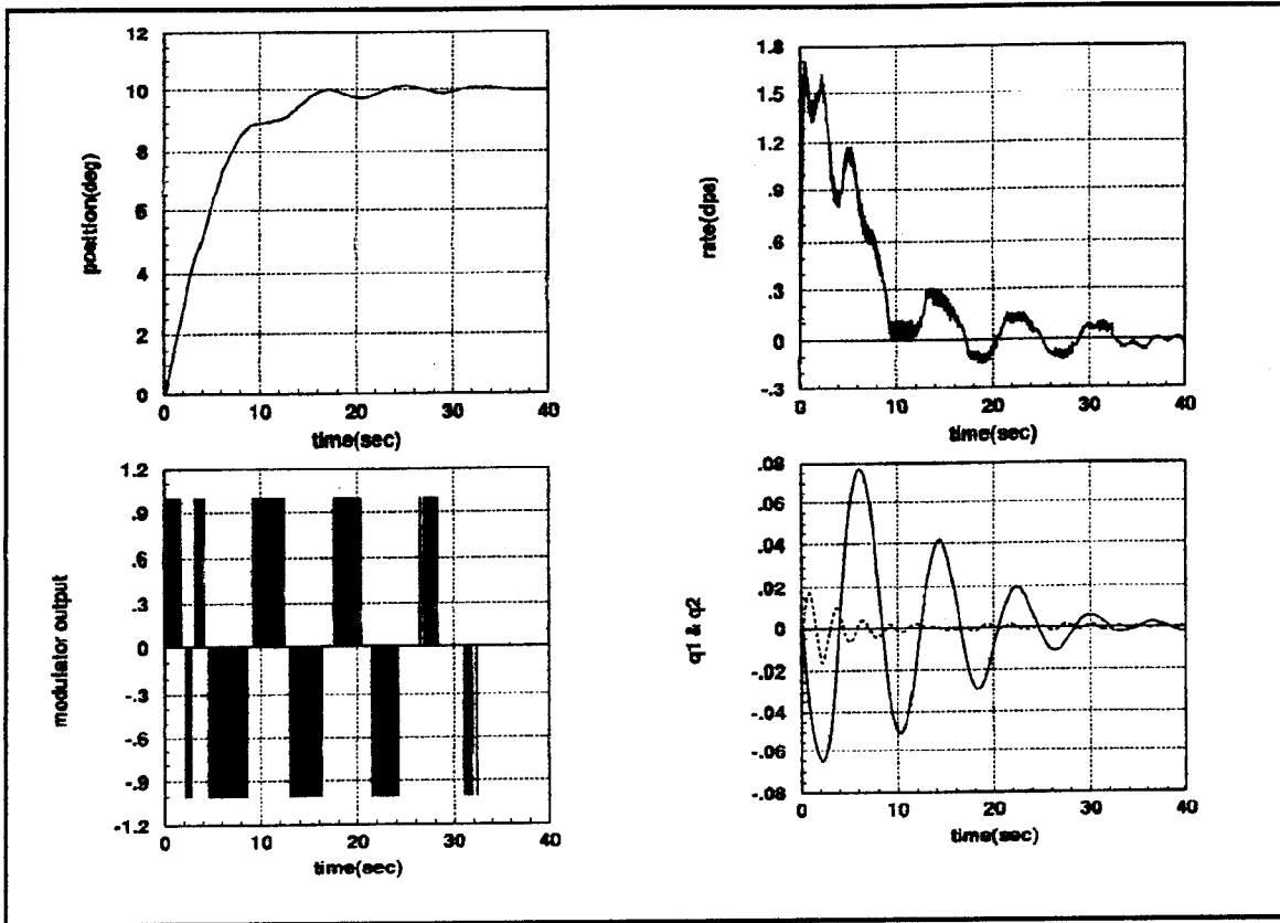
Figure 37. PWWF-Modulated Step Response, K=10 , Flexible Dynamics
