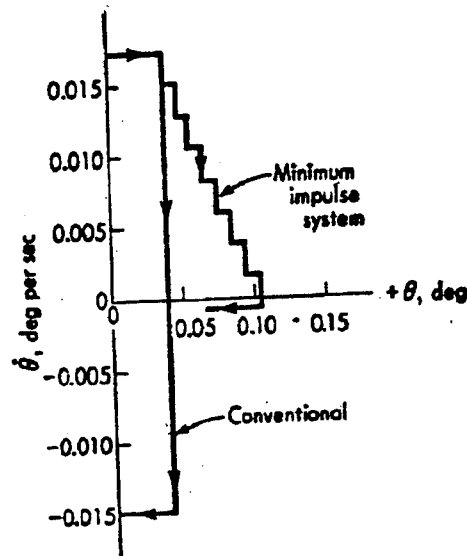
Figure 23. Expected Limit Cycles for Conventional (Bang-Bang) and Minimum Impulse (PWPF) Systems
