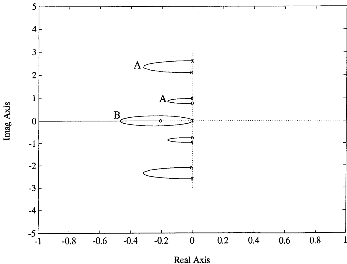
Figure 35. Root Locus vs. Forward Loop Gain With Position and Rate Feedback
