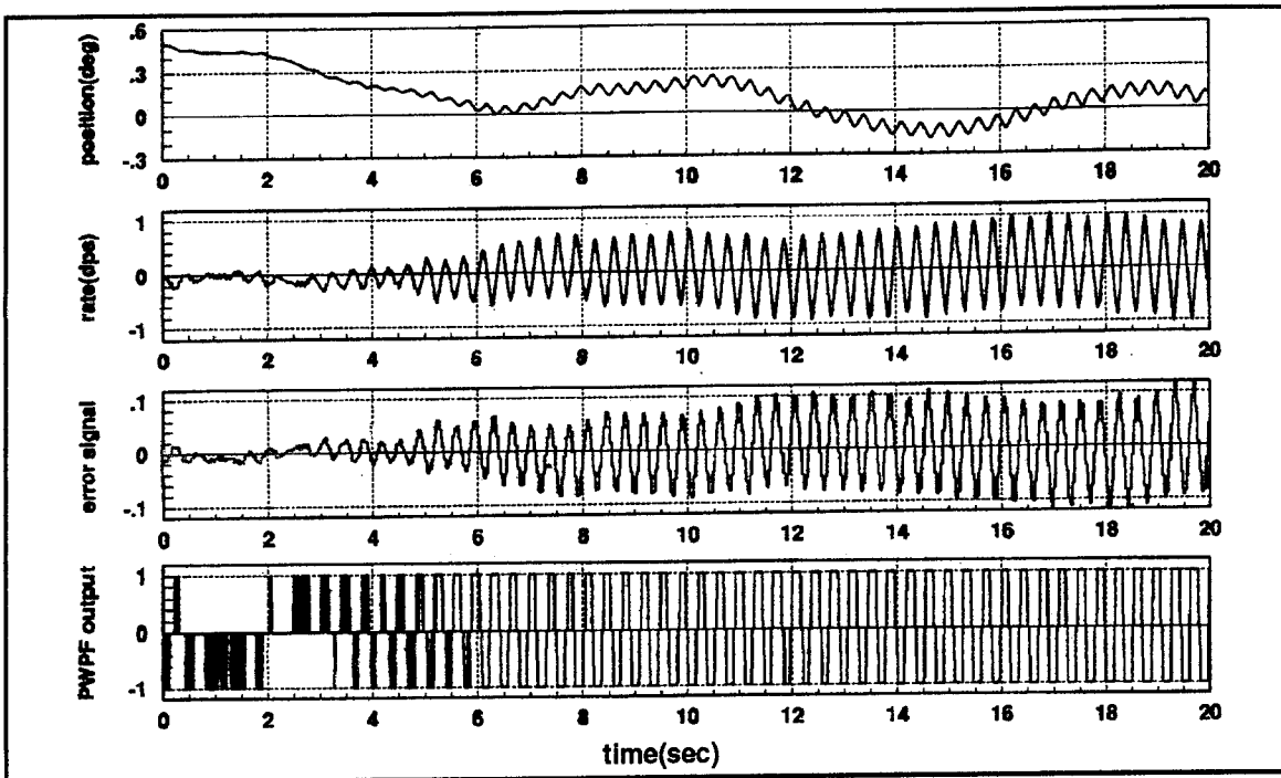
Figure 58. Initial Condition Response with K=30 , 60 msec Delay
