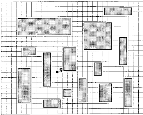
Figure 1: A city-block graph with distinguished start vertex s .
