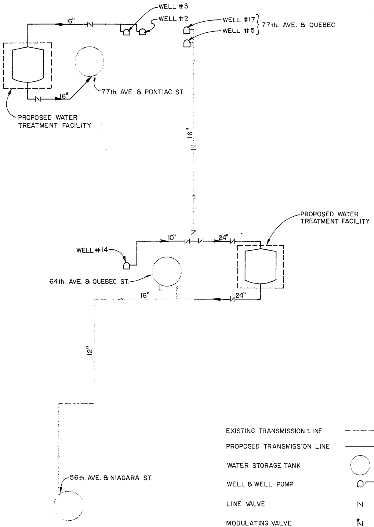
PIPELINE SCHEMATIC DECENTRALIZED PLANTS ALTERNATIVE
