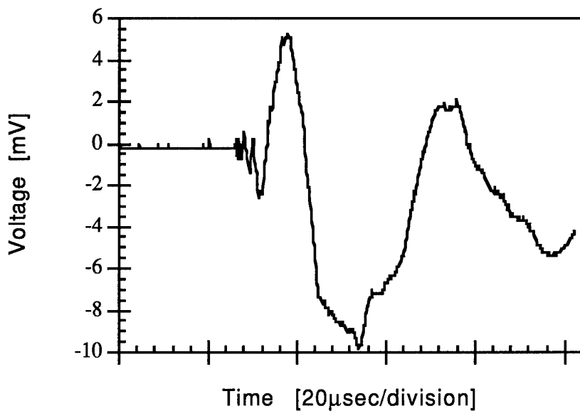
Fig. 5. Embedded sensor response to a lead break AE source. Trace taken by connecting the sensor directly to the 1M\Omega input of the DSO.
