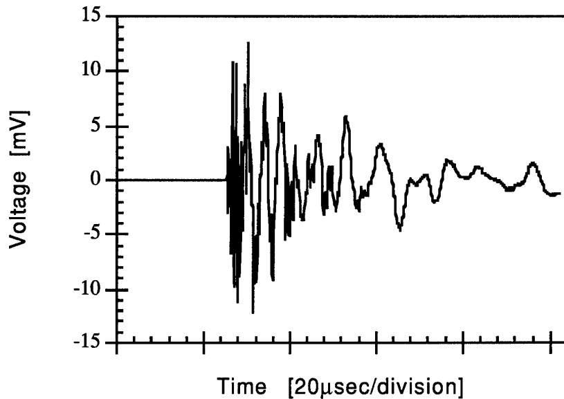
Fig. 4. Commercial sensor response to a lead break AE source. Trace taken by connecting the sensor directly to the 1M\Omega input of the DSO.
