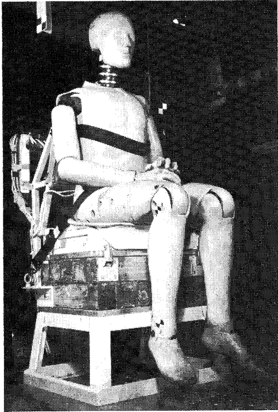
Figure 4. Hard Seat #1.
