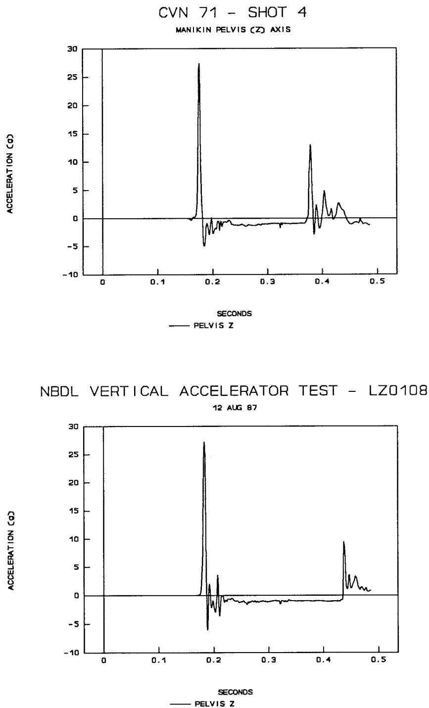
Figure 19. Pelvis Z-axis Response to Actual and Simulated Shock Pulses.
