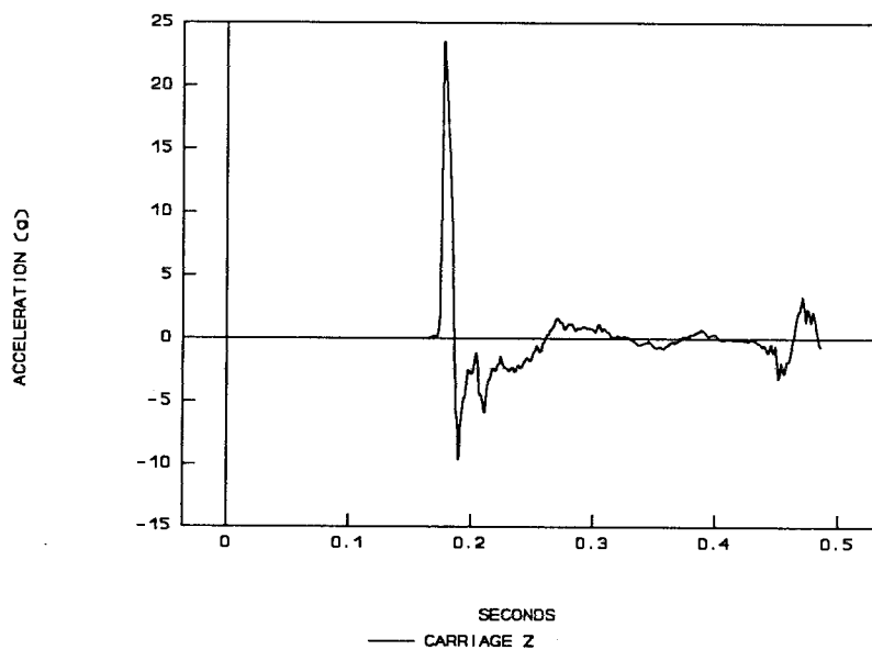
Figure 18. Comparison of Actual and Simulated Shock Pulses.
