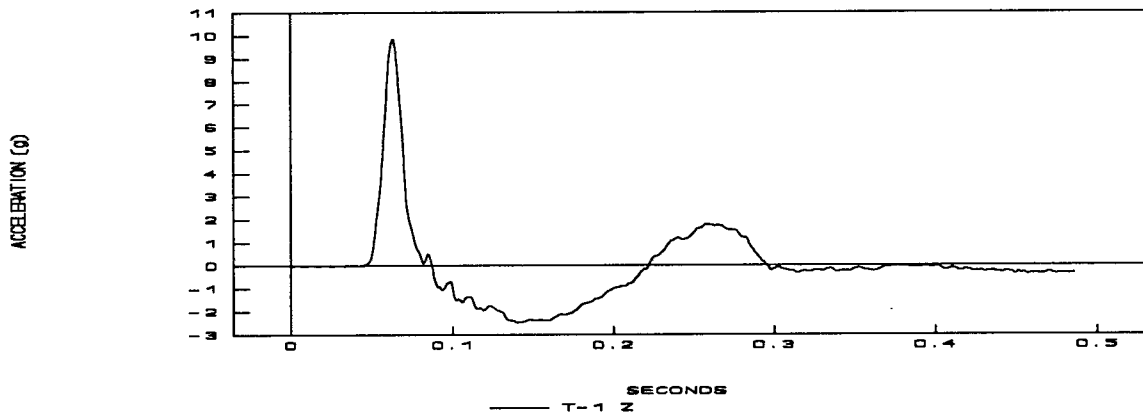
Figure 12. Shock Propagation through Pelvis and T-1 SPOC.
