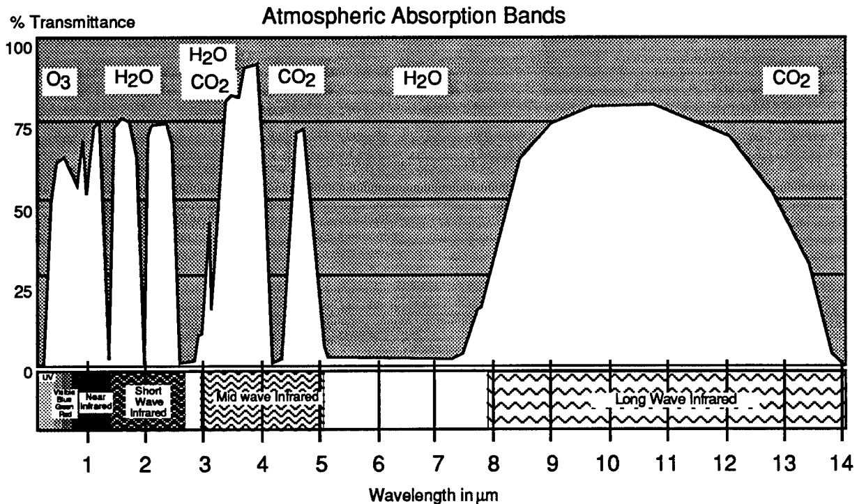
Figure 5. Atmospheric Absorption Bands & Transmission Windows 0 to 14 μm.
