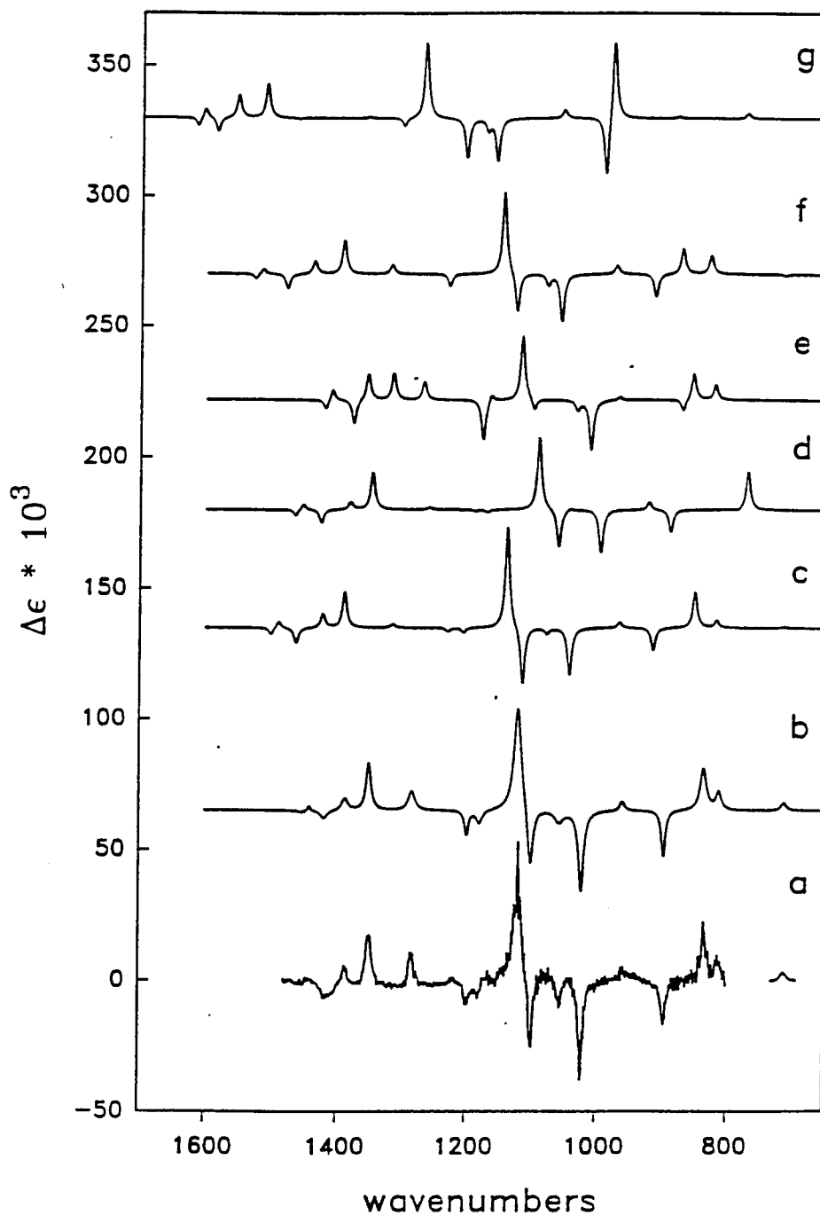
Figure 2. (a) Experimental VCD spectrum of R-1 (in \text{CCl}_4 and \text{CS}_2 solutions, from Devlin et al. [to be published]) ; (b) Fundamental VCD spectrum of R-1 (obtained from (a) by Lorentzian fitting [Devlin et al., to be published]) ; (c)–(g) Calculated VCD spectrum of R-1 (These originate as in Figure 1. All calculations use SCF TZ2P local AATs. Lorentzian band half-widths, \gamma , are 4.0 \text{ cm}^{-1} ).
