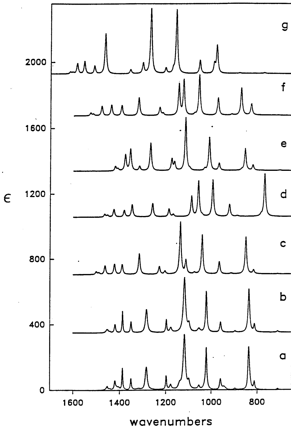
Figure 1. (a) Experimental unpolarized absorption spectrum of 1 (in \text{CCl}_4 and \text{CS}_2 solutions, from Devlin et al. [to be published]); (b) Fundamental unpolarized absorption spectrum of 1 (obtained from (a) by Lorentzian fitting [Devlin et al., to be published]); (c)–(g) Calculated unpolarized absorption spectrum of 1 (In (c), (d), and (e), force fields and APTs are calculated using DFT and B3LYP, BLYP, and LSDA density functionals, respectively. In (f) and (g), force fields and APTs are calculated using MP2 and SCF methodologies. All calculations use the TZ2P basis set. Lorentzian band half-widths, \gamma , are 4.0 \text{ cm}^{-1} ).
