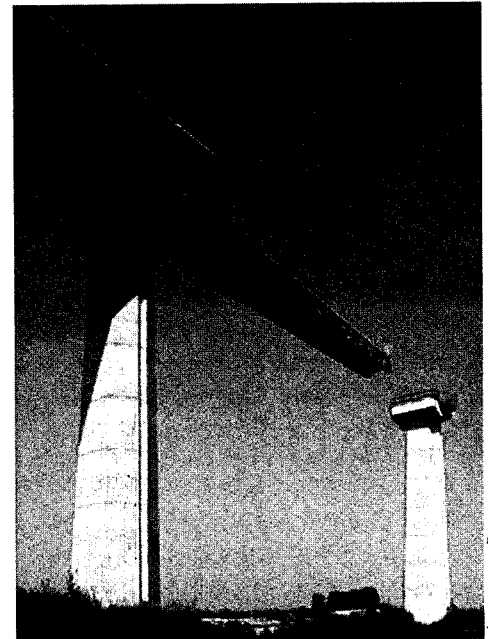
Construction of a bridge along the TGV North using a movable modular deck forming system.
