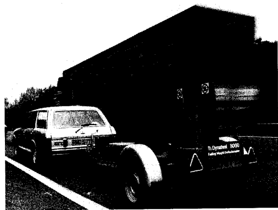
TRL's advanced condition survey equipment can perform all types of pavement assessment, from analysis of skid resistance to detailed investigations of structural problems in bituminous and concrete pavements.
