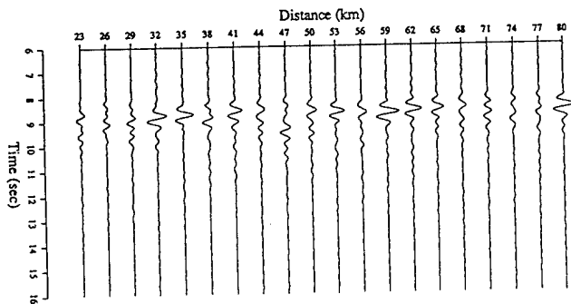
(b) Flicker-Noise Random Media ( \epsilon = 0.1, a = 5.0 \text{ km} )
