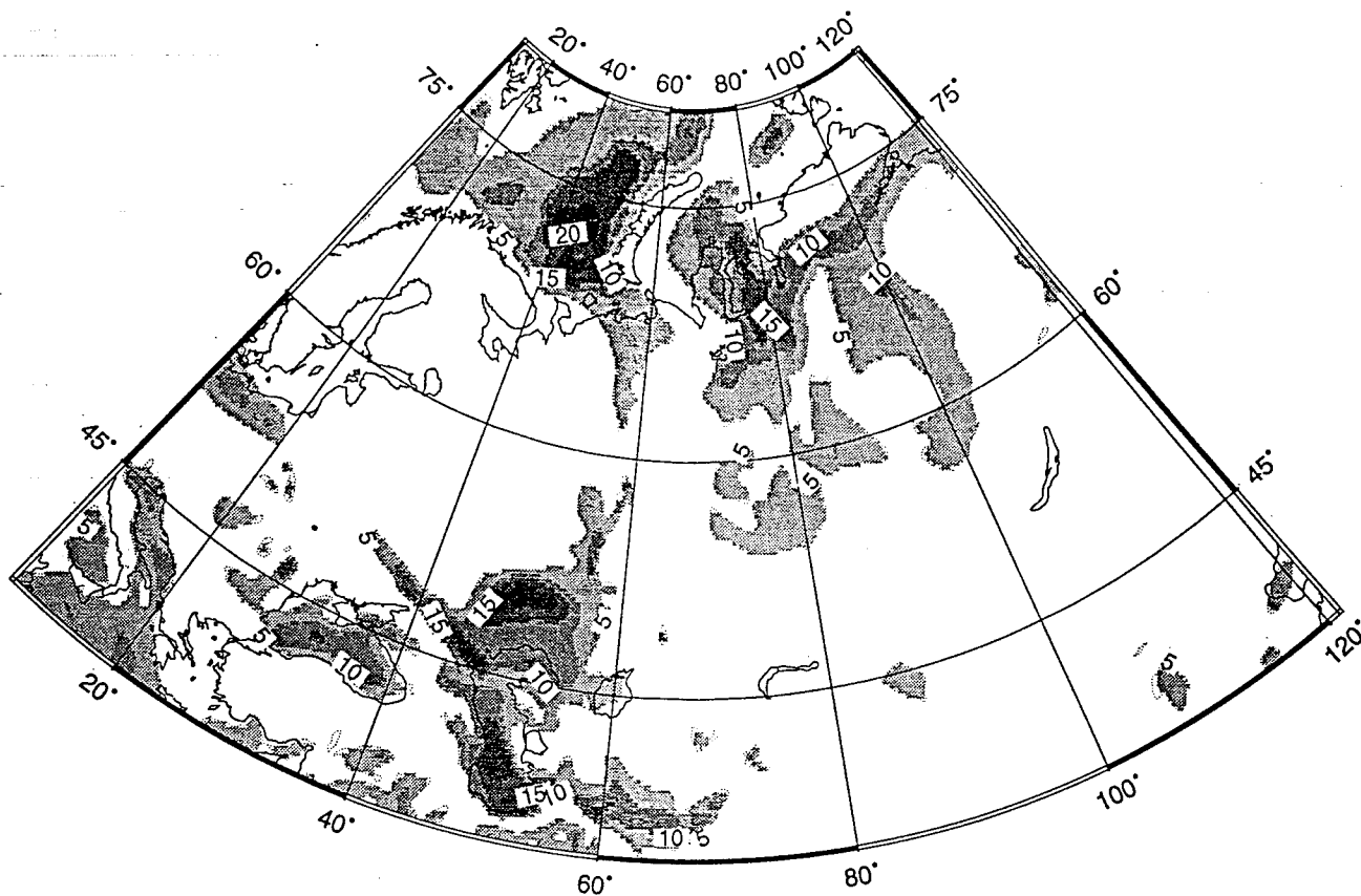
Figure 3. Map showing the sediment thickness, or basement depth variations of Eurasia. The data were digitized at Cornell from a Soviet map compiled by N. Kunin [Kunin, 1987; Fielding et al., 1992]. The sediment depth is indicated with 5-km contour intervals.
