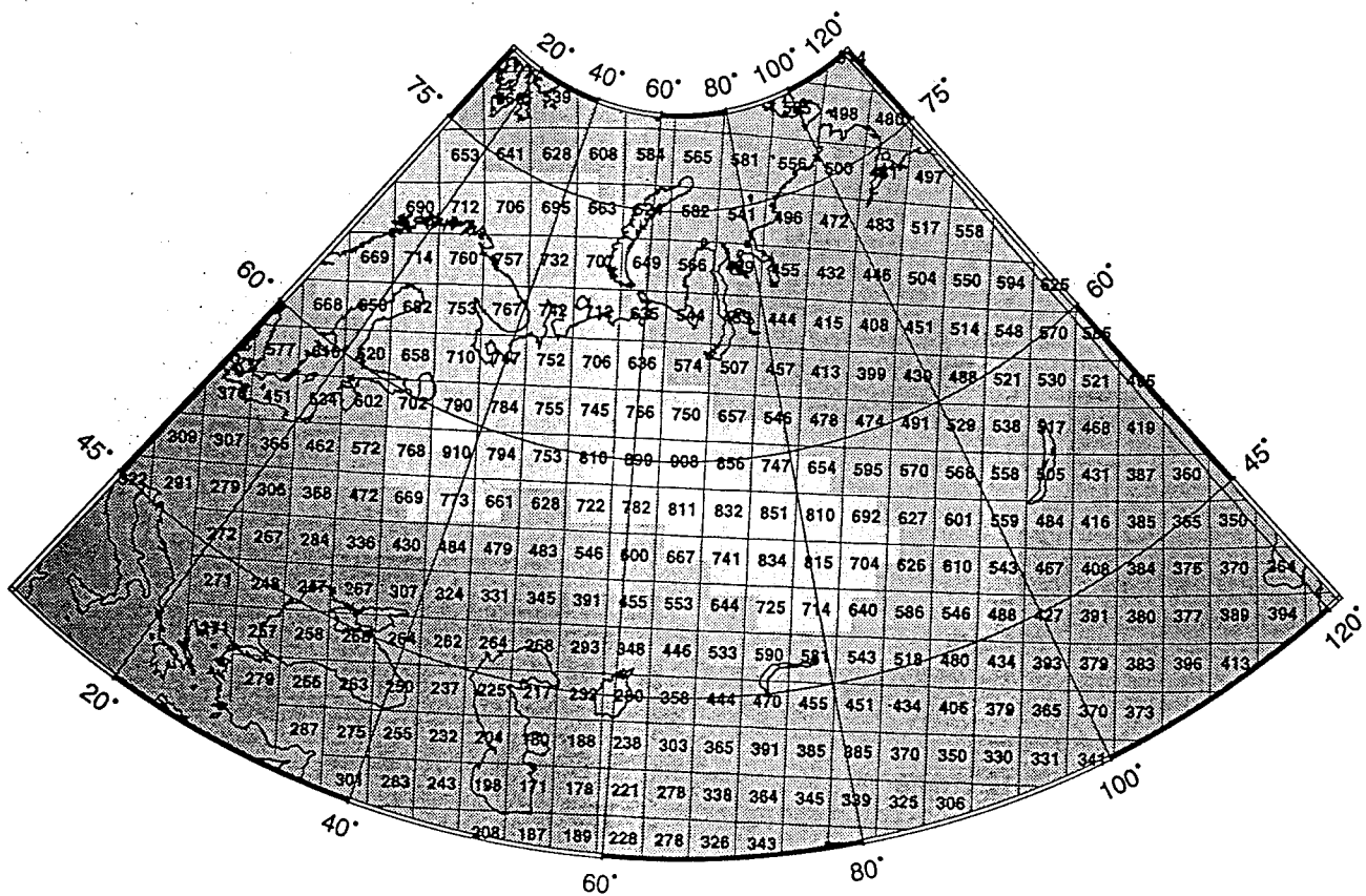
Figure 4. Map showing the L_p coda Q values of Eurasia at f = 1 Hz. These tomographic results are from Pan et al. [1992].
