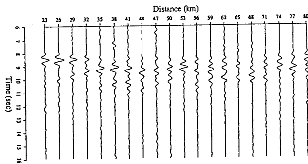
(a) Multi-Uniform-Cylinder Model ( \epsilon = -0.3, a = 5.0 \text{ km} )
