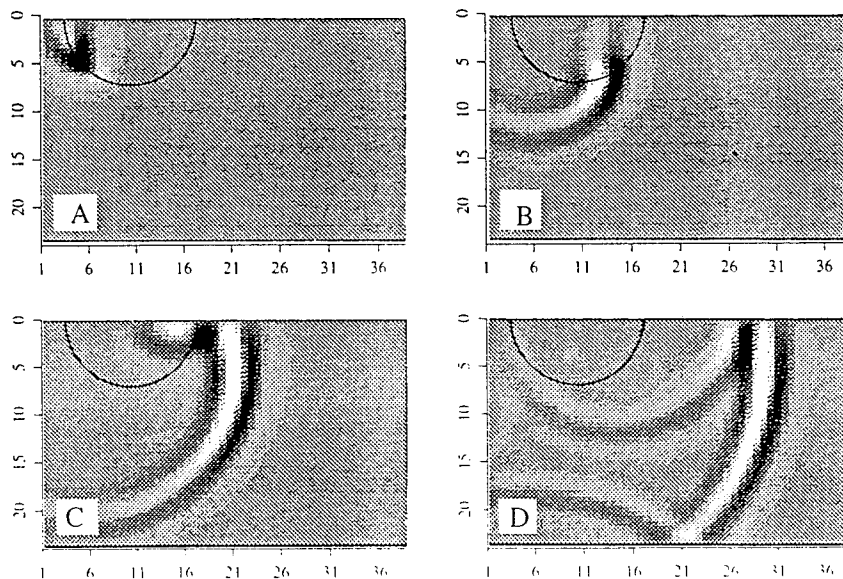
Fig. 4b. Some corresponding snapshots from FD: A, t = 1 s; B, t = 3 s; C, t = 5 s; D, t = 7 s. From comparison of Figure 4a and 4b it can be seen that except for the lack of backscattered waves in the ECS method, the forward wavefronts are quite similar for these two methods.
