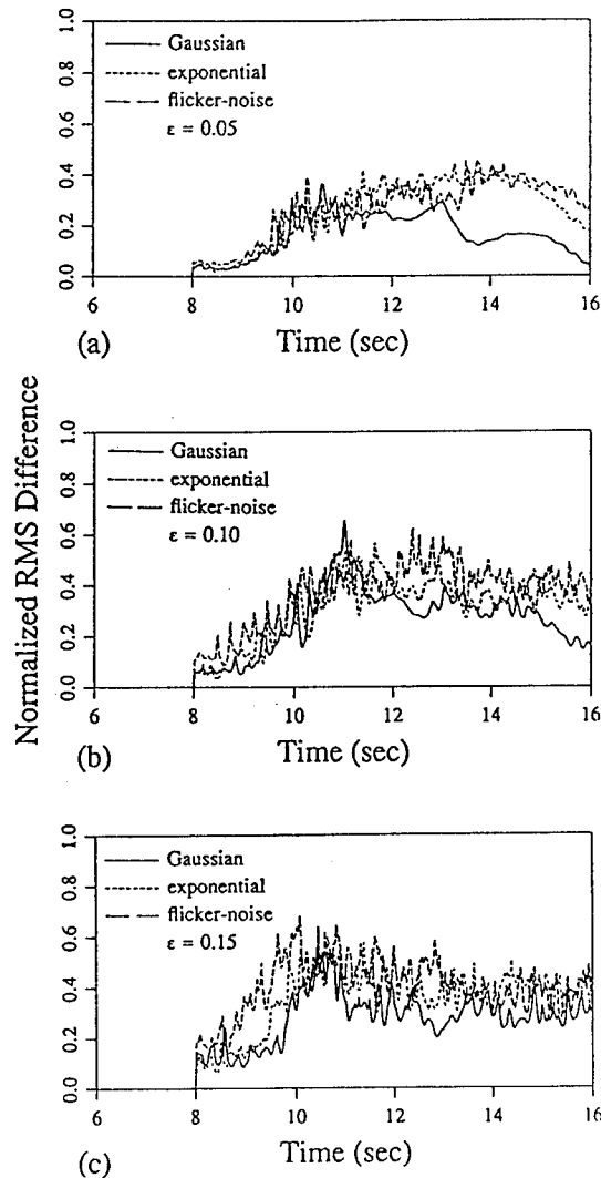
Figure 9. Root mean square differences of the phase screen and finite difference seismograms for the nine models. The rms differences are normalized by the maximum amplitude at the corresponding time for each curve.
