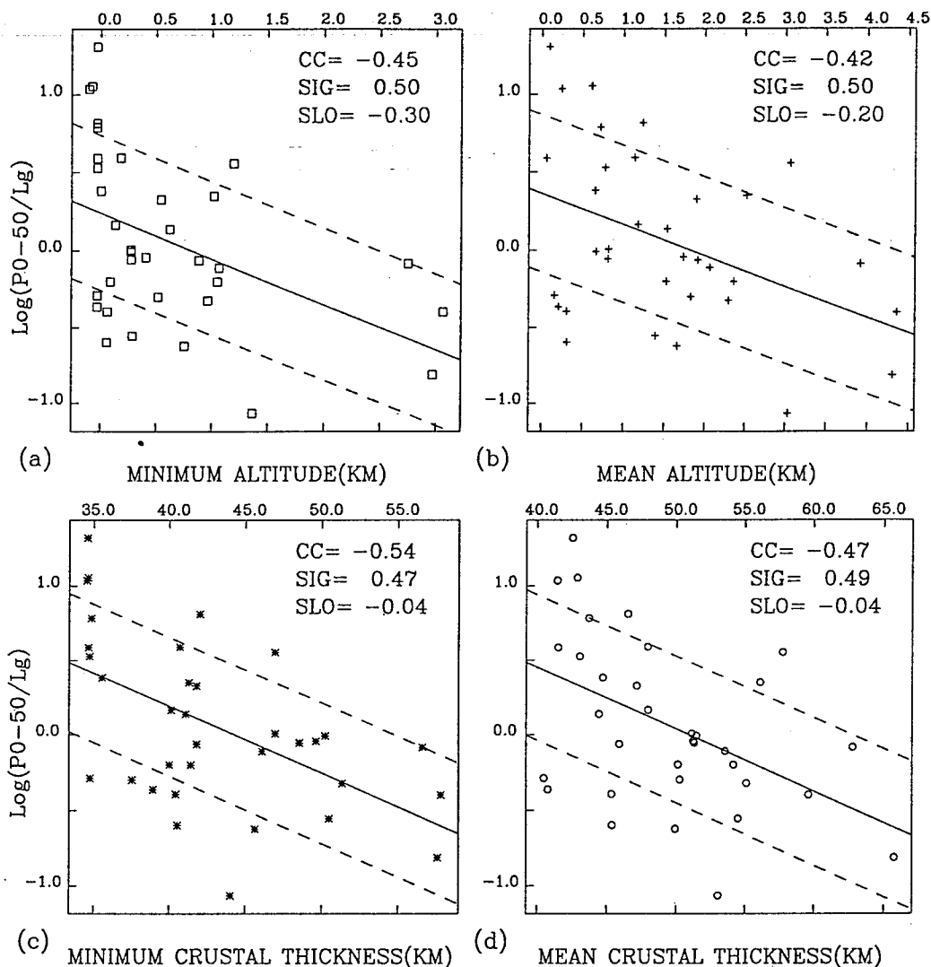
Figure 6. The log P/L_g ratio variations with (a) minimum and (b) mean altitude, and (c) minimum and (d) mean crustal thickness for earthquake data. CC stands for correlation coefficient, SIG is standard deviation of linear correlation, SLO is the slope of the linear regression. "P0-50" refers to RMS amplitude in 50-s window beginning with P onset.
