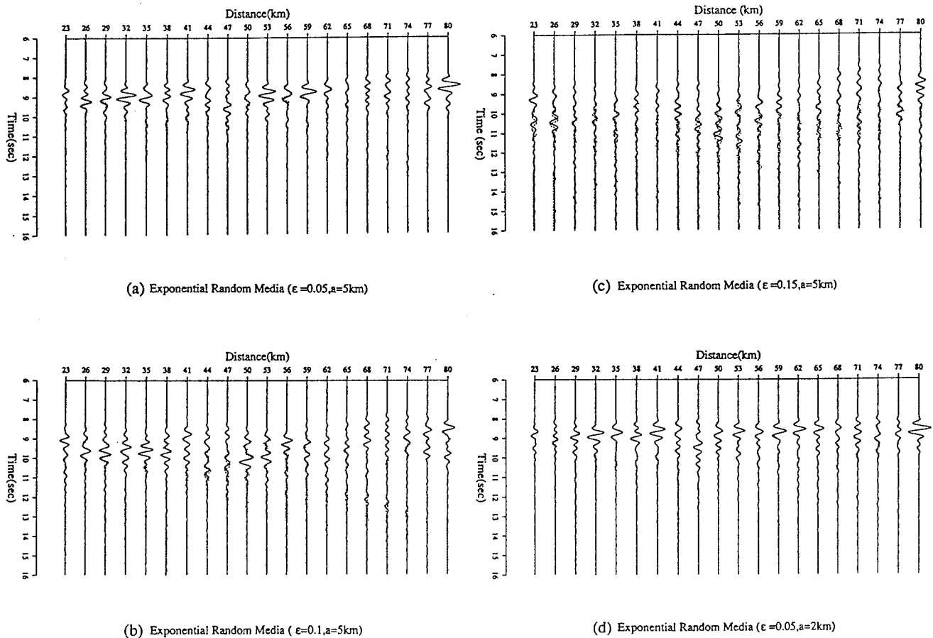
Figure 7. Comparison of synthetic seismograms for (a) model 4a, (b) model 4b, (c) model 4c, and (d) model 4d (see Table 1). Solid and dotted curves stand for the phase screen and finite difference solutions, respectively.
