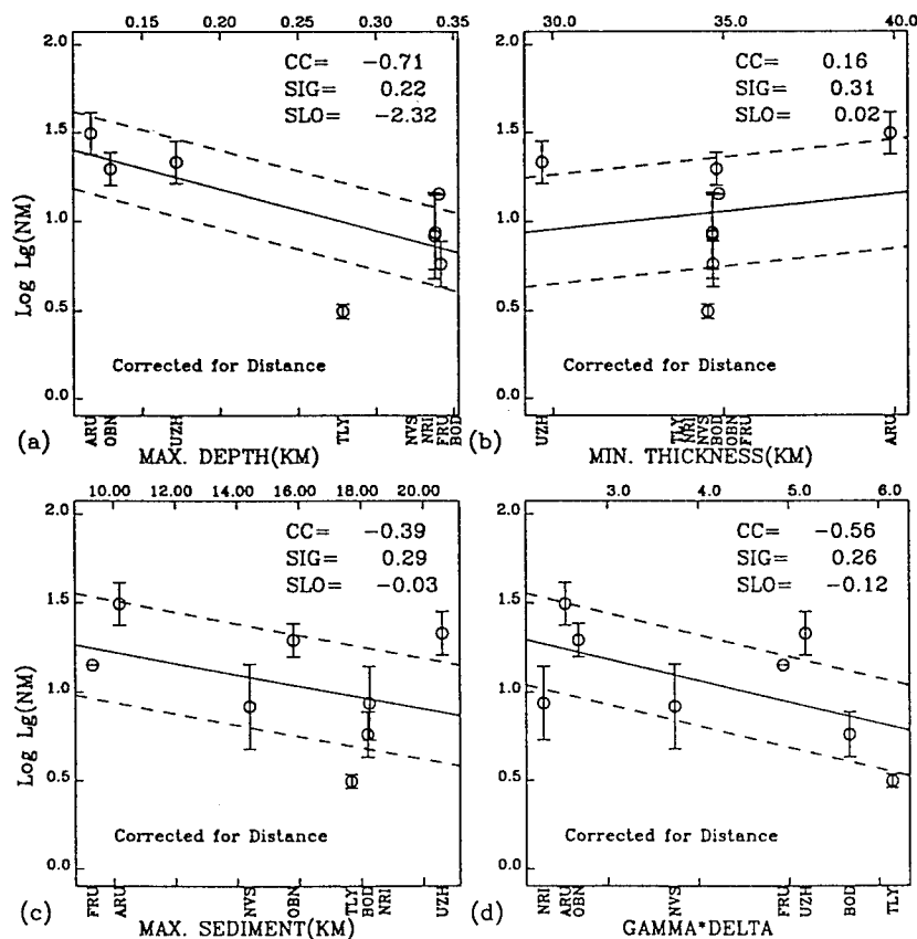
Figure 17. The relationships between L_g amplitudes, corrected for geometric spreading, and (a) maximum water depth, (b) minimum crustal thickness, (c) maximum sedimentary layer thickness, and (d) the attenuation term \gamma\Delta along each path.
