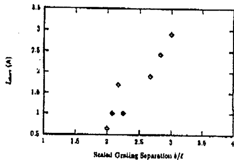
Fig. 13. Start oscillation current versus grating spacing: Configuration A.
