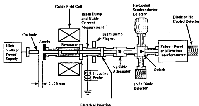
FIG. 1. A schematic view of the experimental apparatus is shown in block form.
