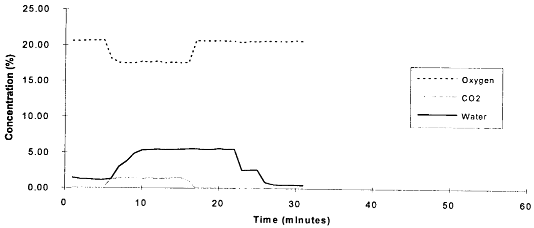
Halon 1301 - Test 2
