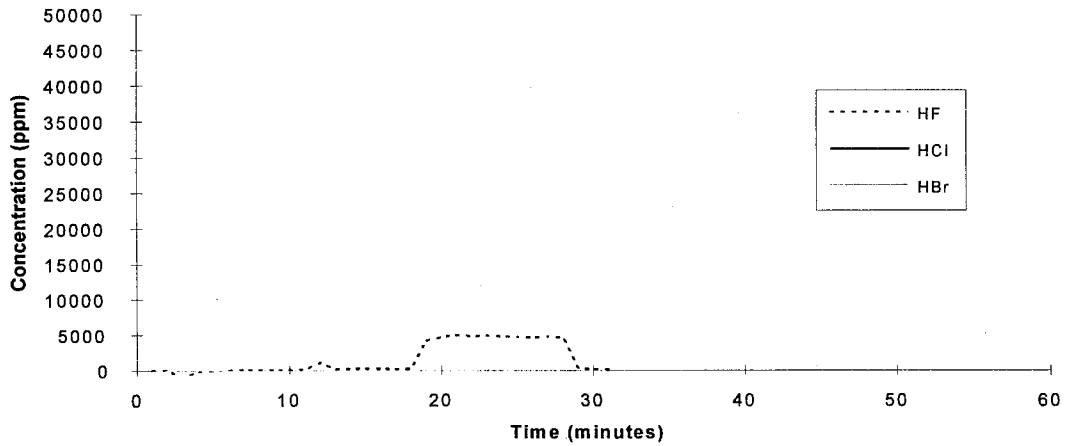
CF3I - Test 3
