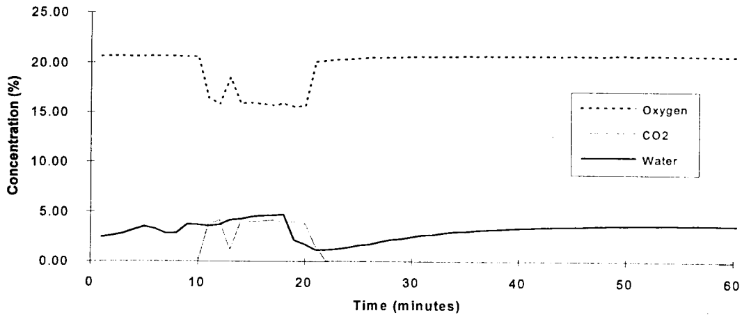
Perfluoropentane - Test 3
