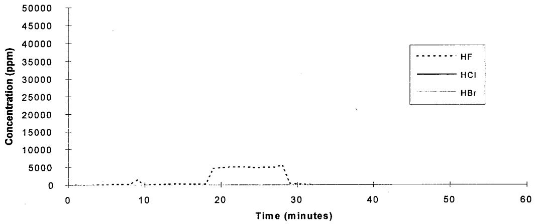
CF3I - Test 2
