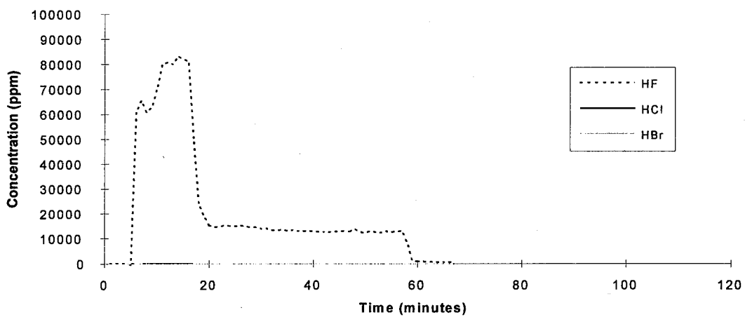
HFC 23 - Test 2
