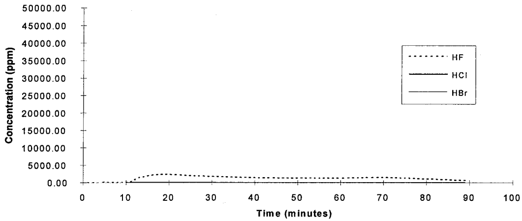
C3F7I - Test 2
