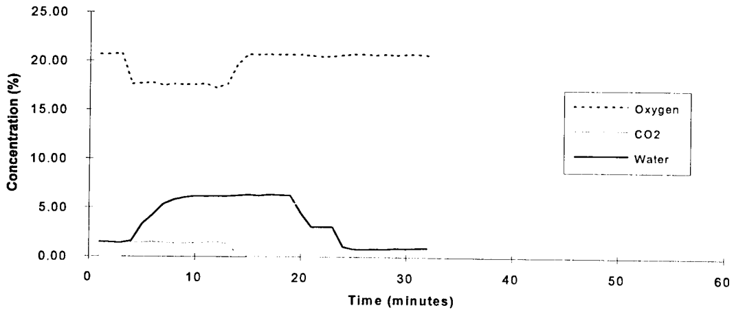
Halon 1301 - Test 3
