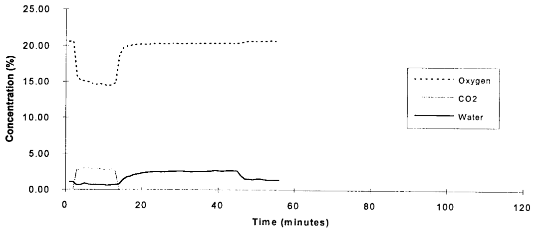
HFC 23 - Test 1
