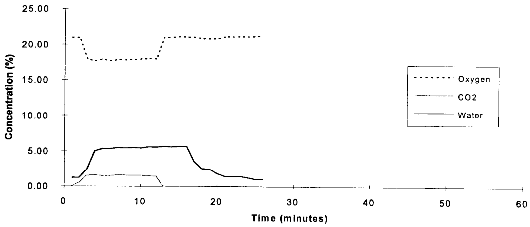
HBFC-22B1 - Test 2
