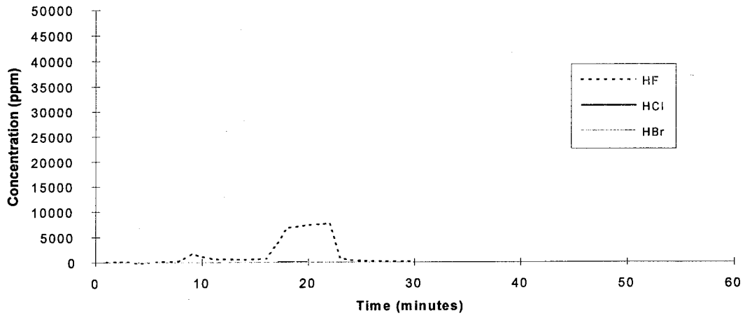
CF3I - Test 1
