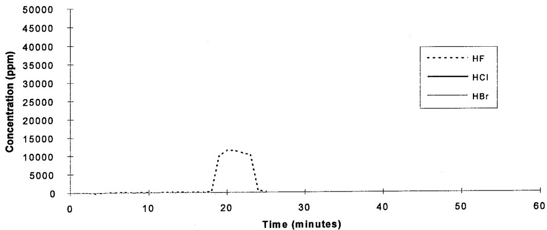
HBFC-22B1 - Test 1
