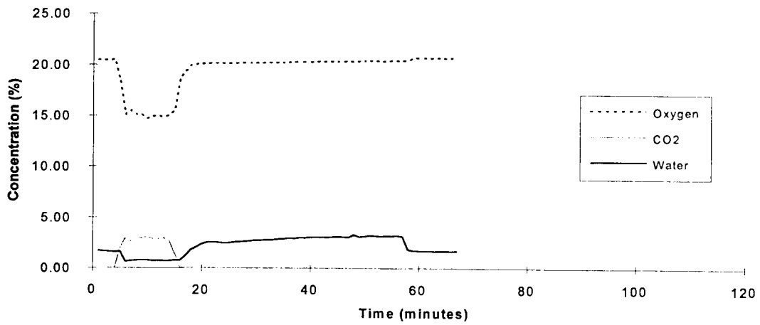
HFC 23 - Test 2
