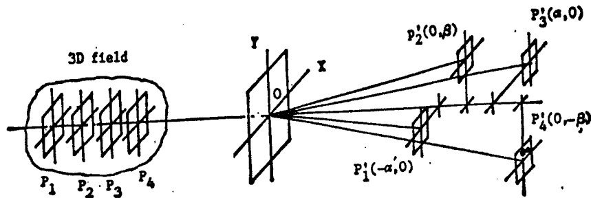
P_1, P_2, P_3, P_4 —Sampled planes in 3D field, P'_1, P'_2, P'_3, P'_4 —Conjugate planes of P_1, P_2, P_3, P_4
