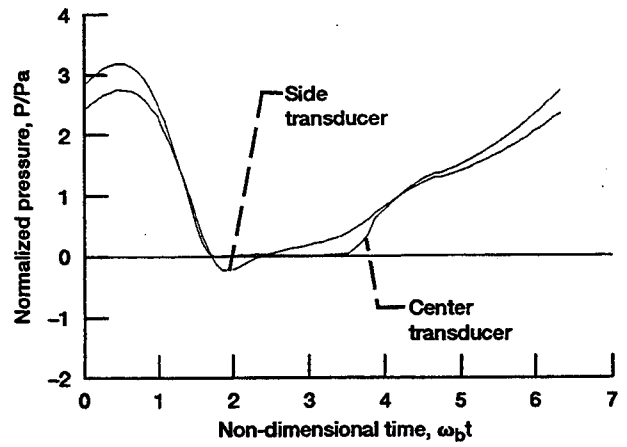
(b) Pressure variation.
