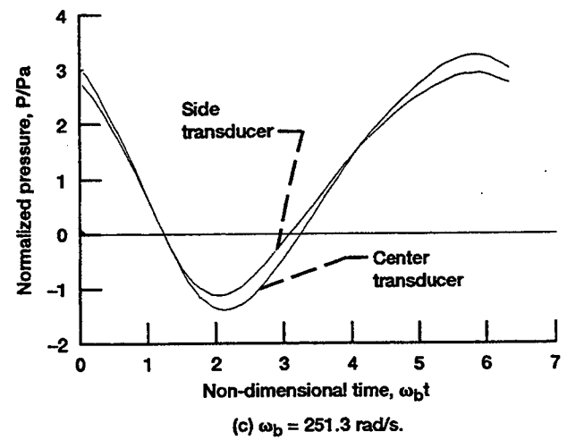
Figure 13.—Pressure variations at \theta = 337.5 deg.
